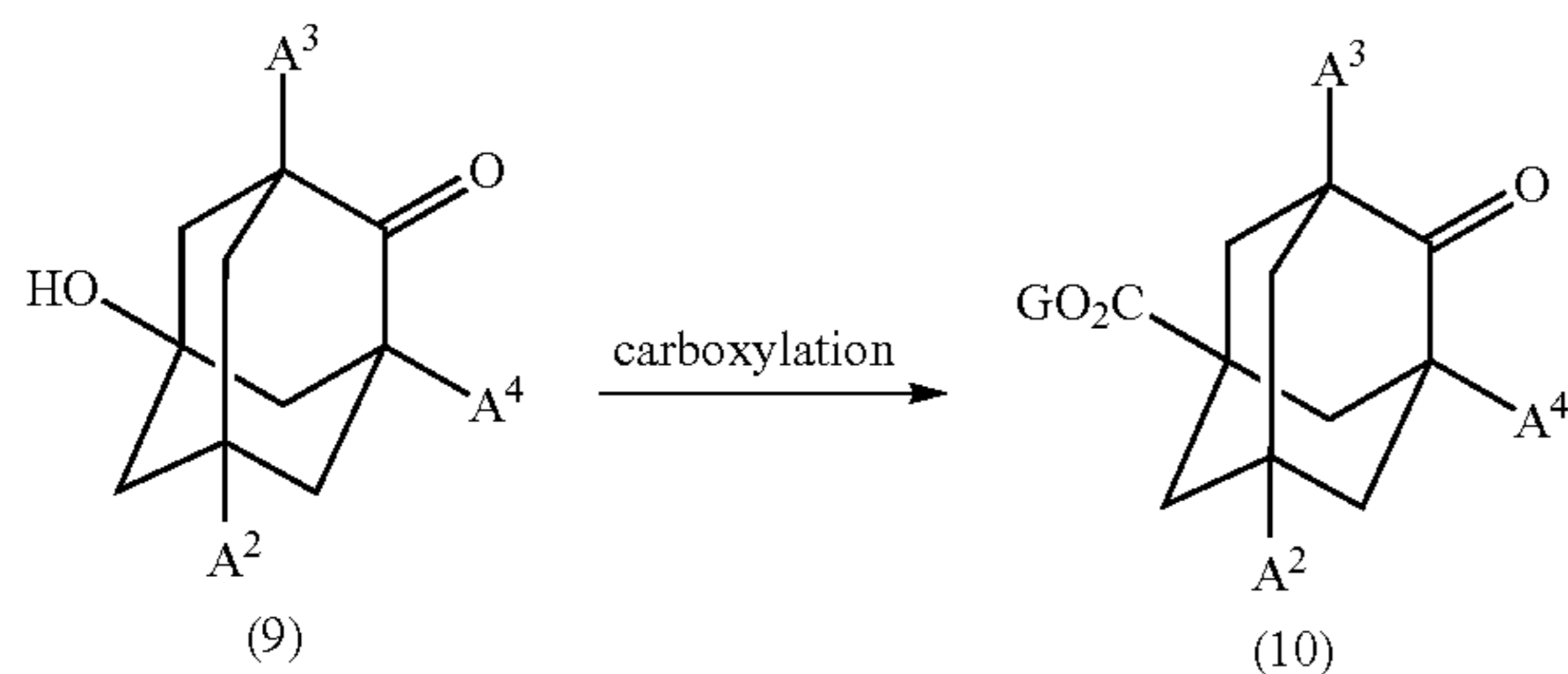
Scheme 3
