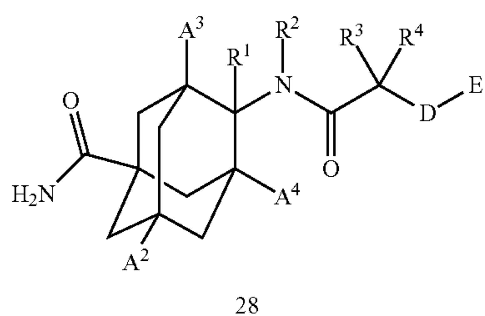
Scheme 8
