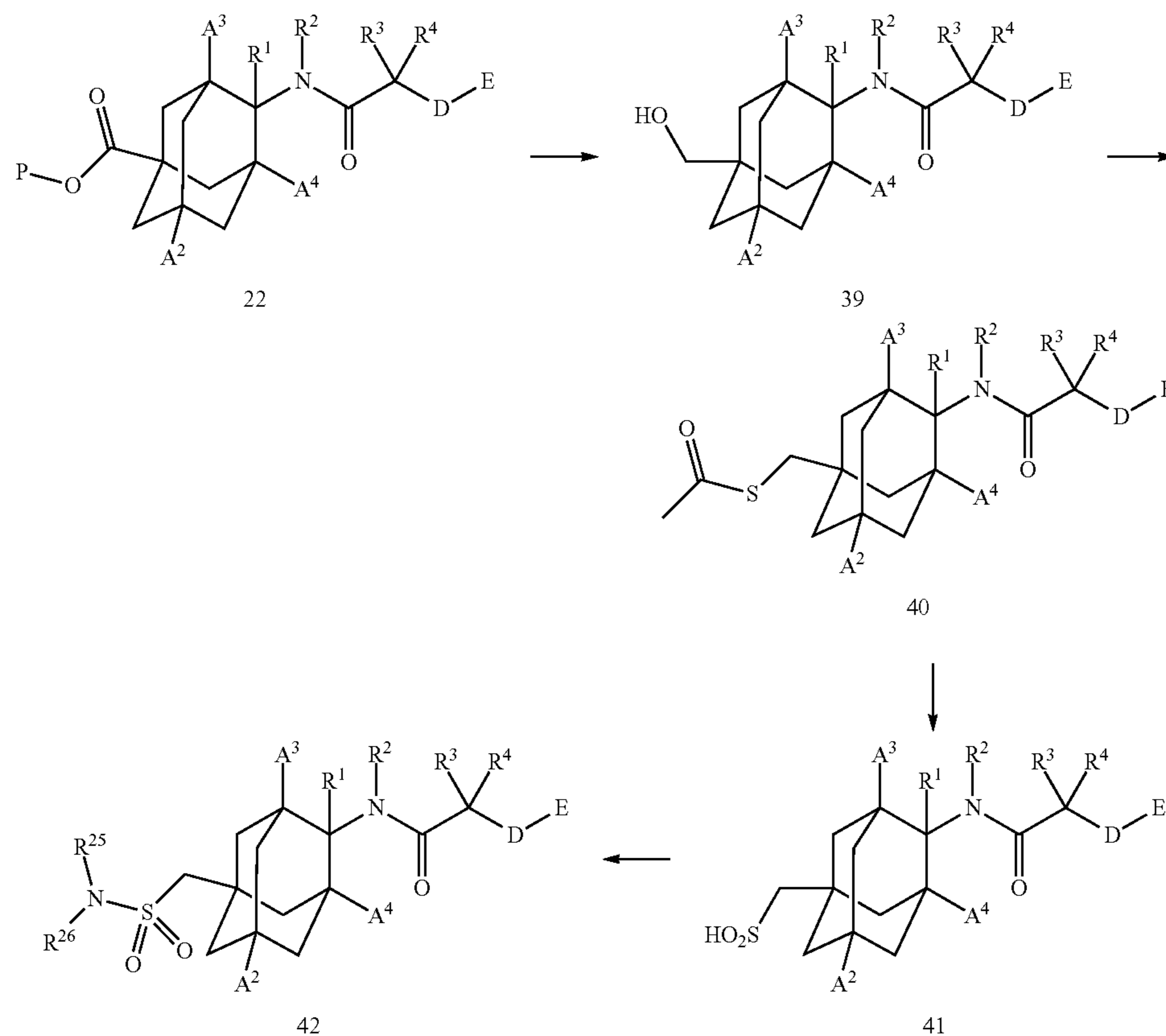
Scheme 11
