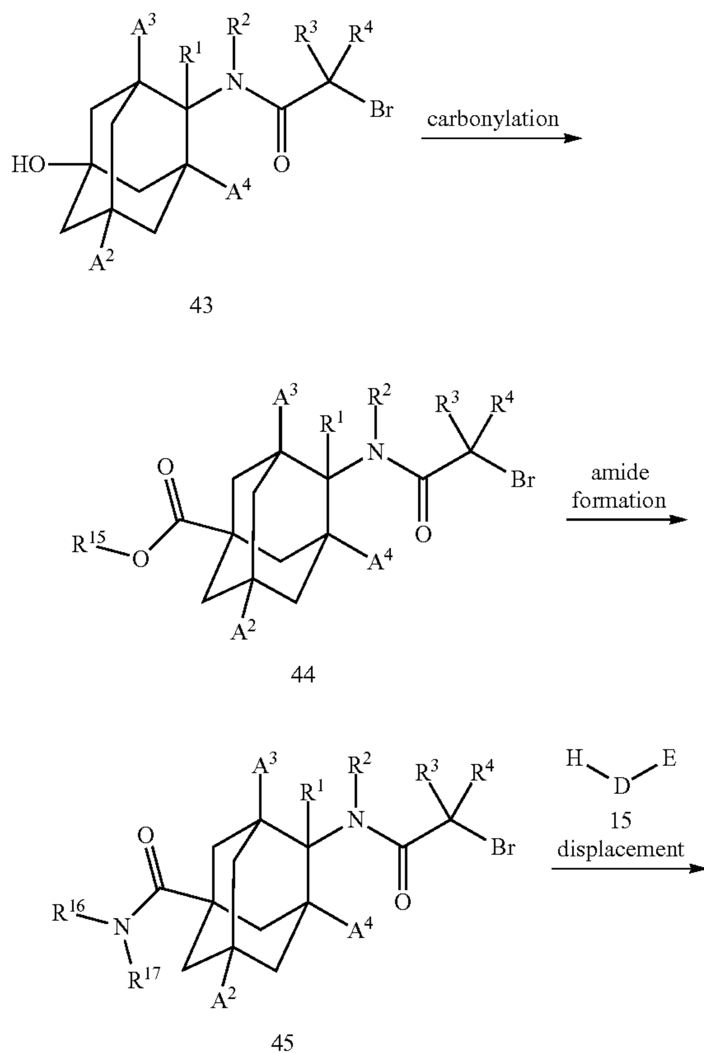
Scheme 12
