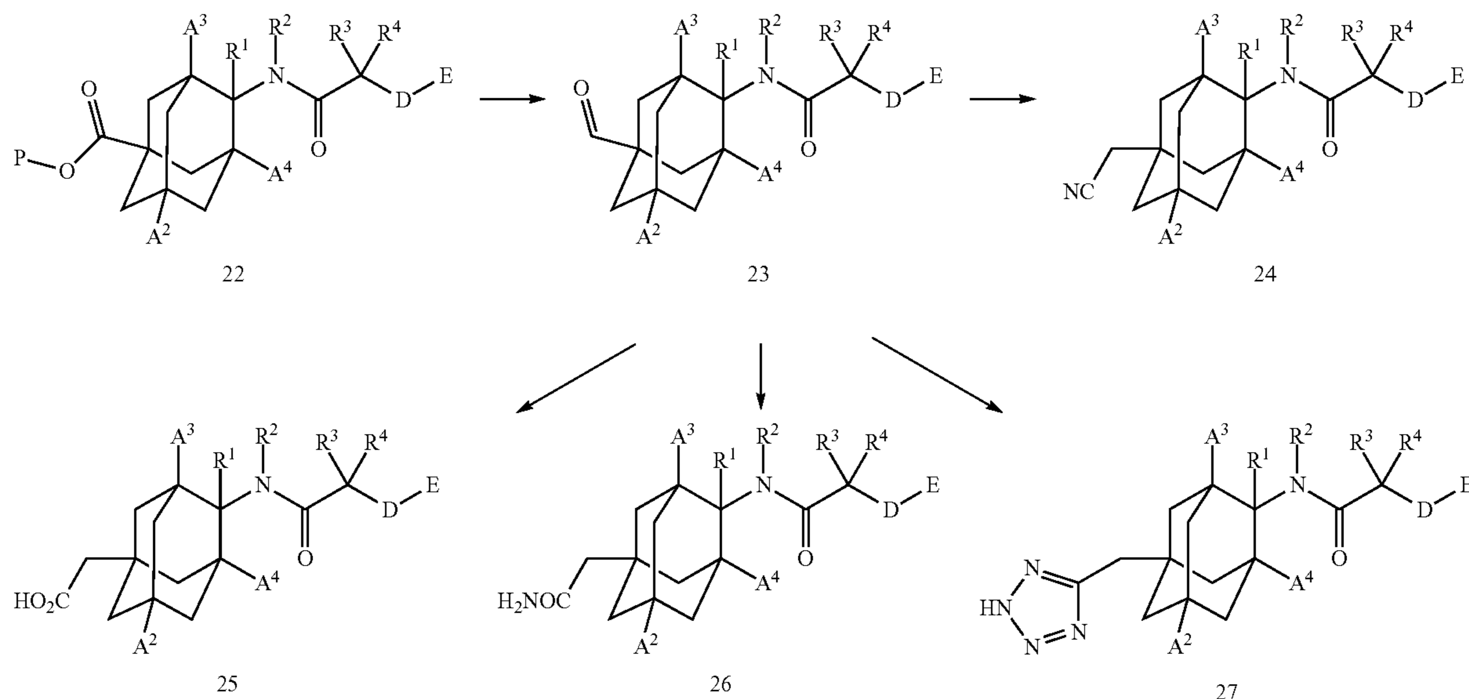
Scheme 7
