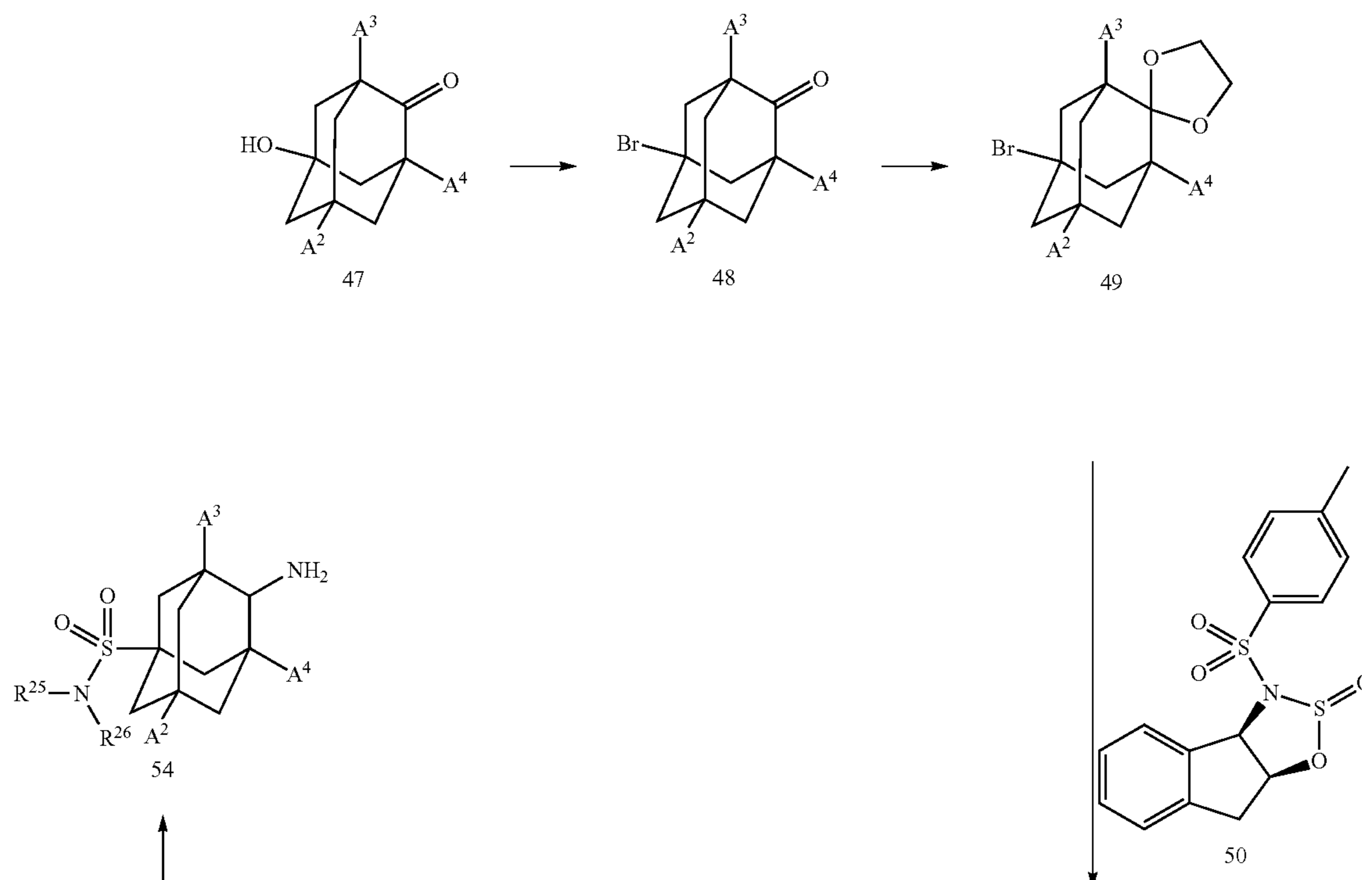
Scheme 13
