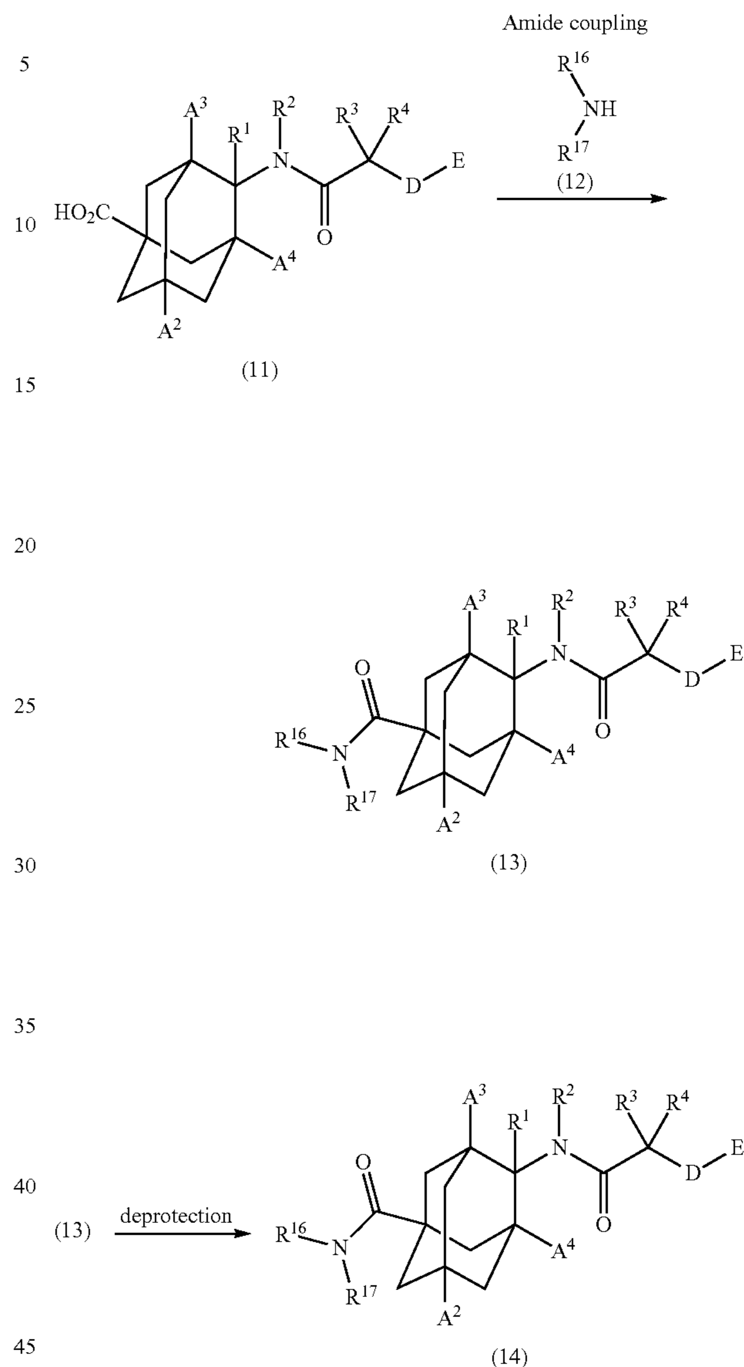
Scheme 4
