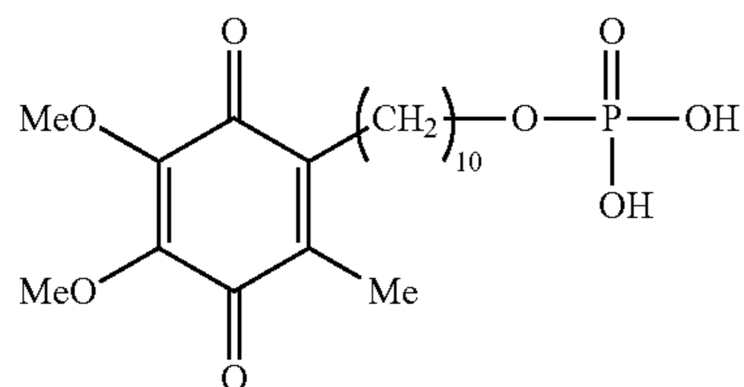
(idebenone phosphate ester)
