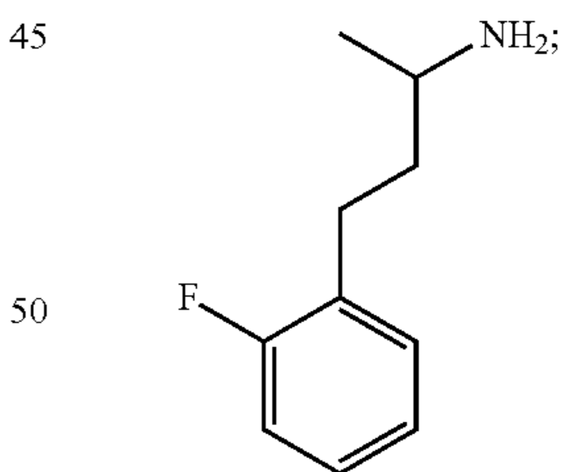
4-(2-bromophenyl)butan-2-amine
