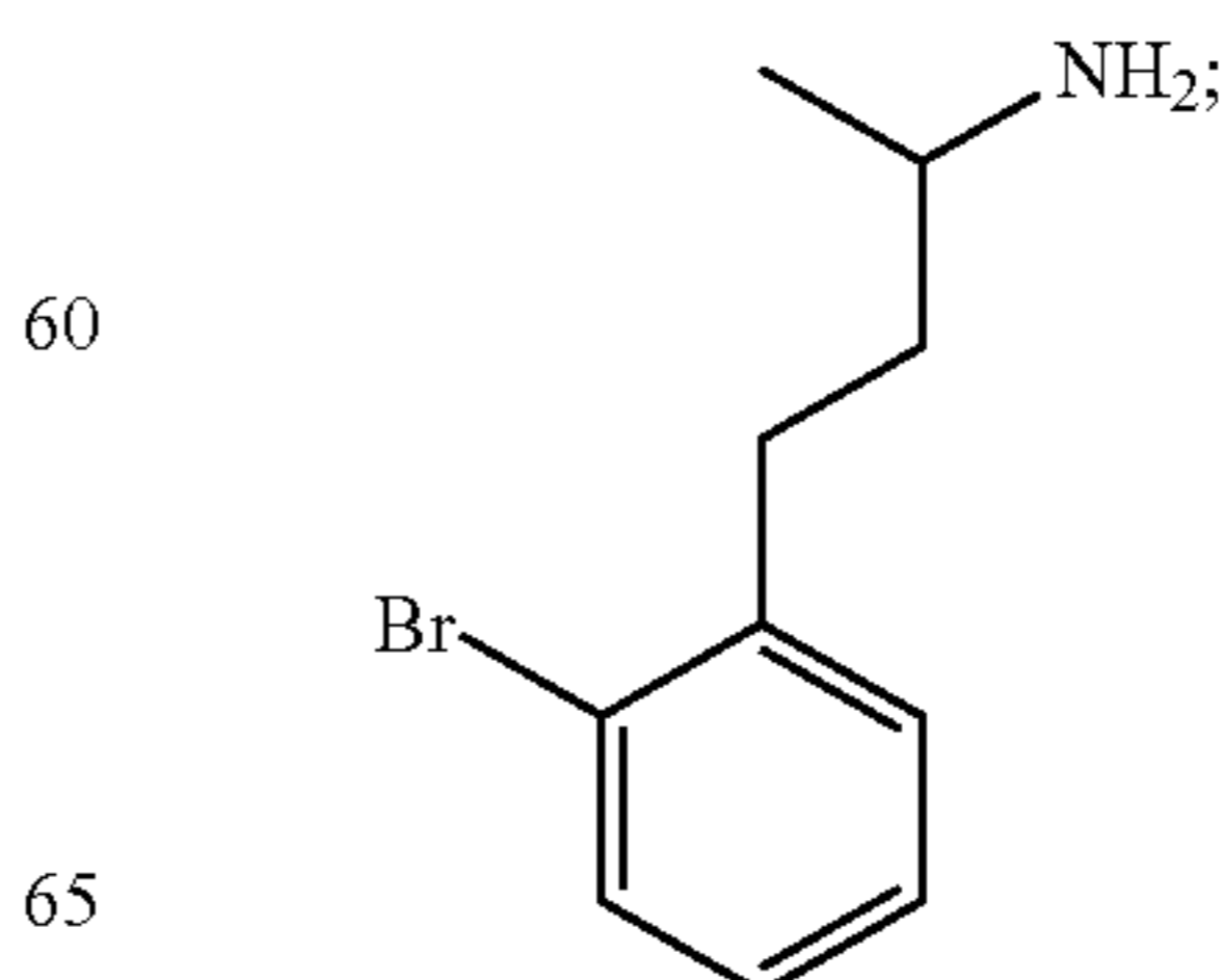
4-(2-bromophenyl)butan-2-amine
