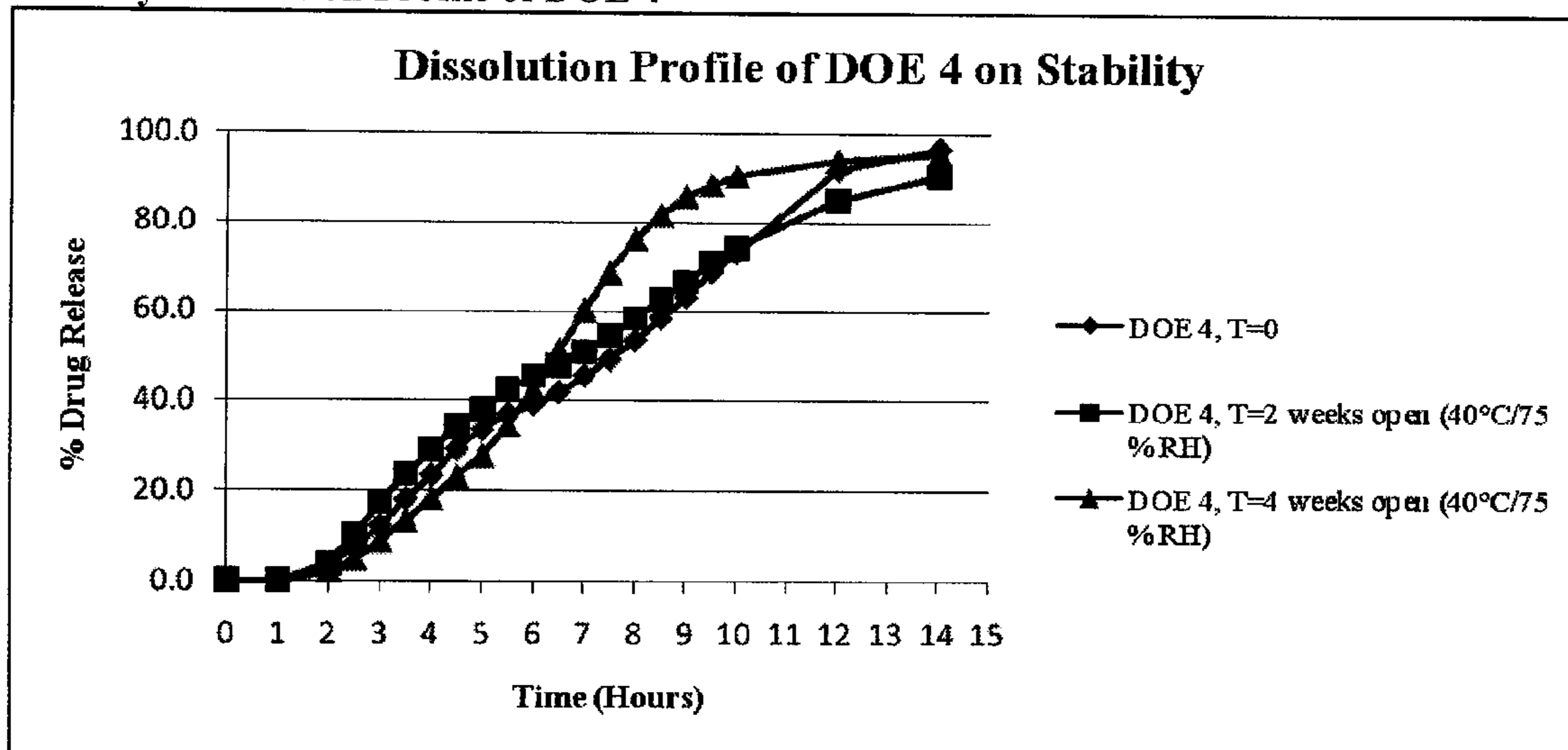
Stability Dissolution Profile of DOE 4
