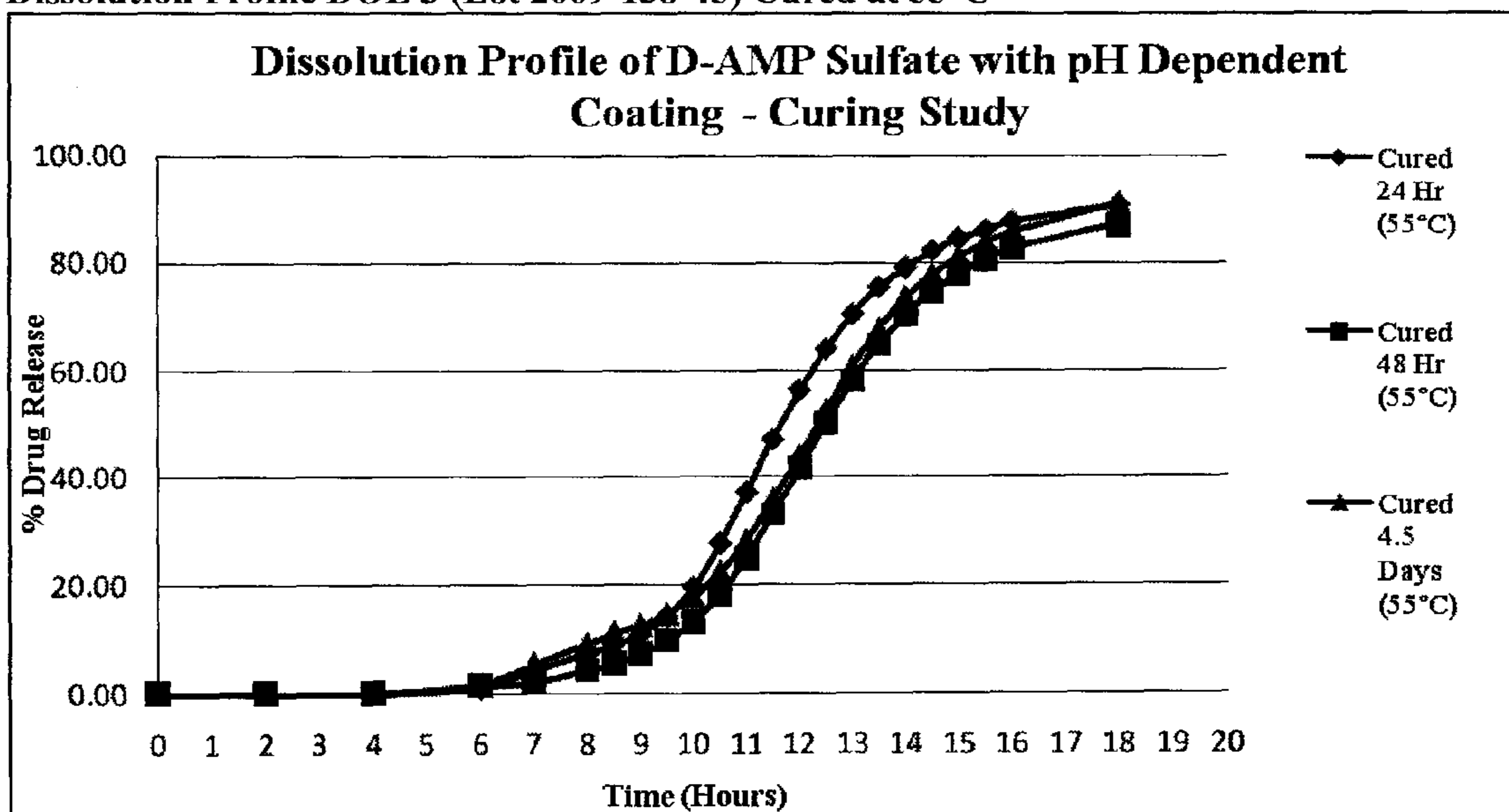
Dissolution Profile DOE 3 (Lot 2009-138-45) Cured at 55°C
