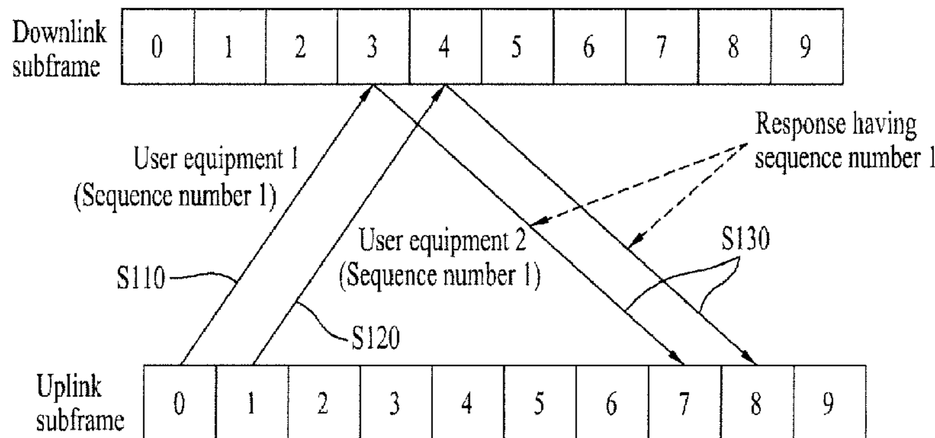
< Example of random access response >
