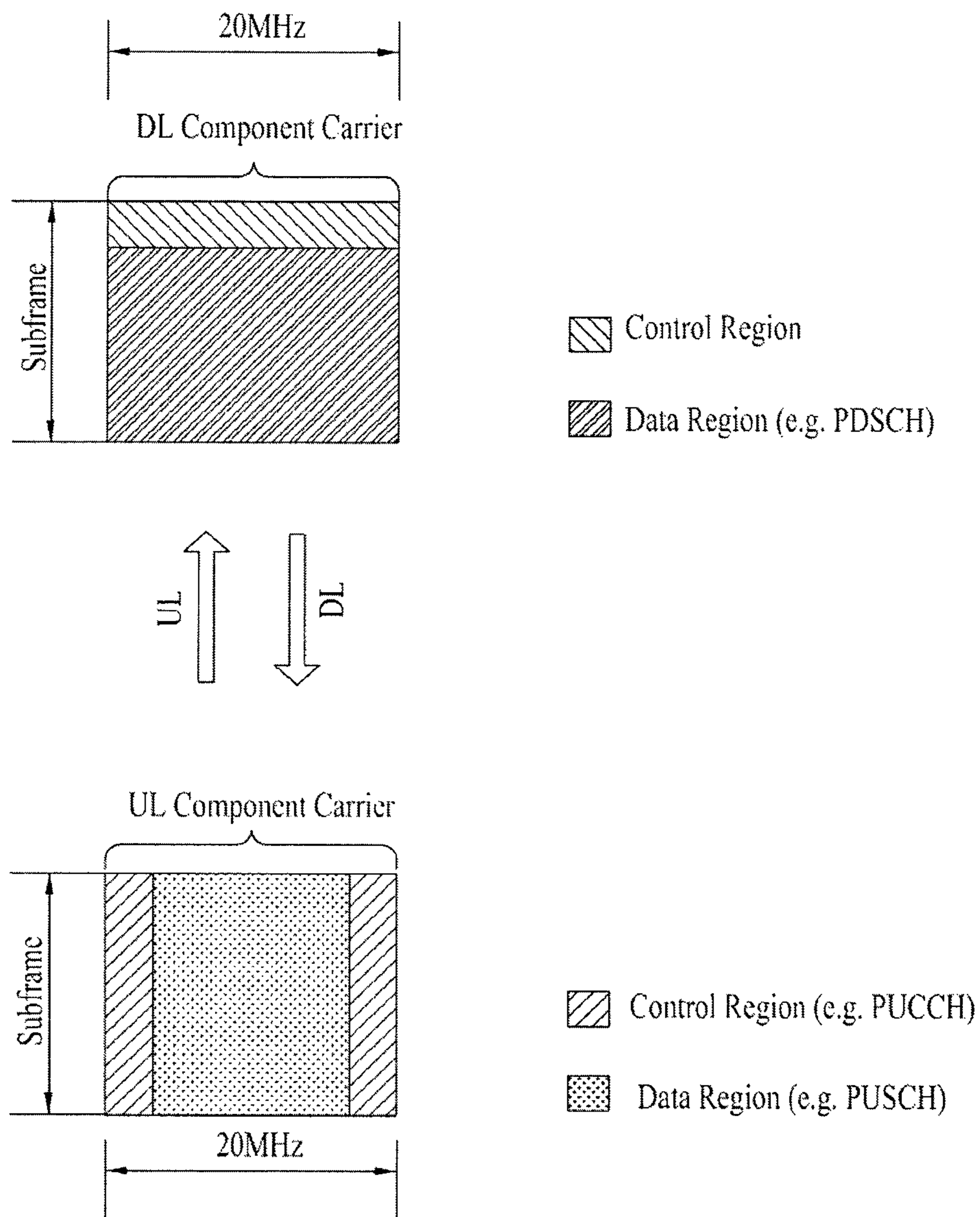
Single Component Carrier (e.g. LTE System)
