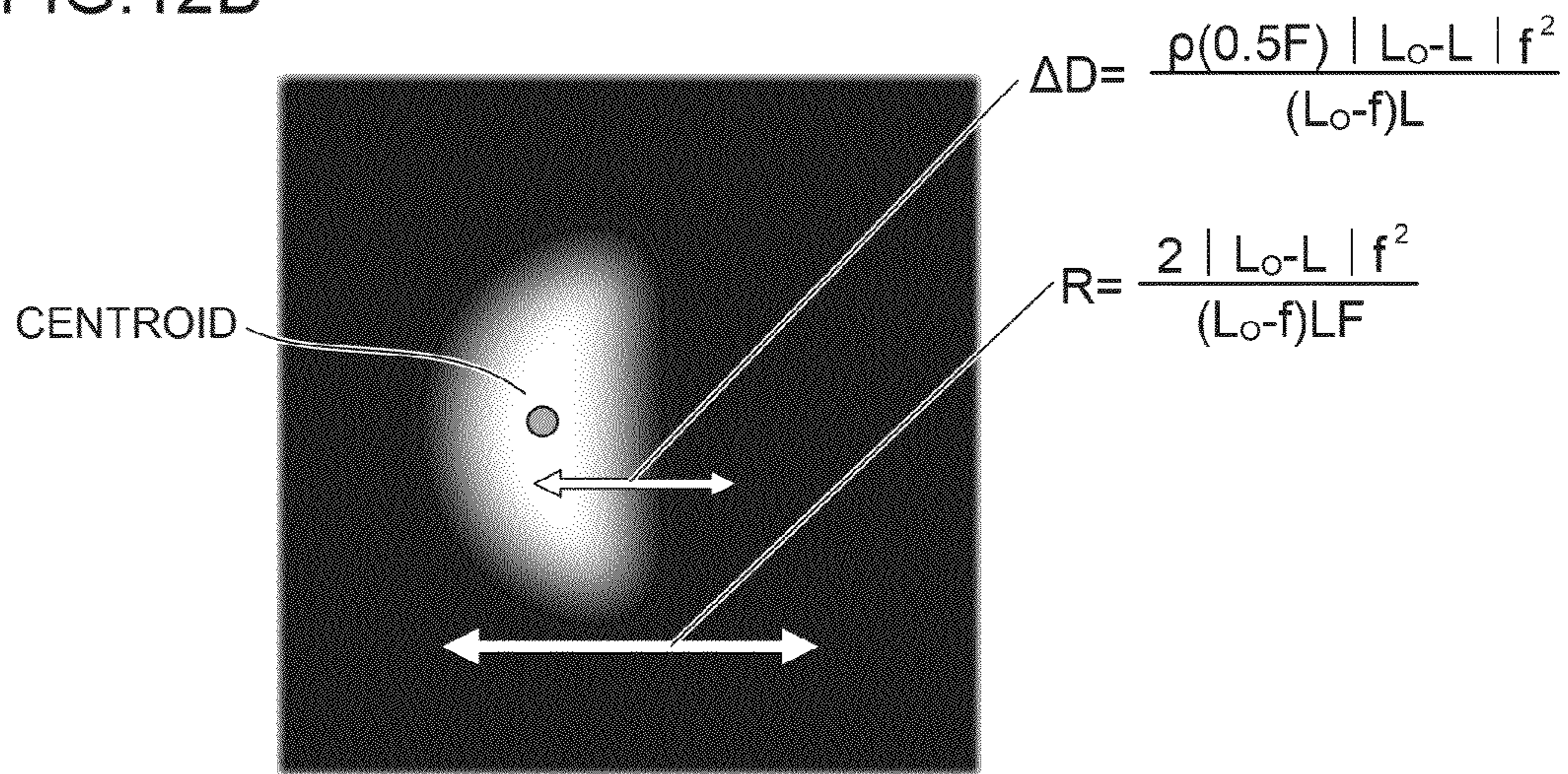
SEMILUNAR FILTER TO BE DESIGNED IN THE EXAMPLE
