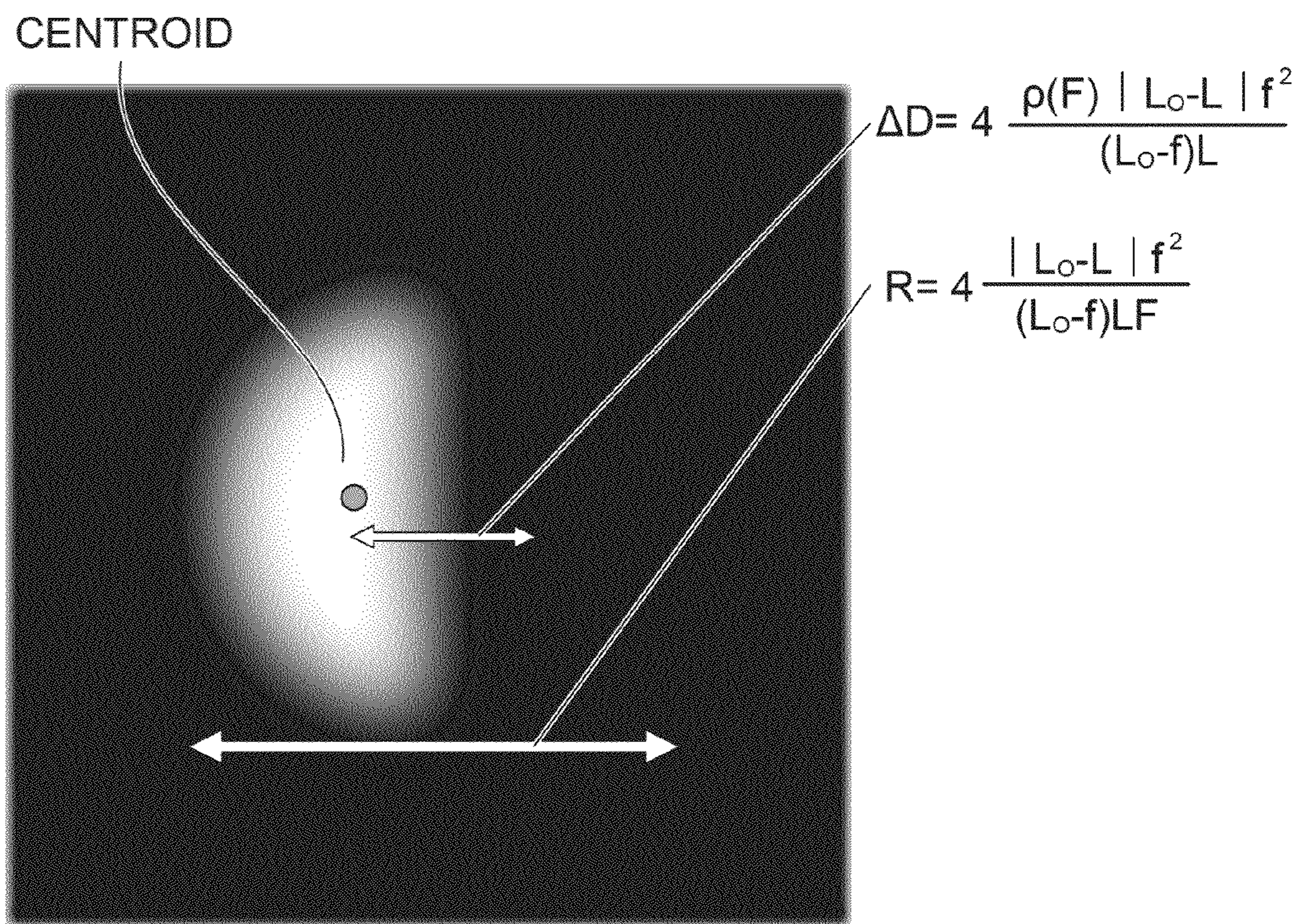
SEMILUNAR FILTER TO BE DESIGNED IN THE EXAMPLE
