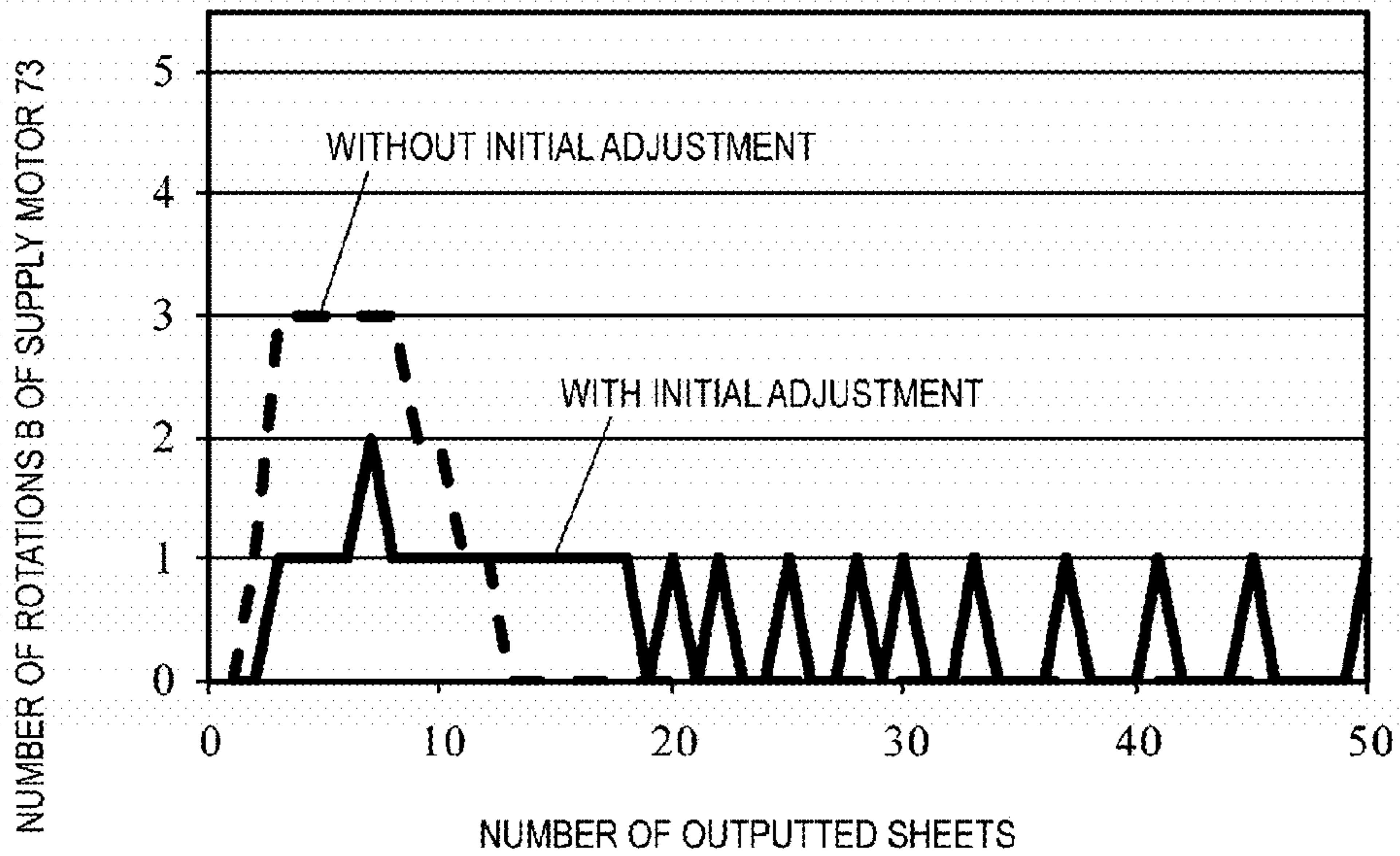
TRANSITION OF NUMBER OF ROTATIONS OF SUPPLY MOTOR (WITH/WITHOUT INITIAL ADJUSTMENT)
