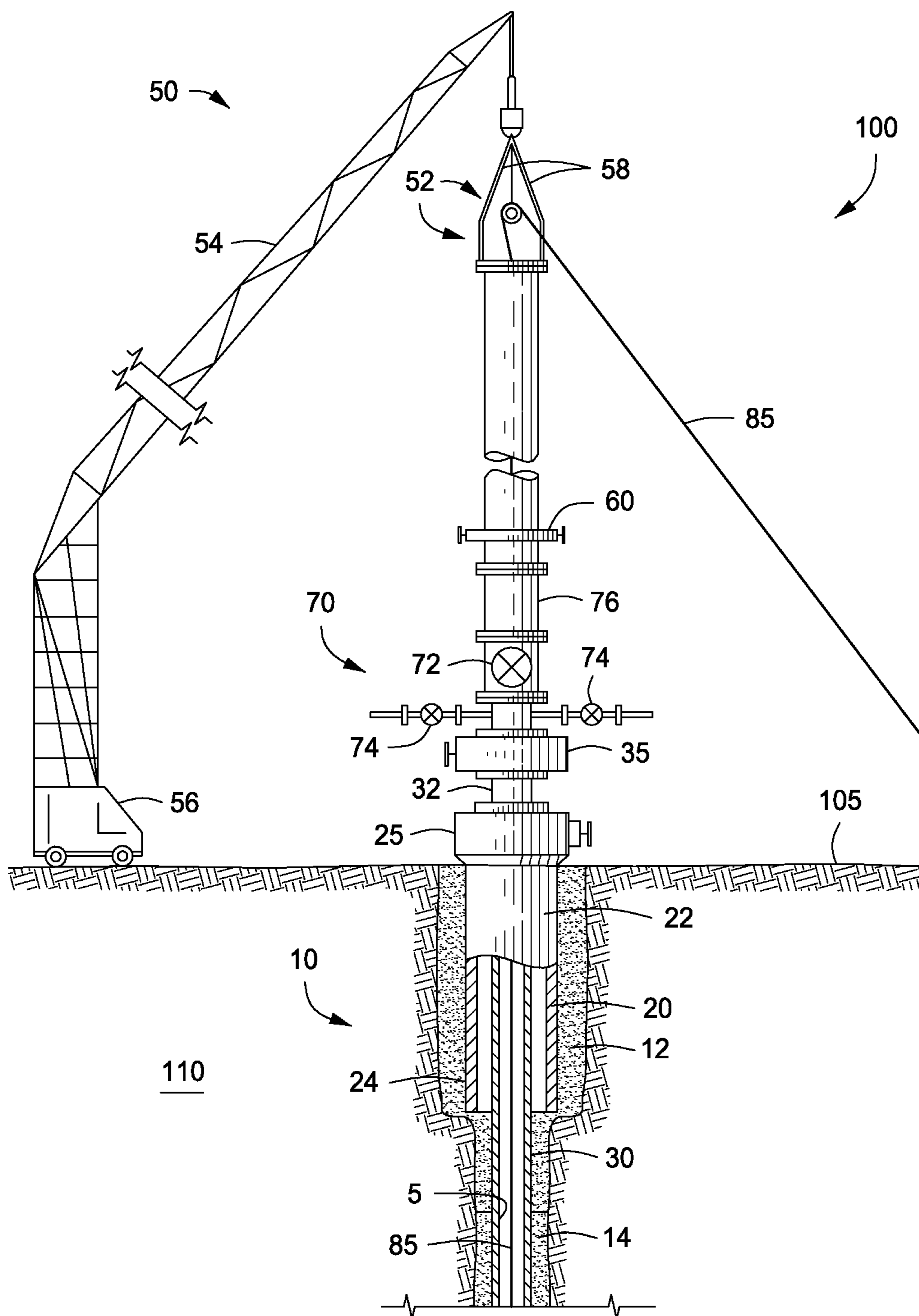
FIG. 1 (PRIOR ART)
