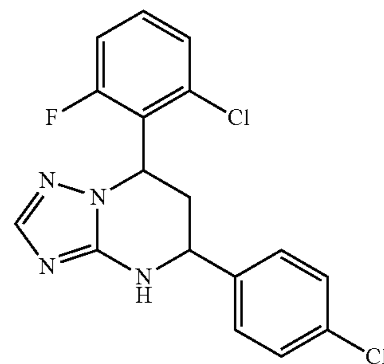
7-(2-chloro-6-fluorophenyl)-5-(4-chlorophenyl)-4,5,6,7-tetrahydro[1,2,4]triazolo[1,5-a]pyrimidine
