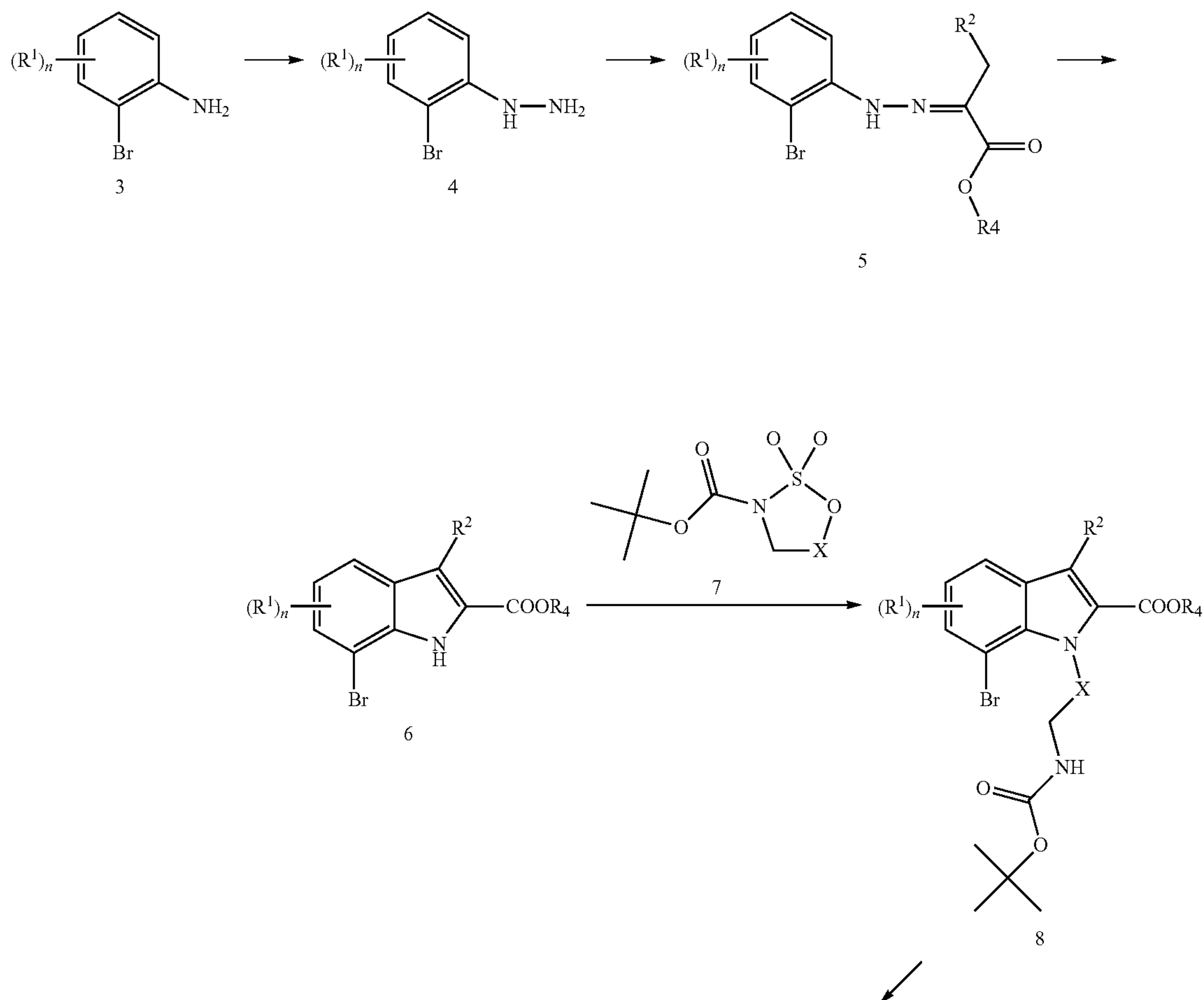
Scheme 1
