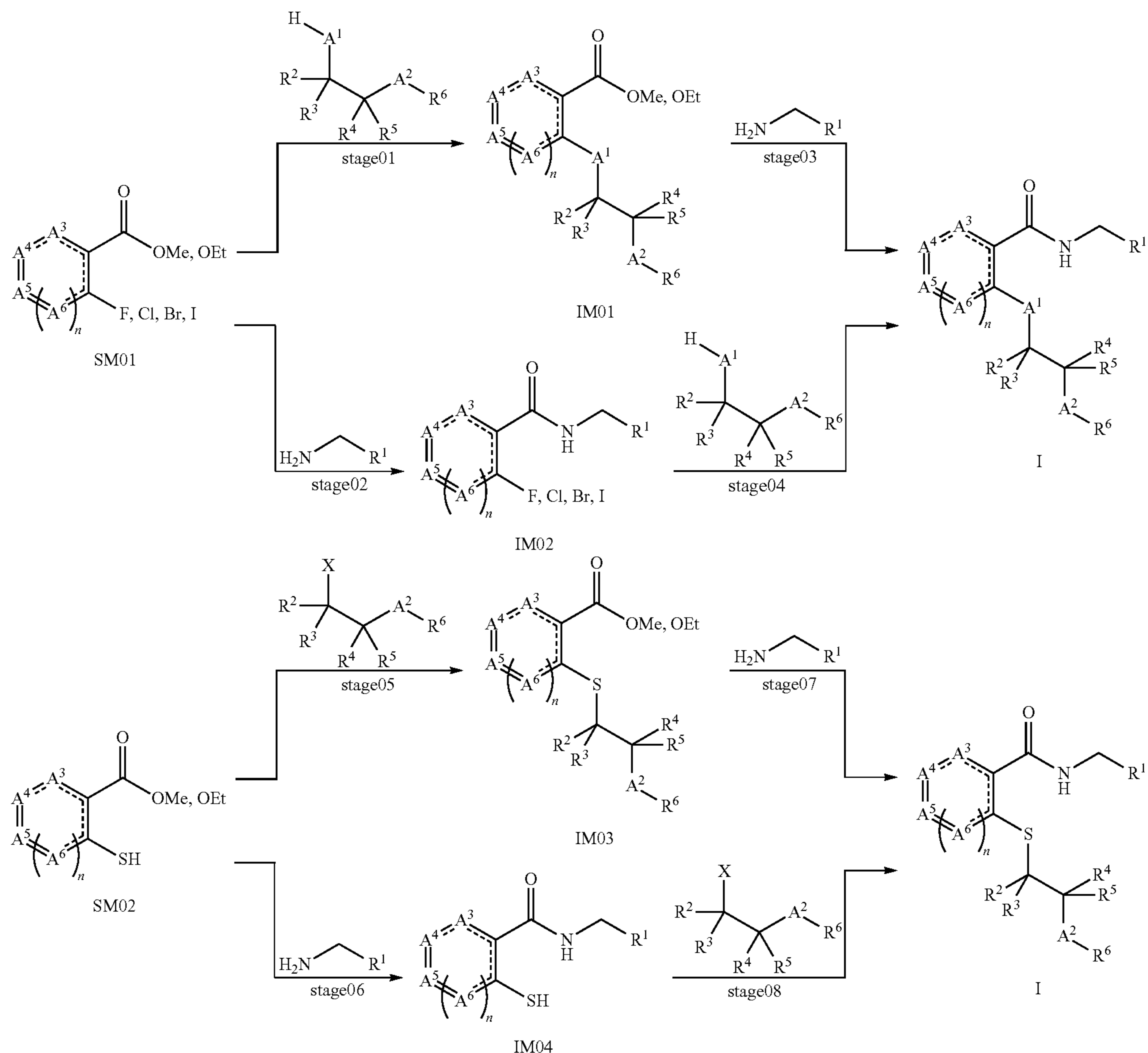
General reaction scheme II:
