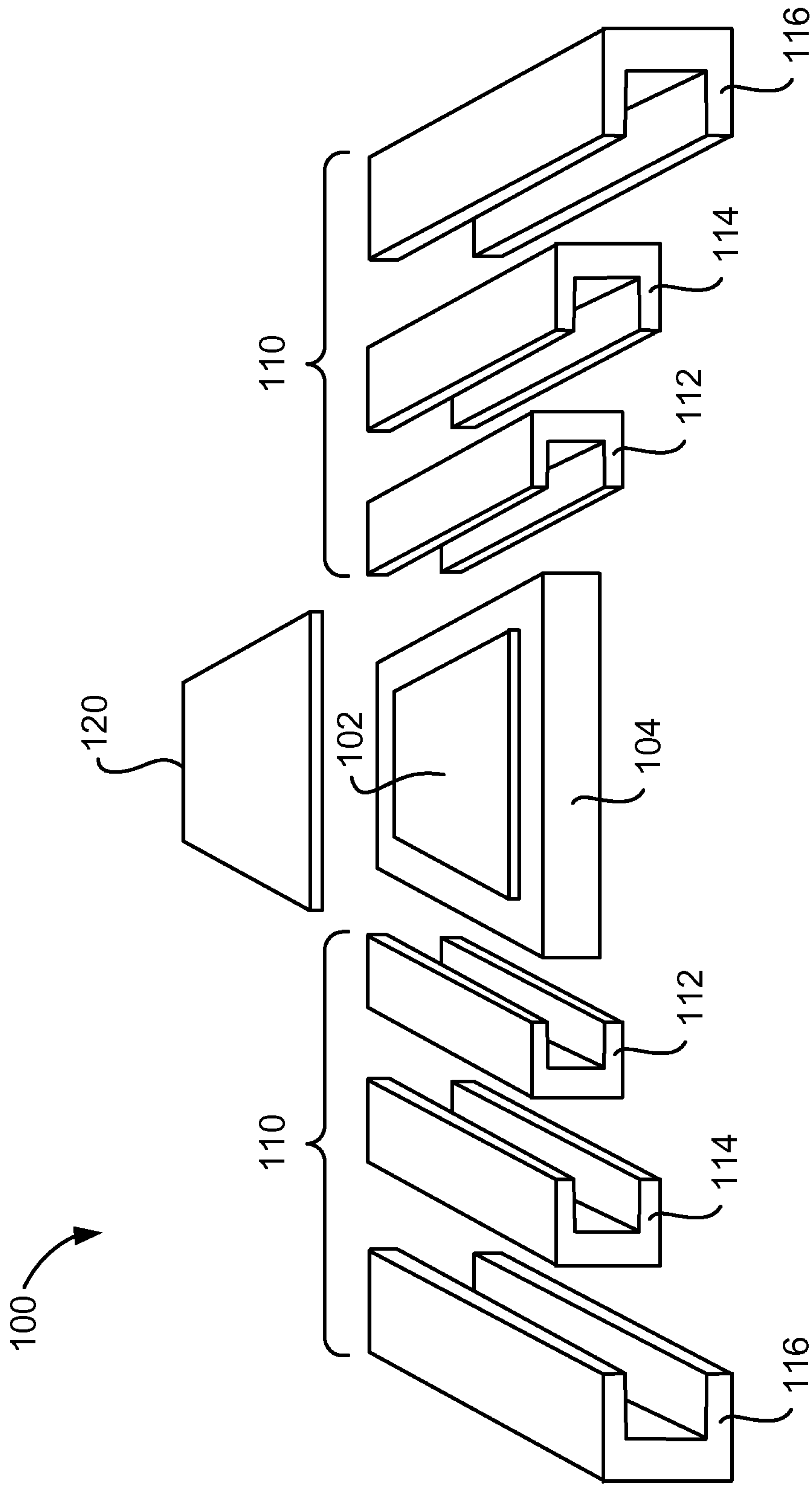
FIG. 1 (Prior Art)
