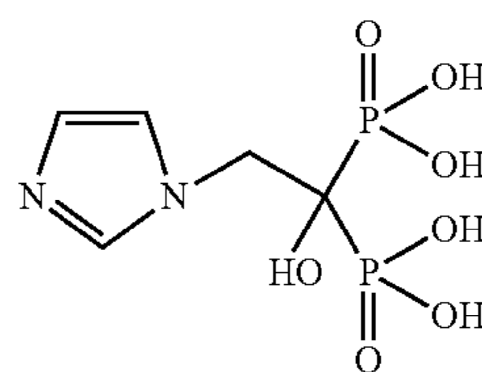
Zoledronic acid
