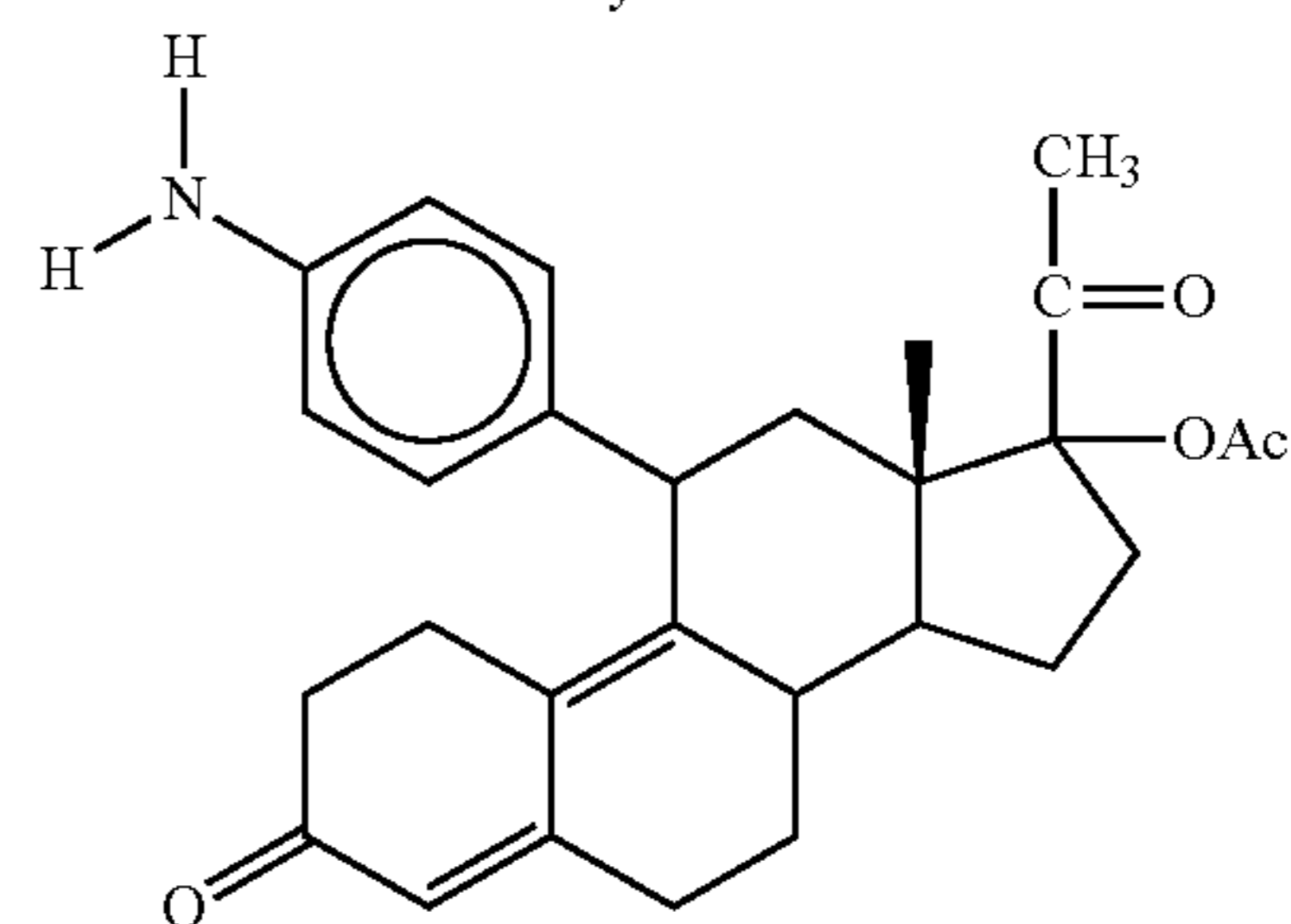
didemethylated CDB-2914
