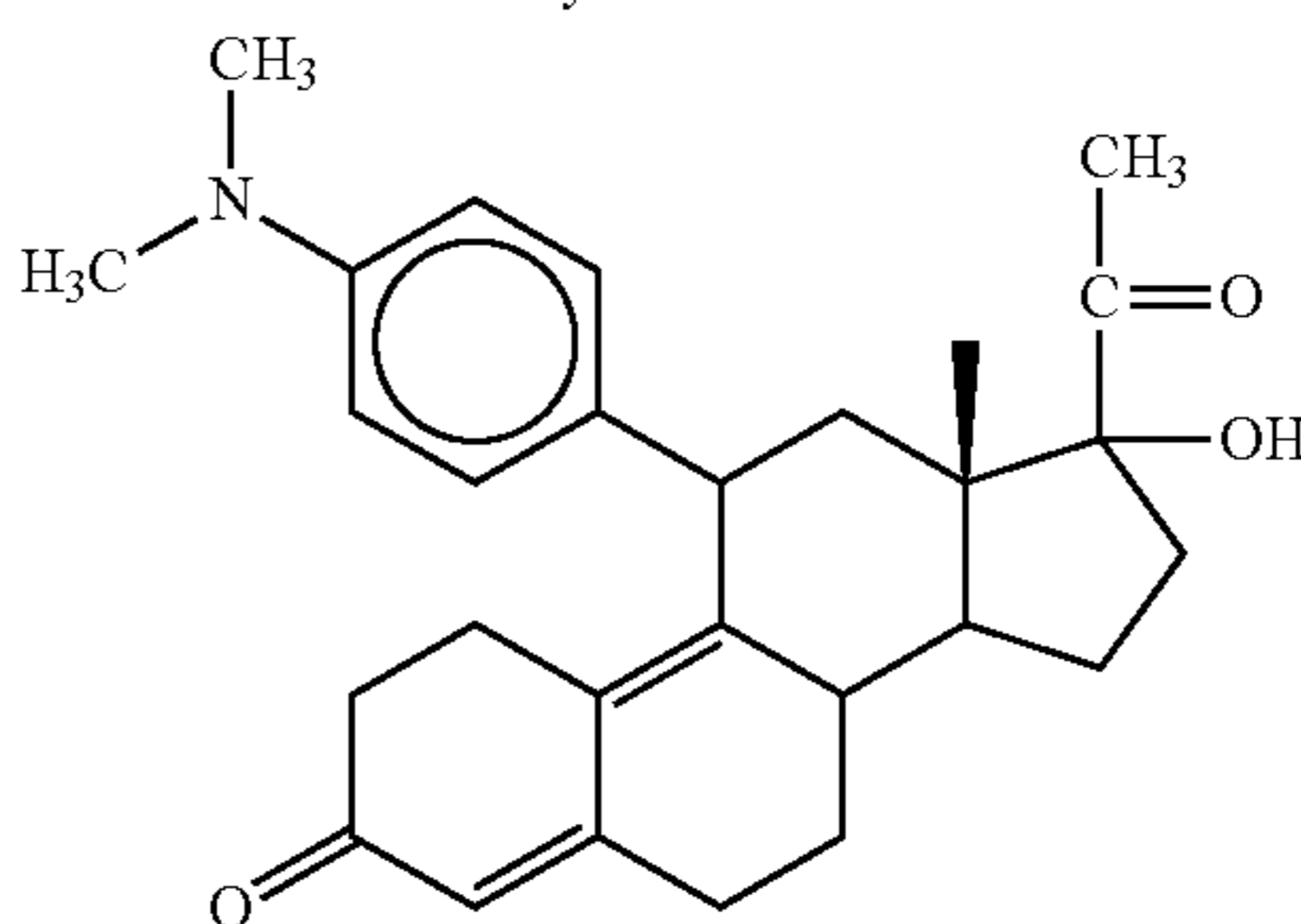
17 \alpha -hydroxy CDB-2914
