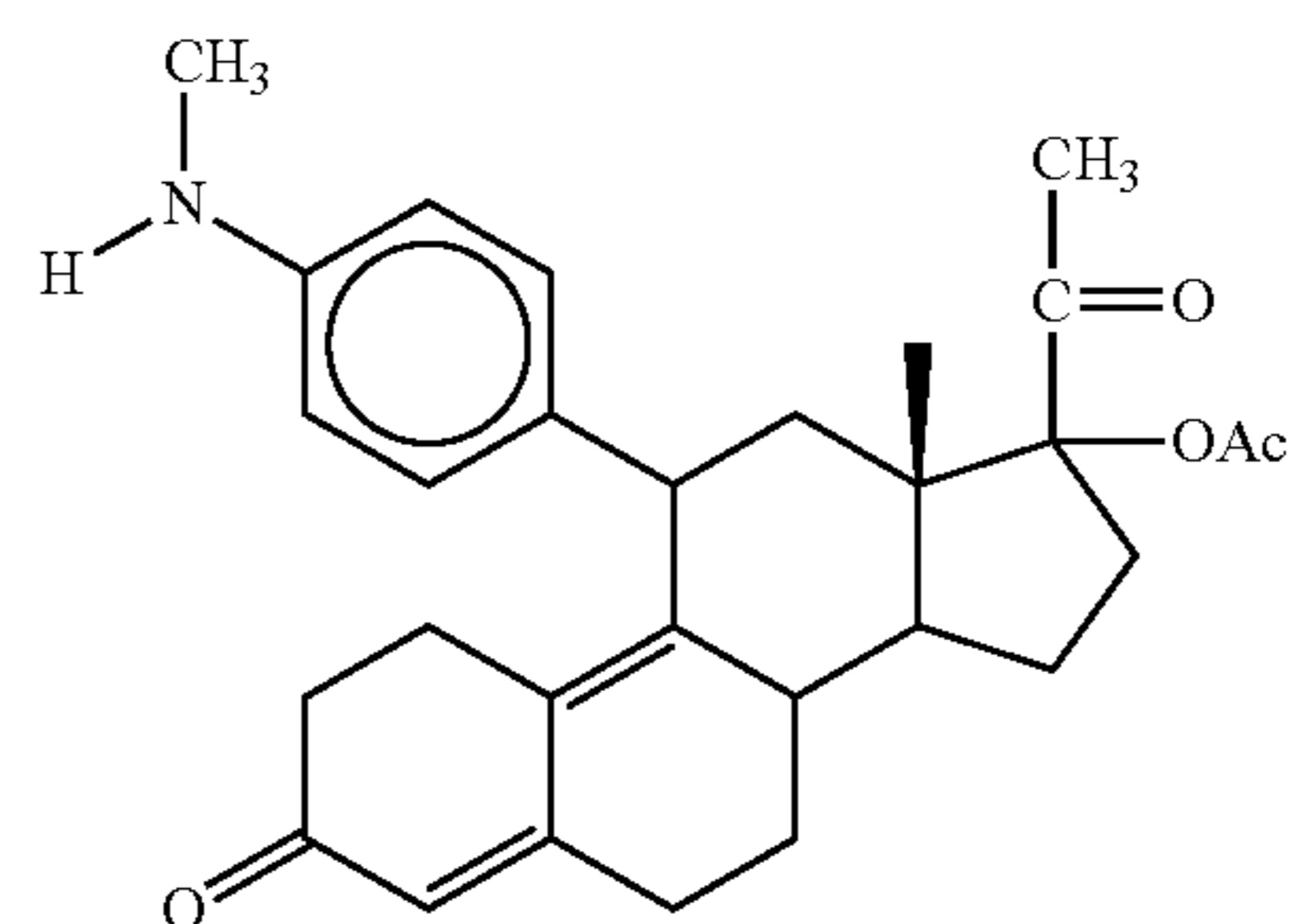
monodemethylated CDB-2914
