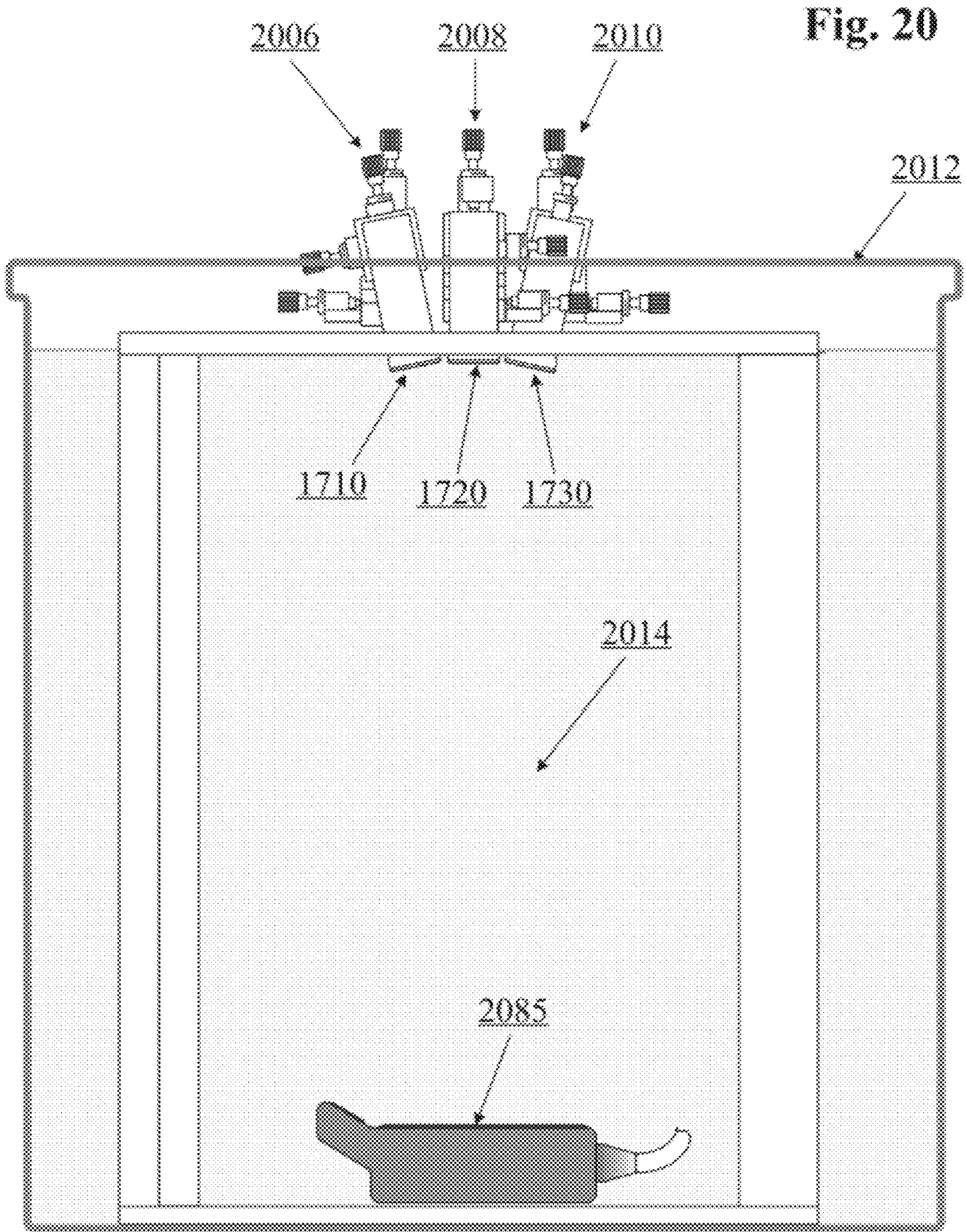
Assembled test fixture in tank.
