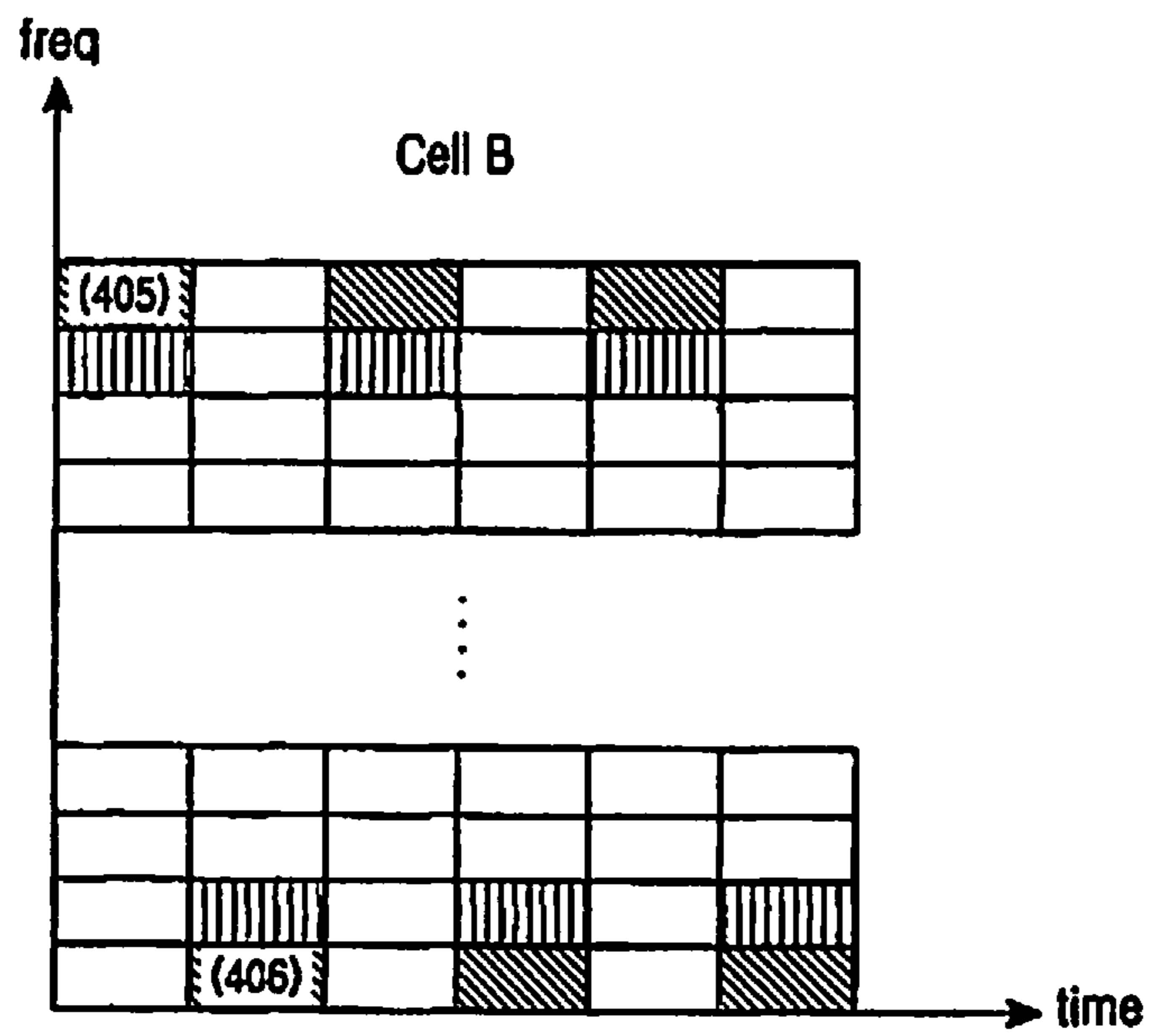
FIG.4 (PRIOR ART)
