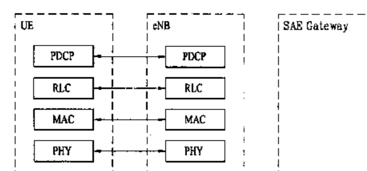
(B) USER-PLANE PROTOCOL STACK
