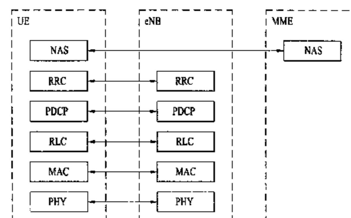
(A) CONTROL-PLANE PROTOCOL STACK
