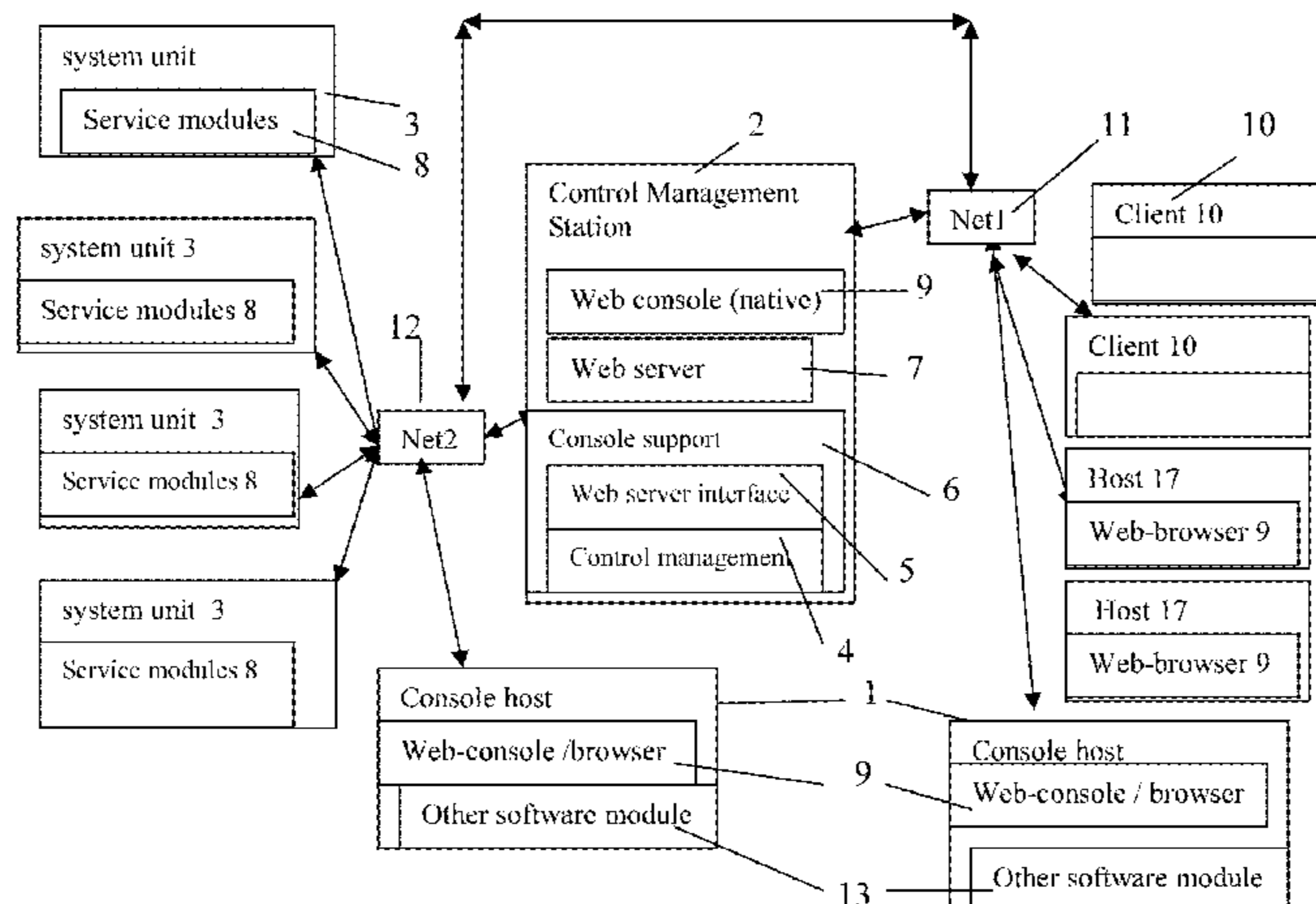
A Typical CCDSVM with Multiple Clients
