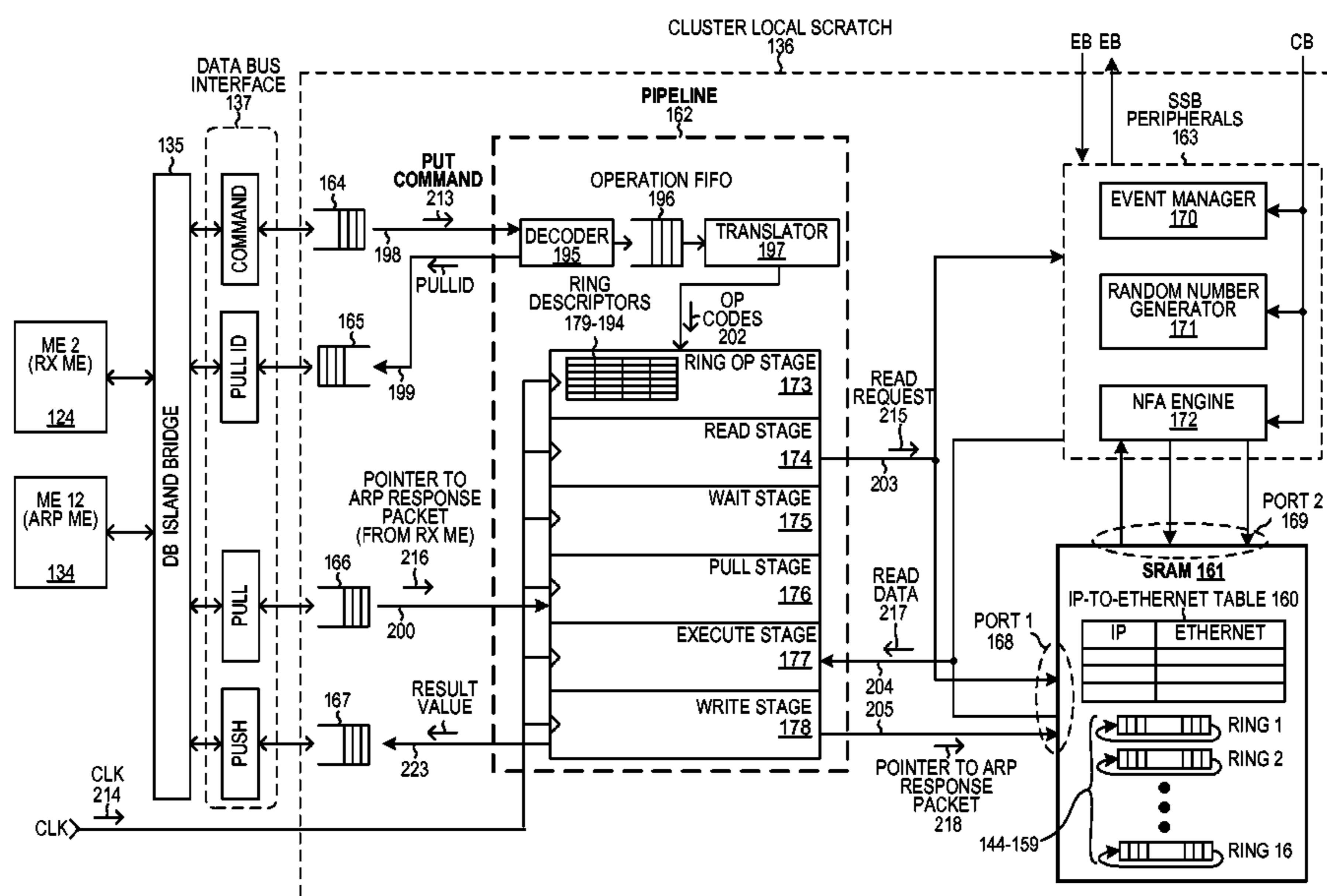
CLUSTER LOCAL SCRATCH ("PUT INTO RING" EXAMPLE)
