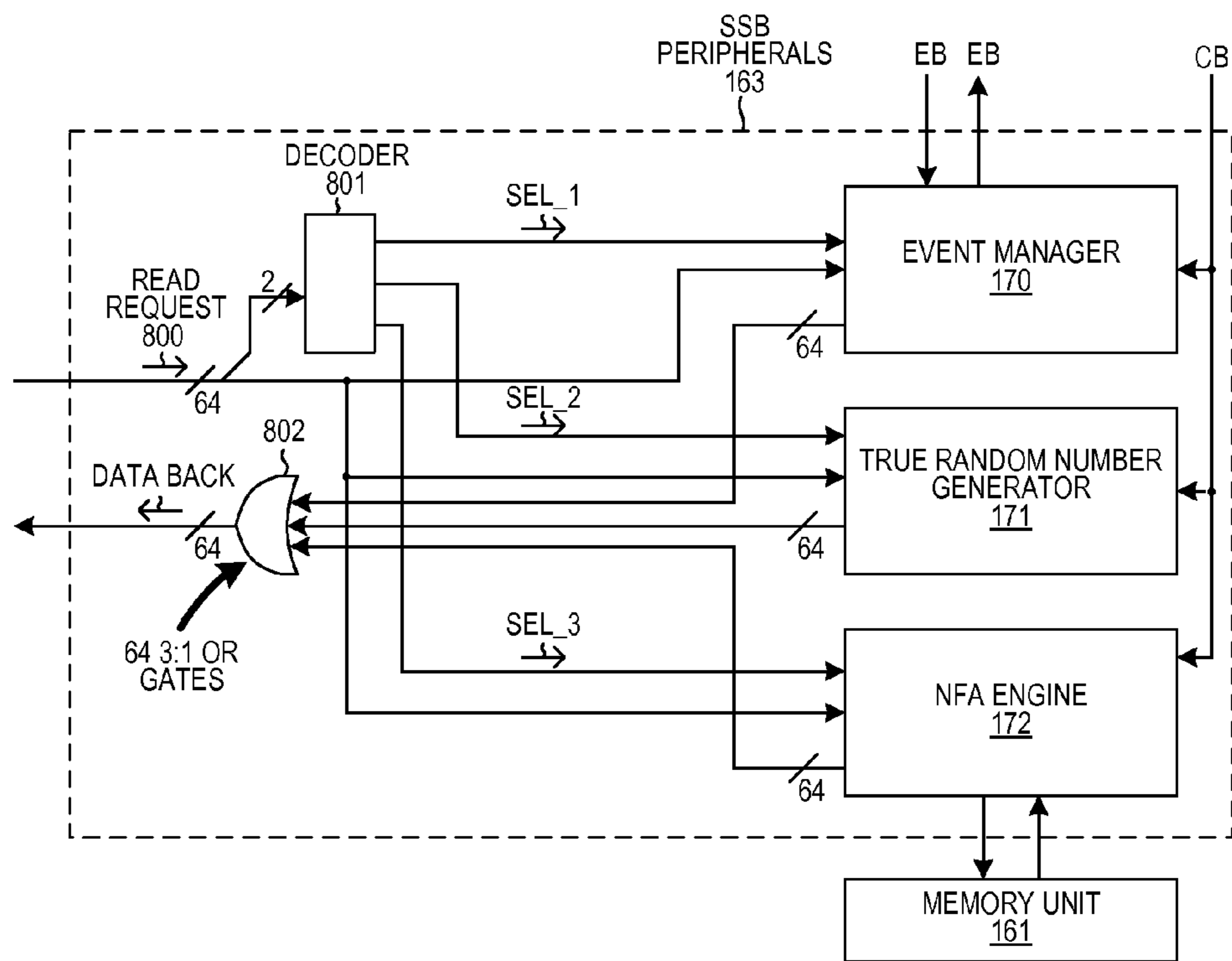
SSB PERIPHERALS BLOCK FIG. 25
