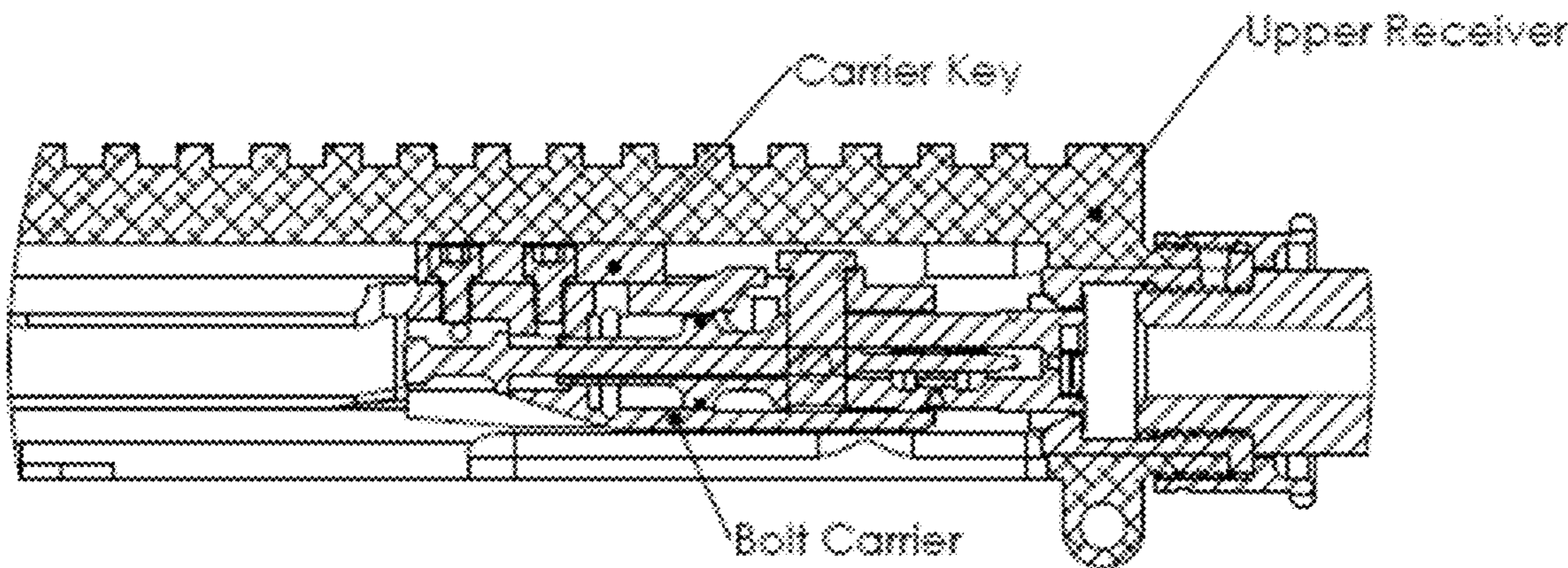
DETAIL C SCALE 2:1.5
