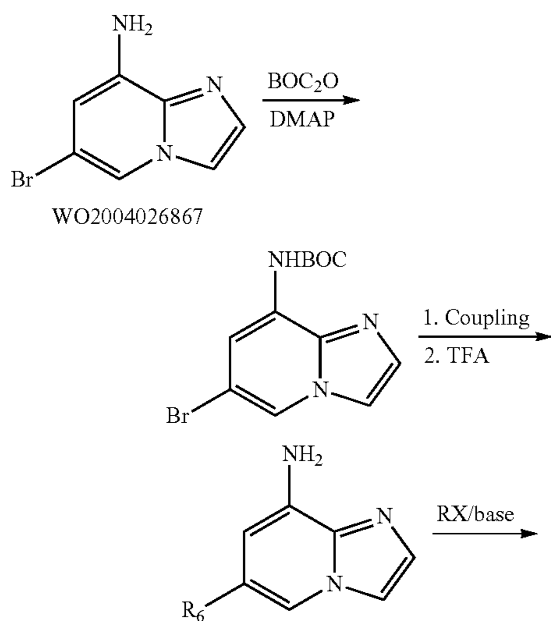
Scheme VIII: Preparation of C-6 and C-8 Substituted 3-Ethynylimidazo[1,2-a]pyridines.
