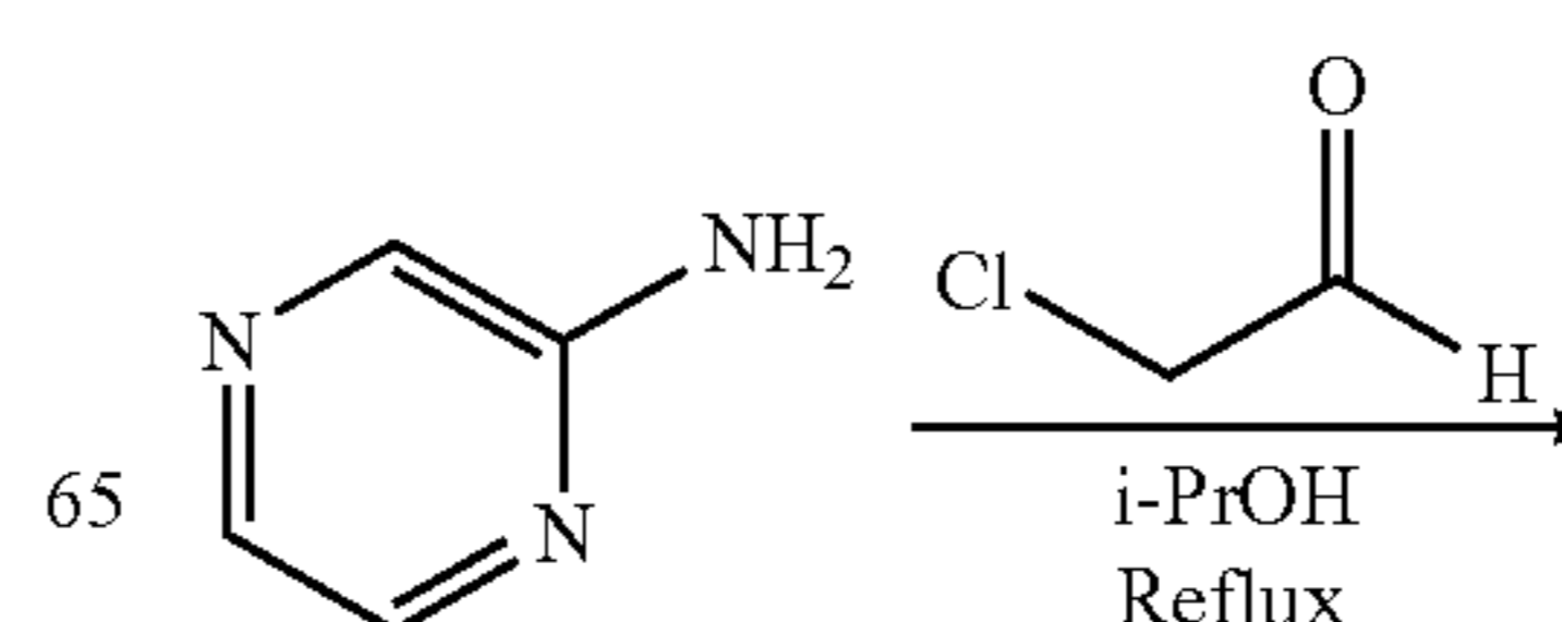
Scheme III: Preparation of 3-Ethynylimidazo[1,2-a]pyrazine
