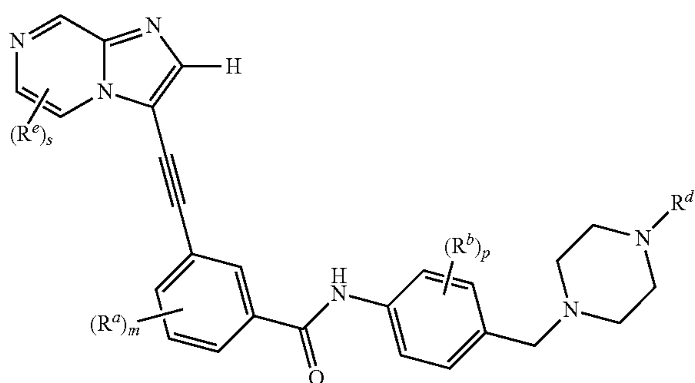
Formula IIIa
