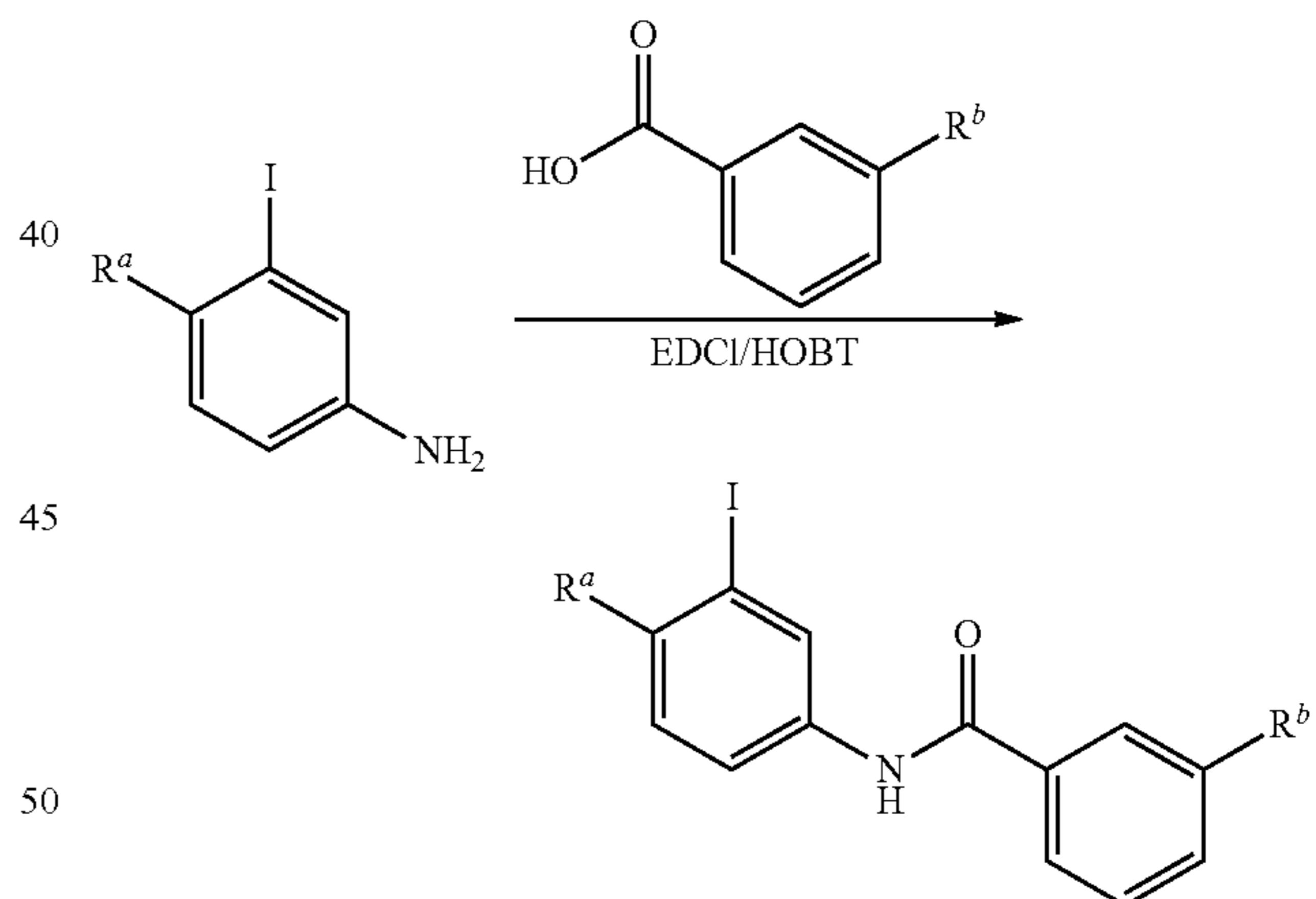
Scheme IX
