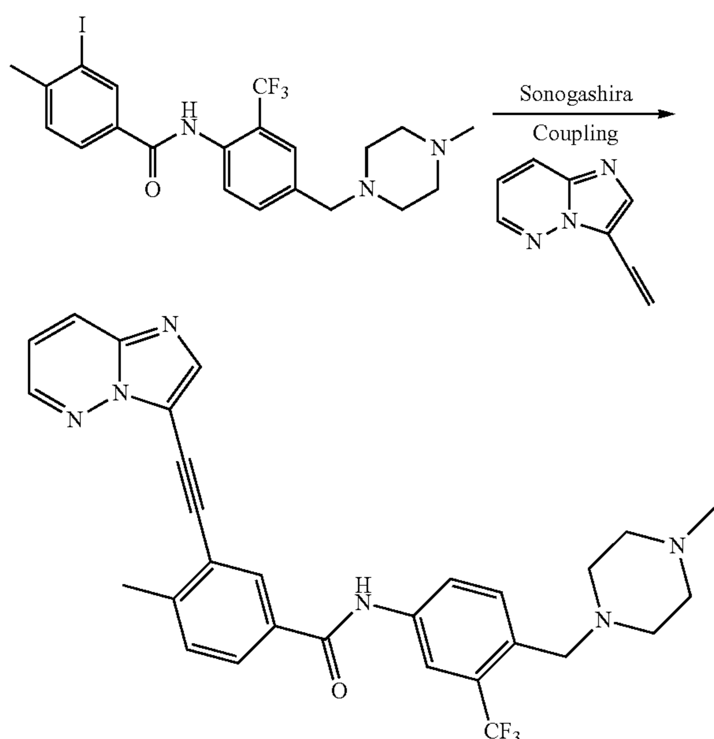
Scheme XIV
