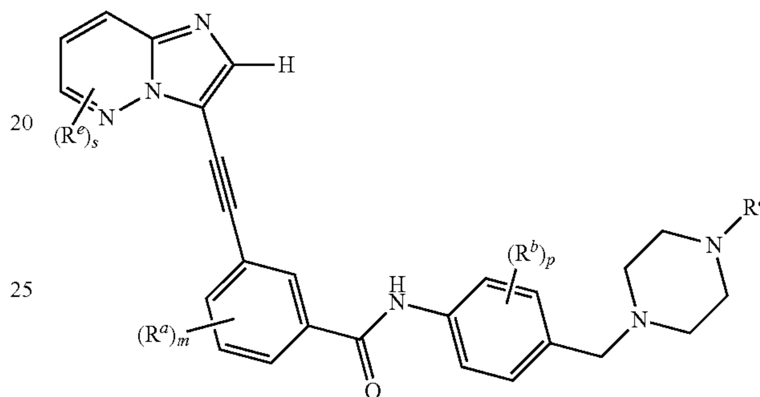
Formula IIIc
