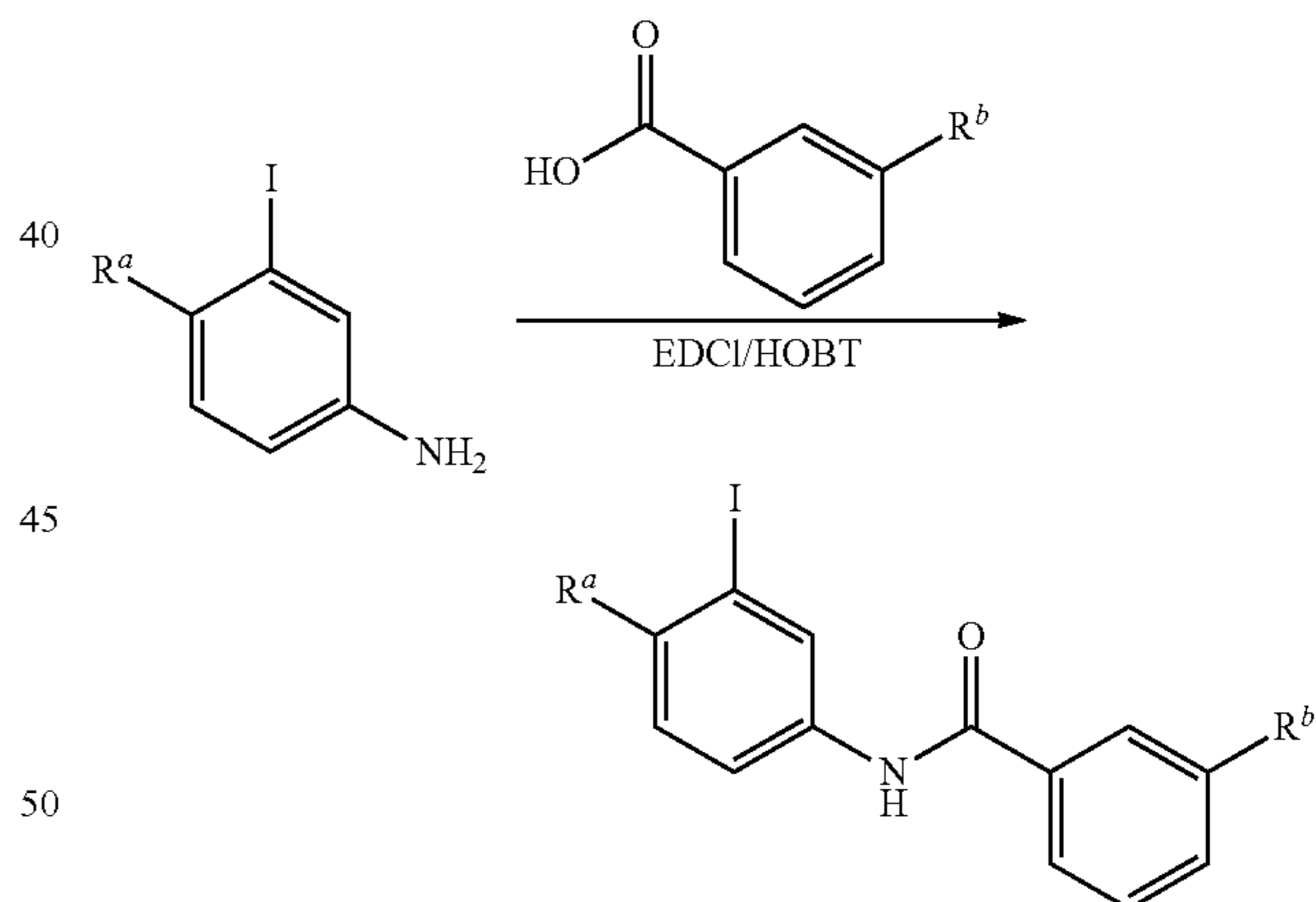
Scheme IX
