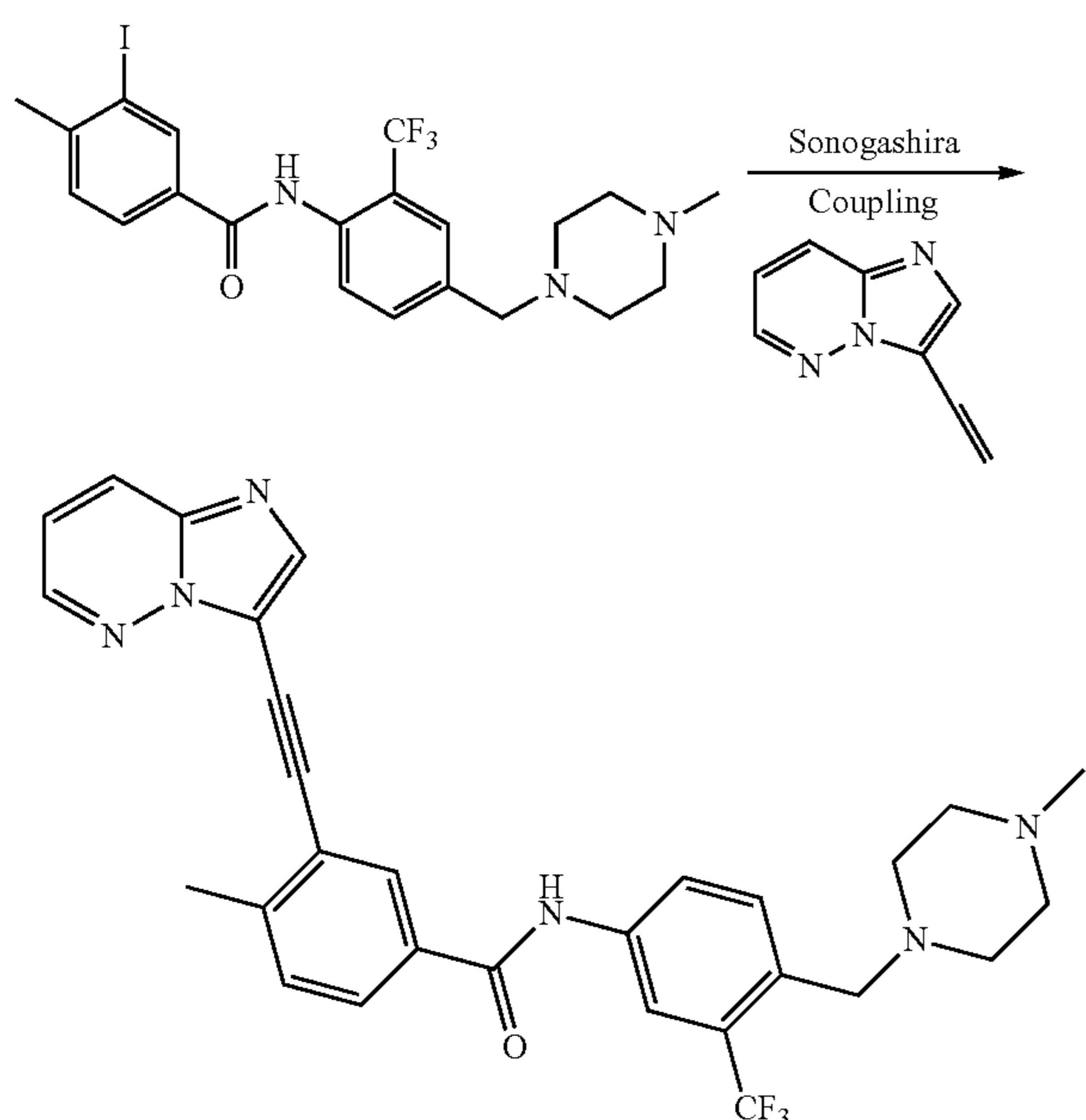
Scheme XIV
