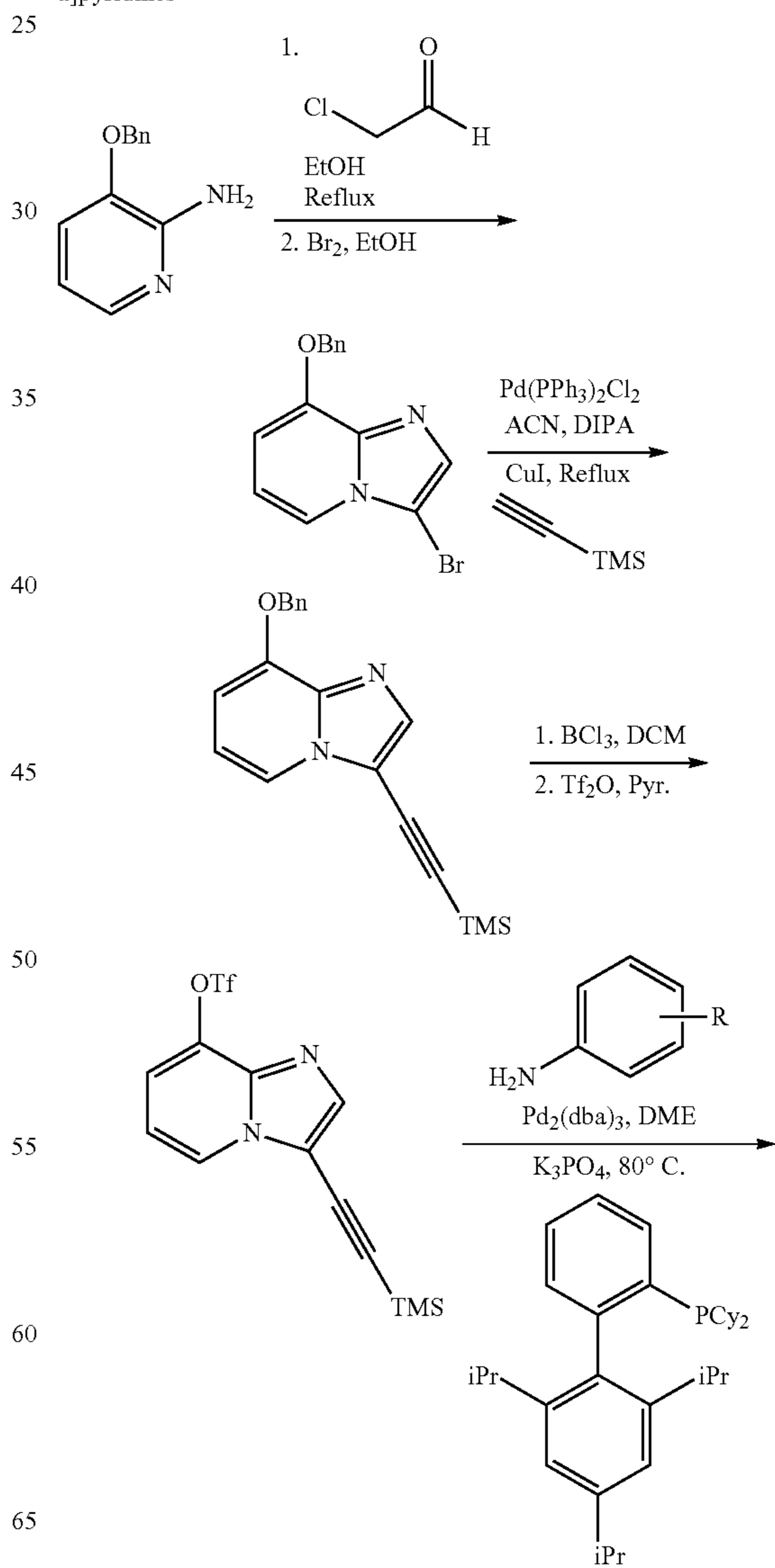
Scheme VI: Preparation of C-8 Amino Substituted 3-Ethynylimidazo[1,2-a]pyridines
