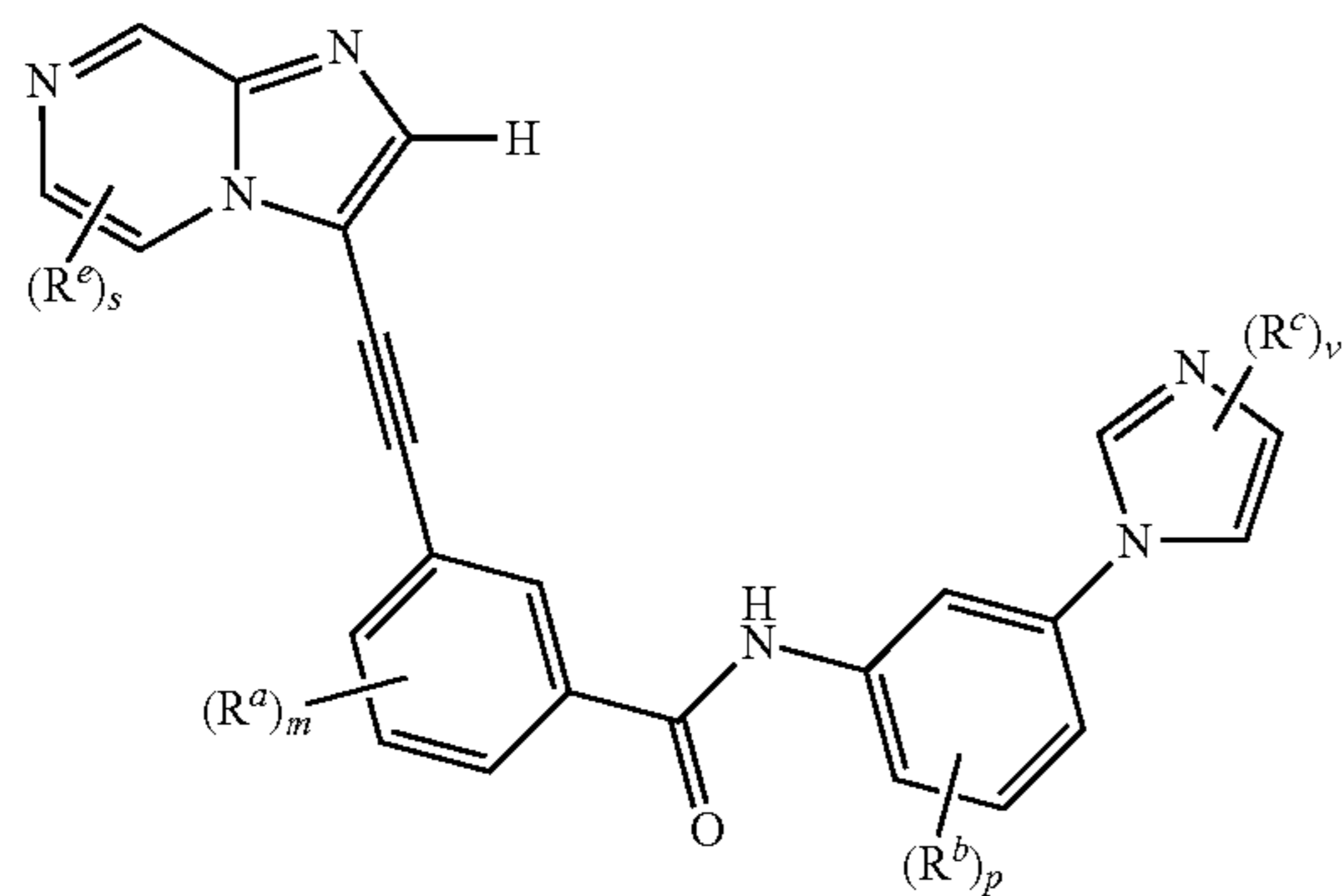
Formula IIa
