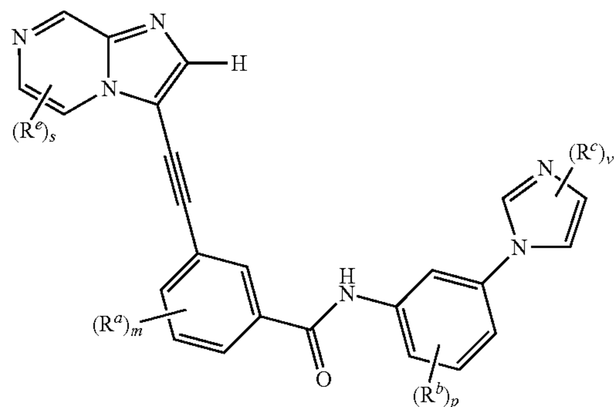
Formula IIa
