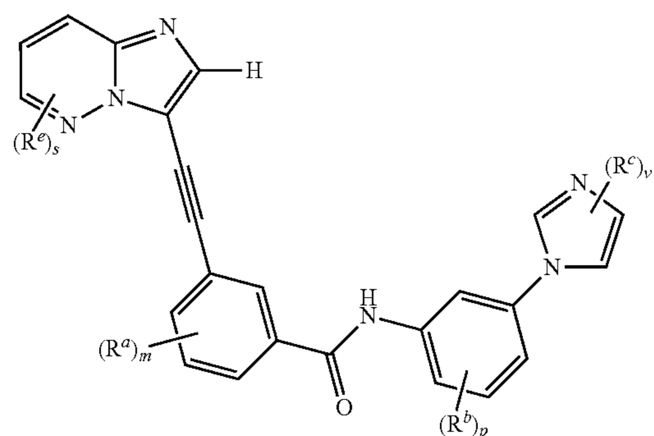
Formula IIc
