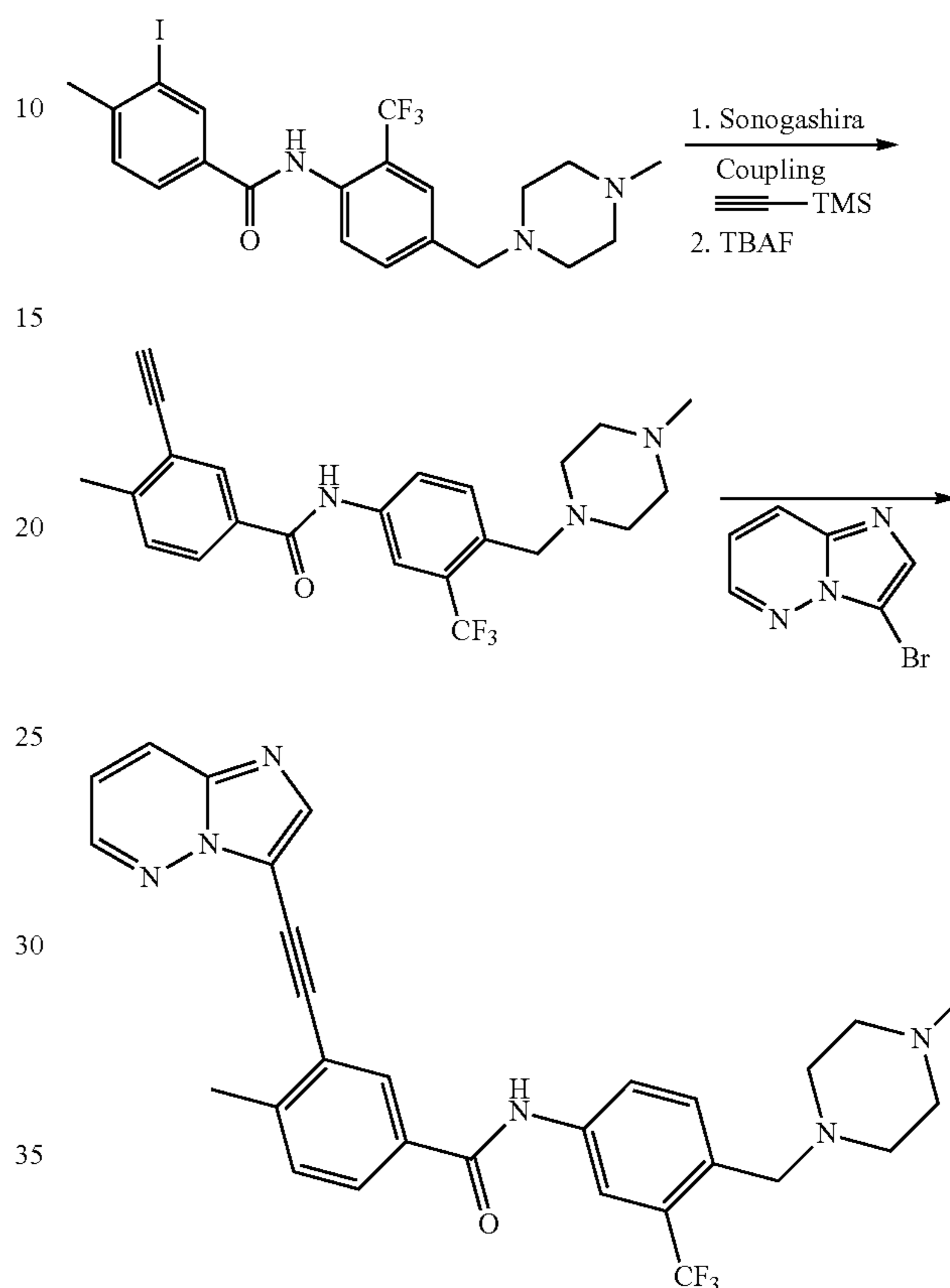
Scheme XV
