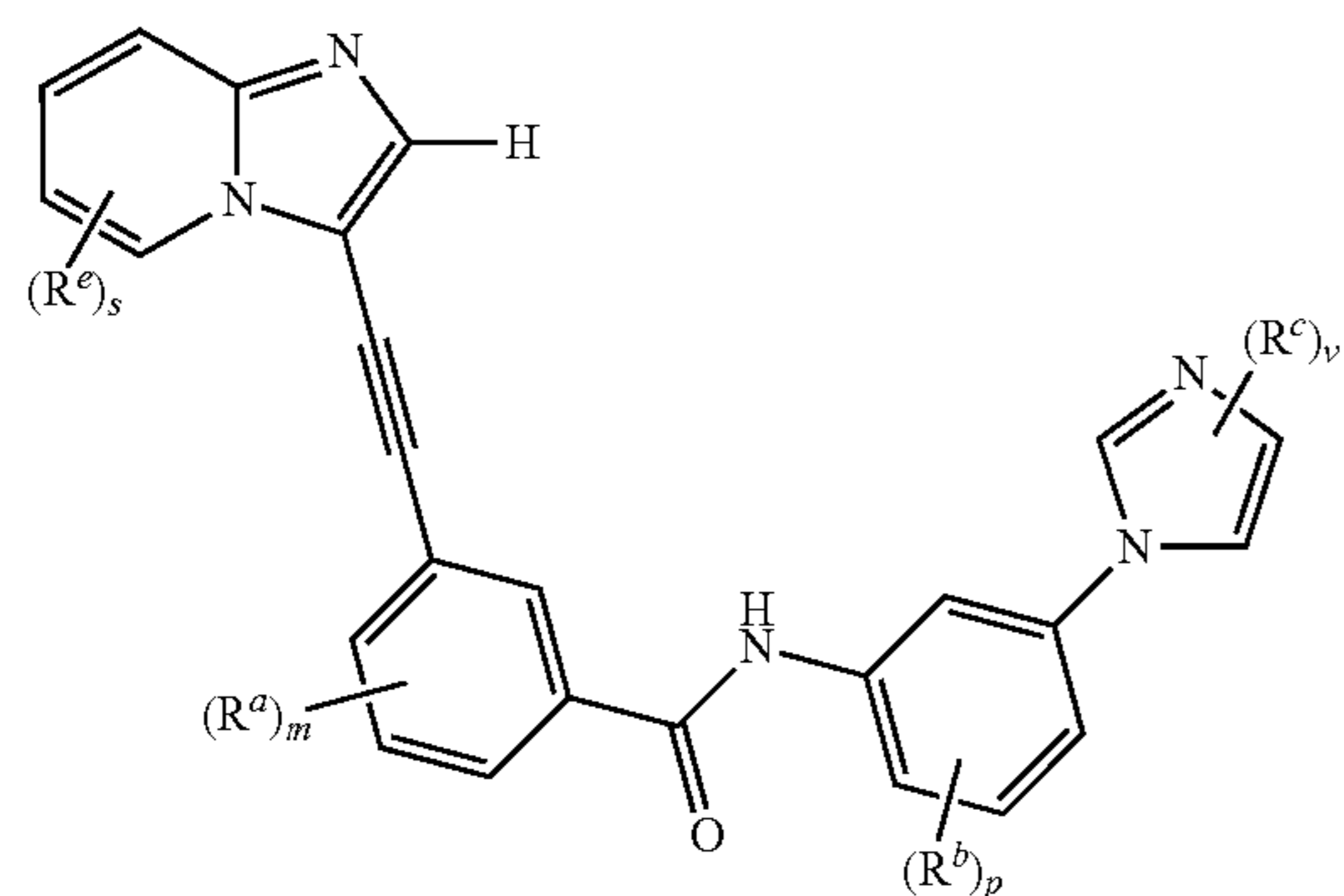
Formula IIb
