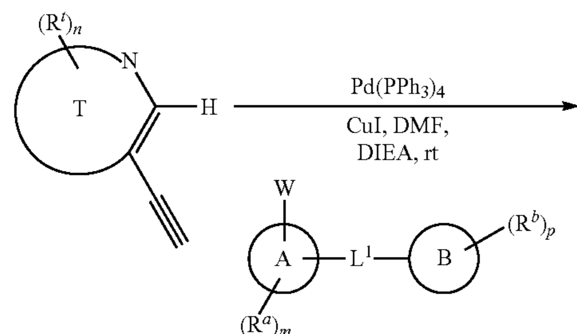
Scheme I: Sonogashira Coupling Reaction
