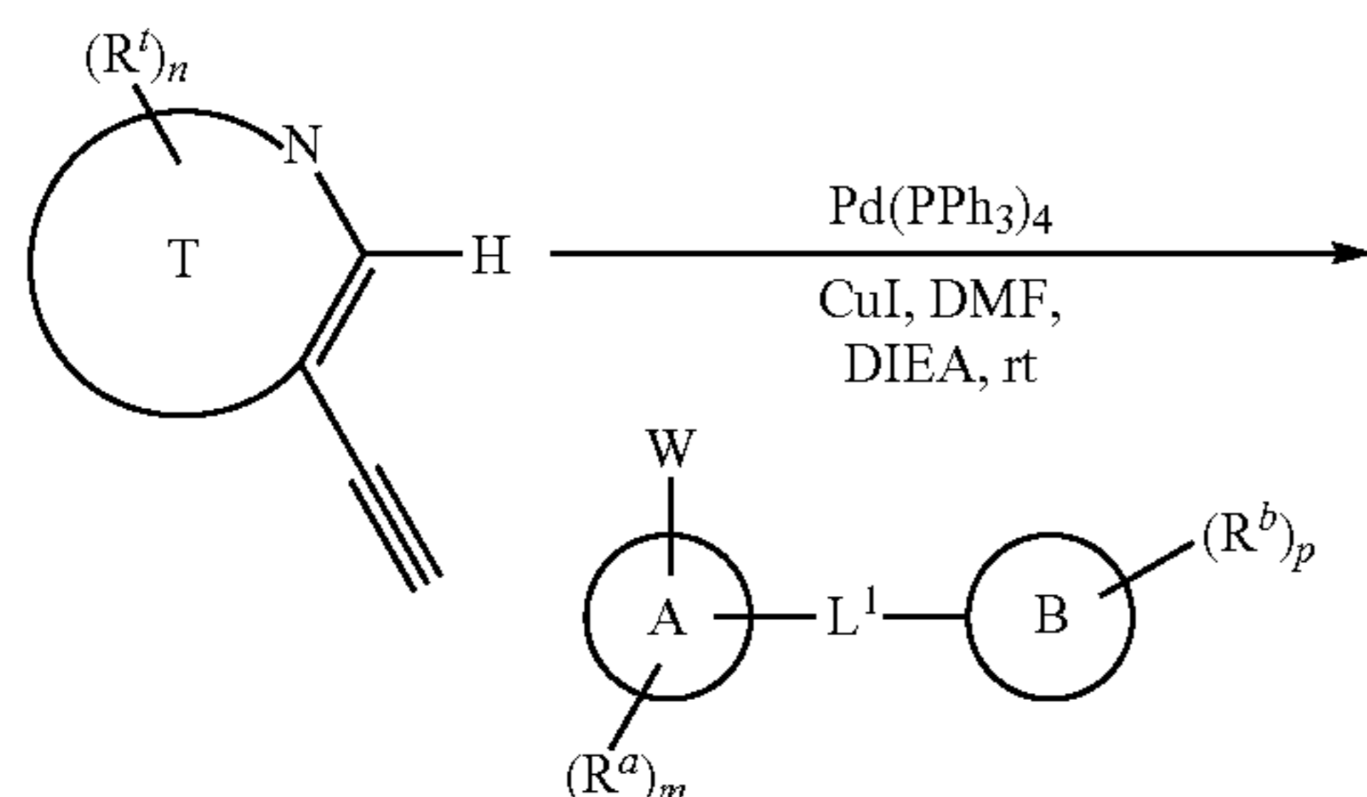
Scheme I: Sonogashira Coupling Reaction
