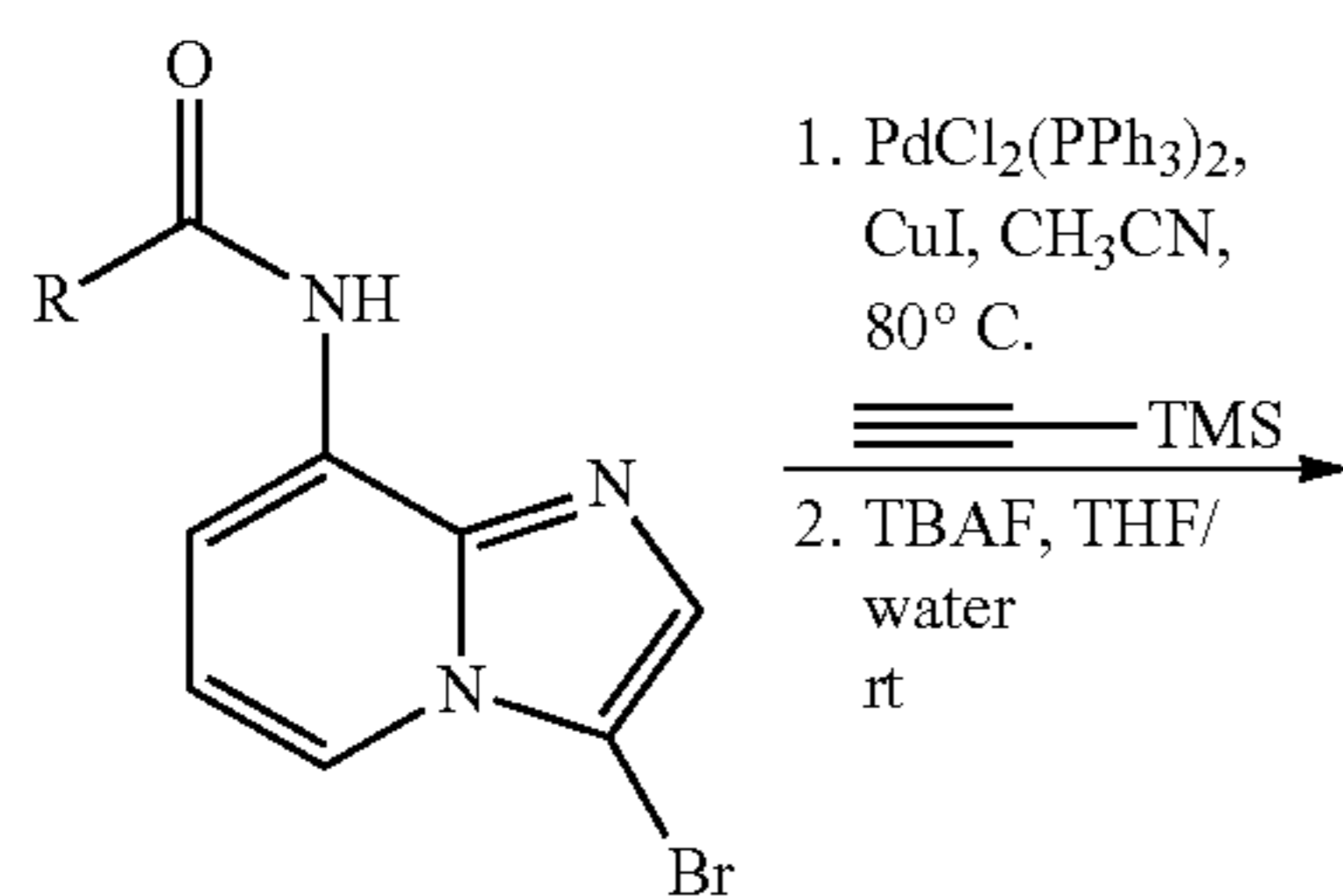
Scheme VII: Preparation of C-8 substituted 3-Ethynylimidazo[1,2-a]pyridines
