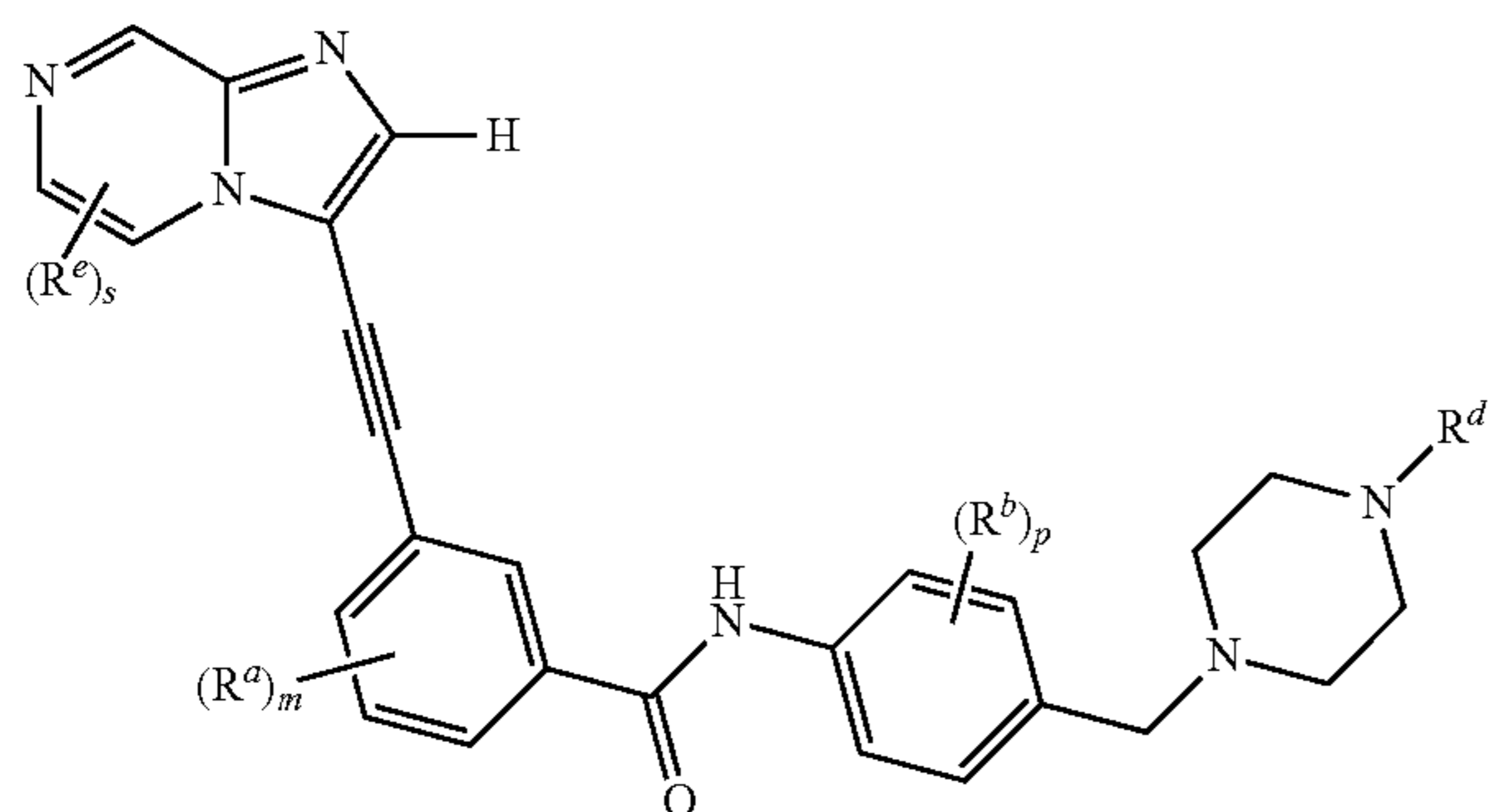
Formula IIIa
