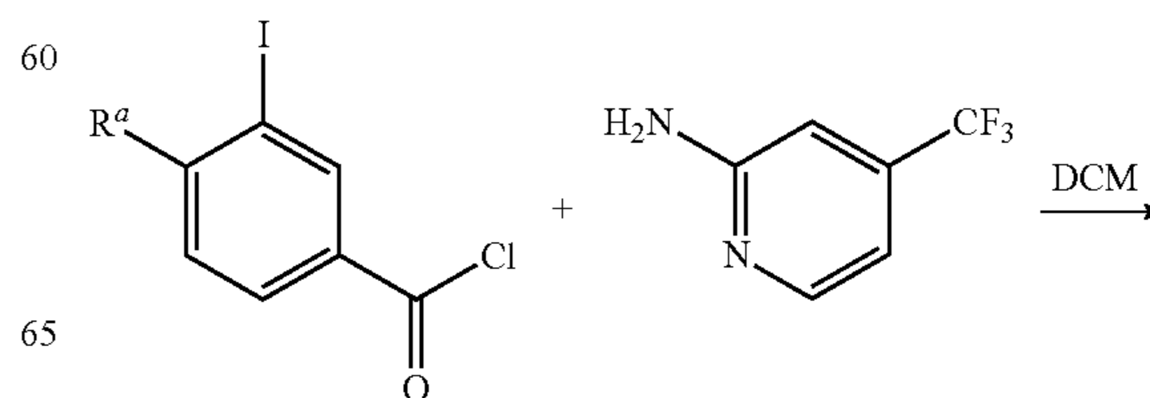
Scheme X
