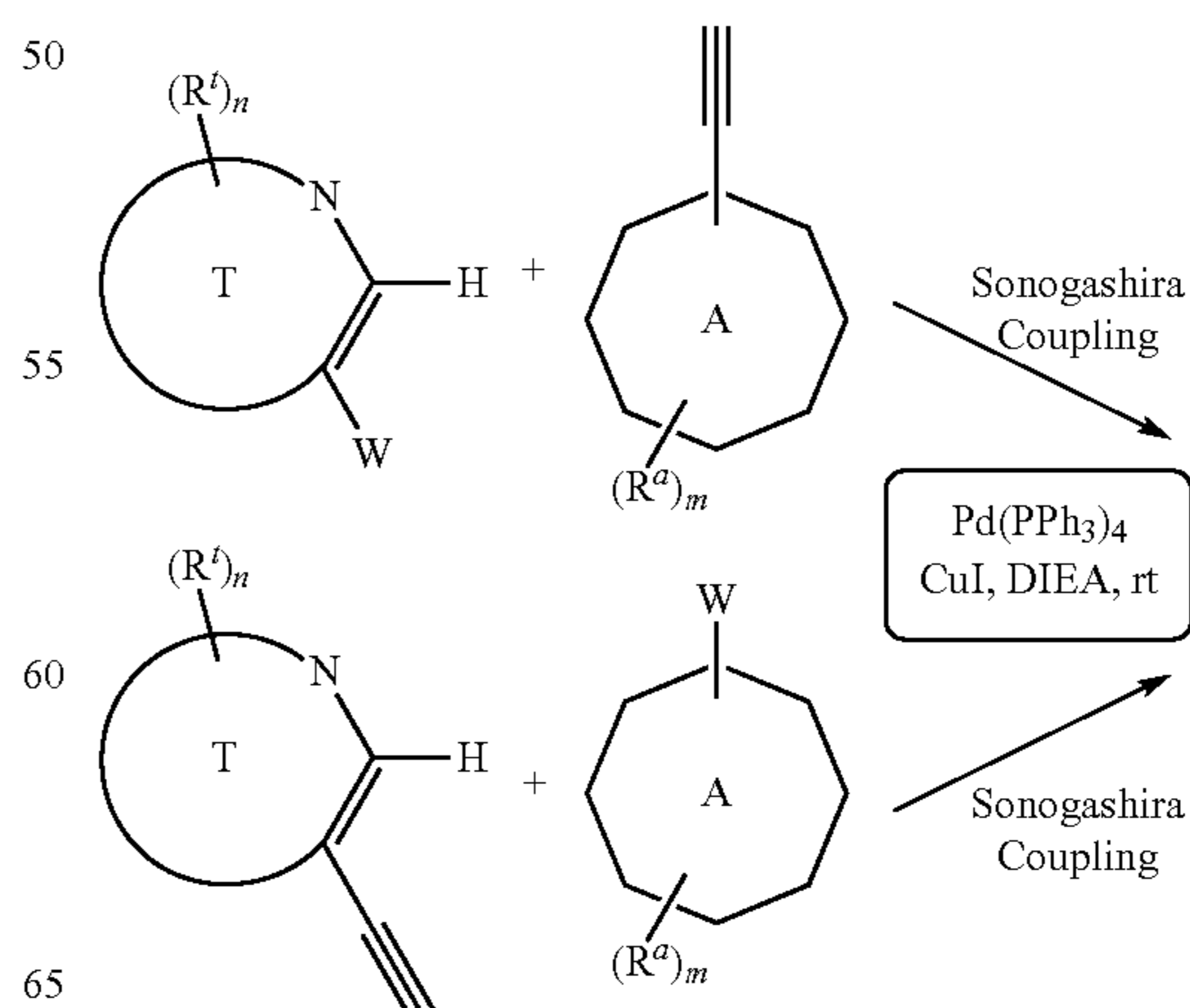
Scheme XVI
