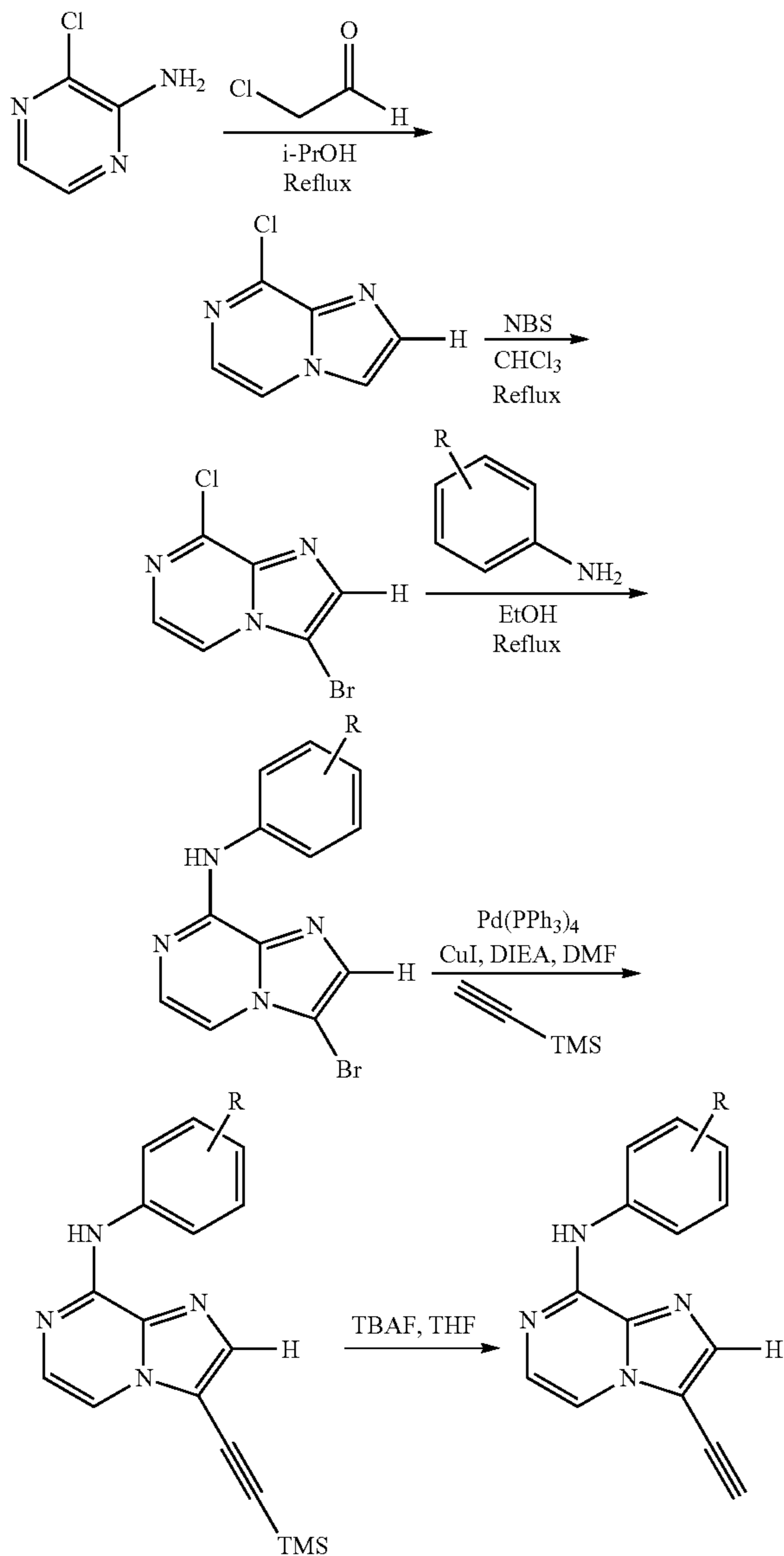
Scheme IV: Preparation of C-8 Substituted 3-Ethynylimidazo[1,2-a]pyrazines
