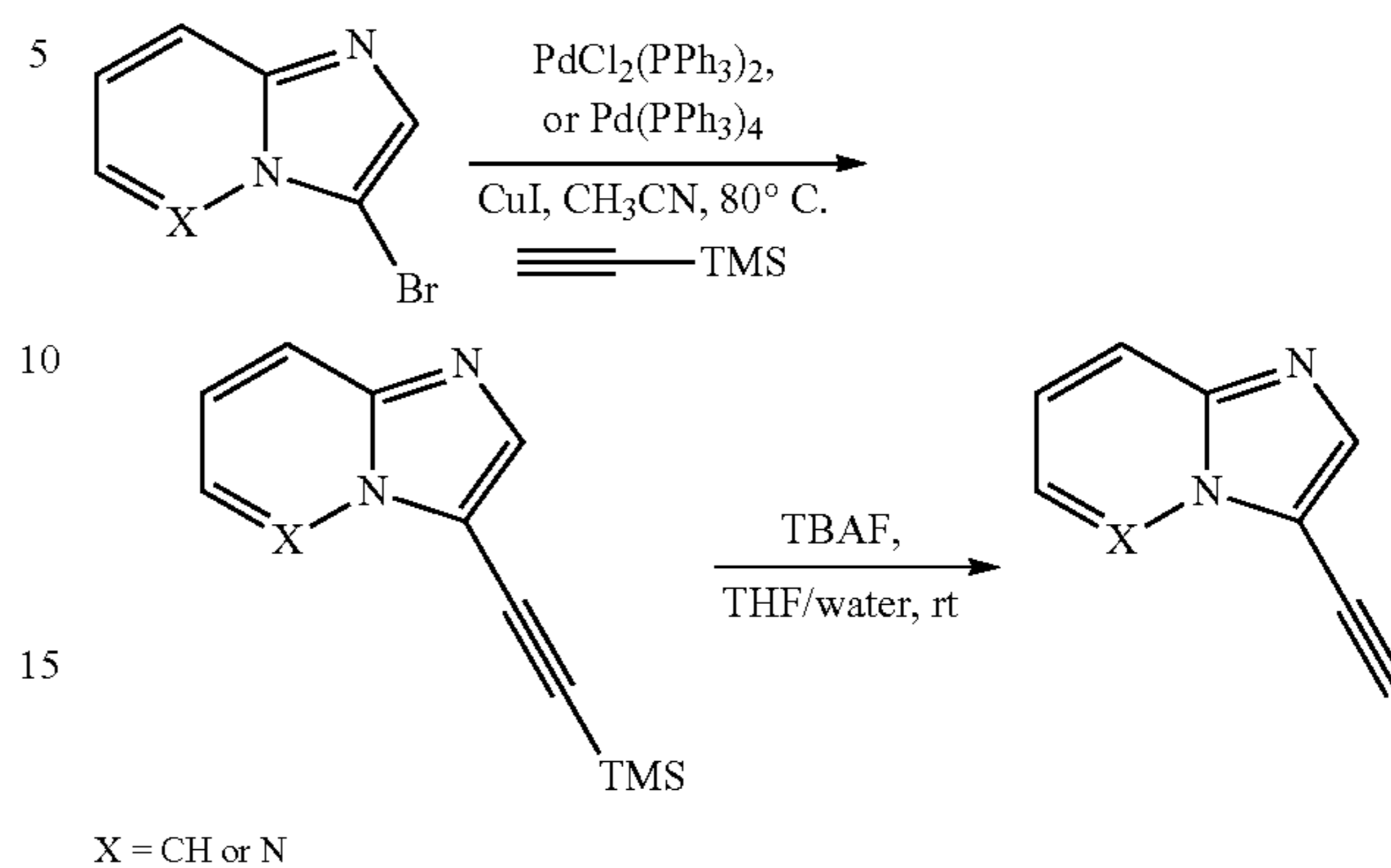
Scheme V: Preparation of 3-Ethynylimidazo[1,2-a]pyridine or 3-Ethynylimidazo[1,2-b]pyridazine
