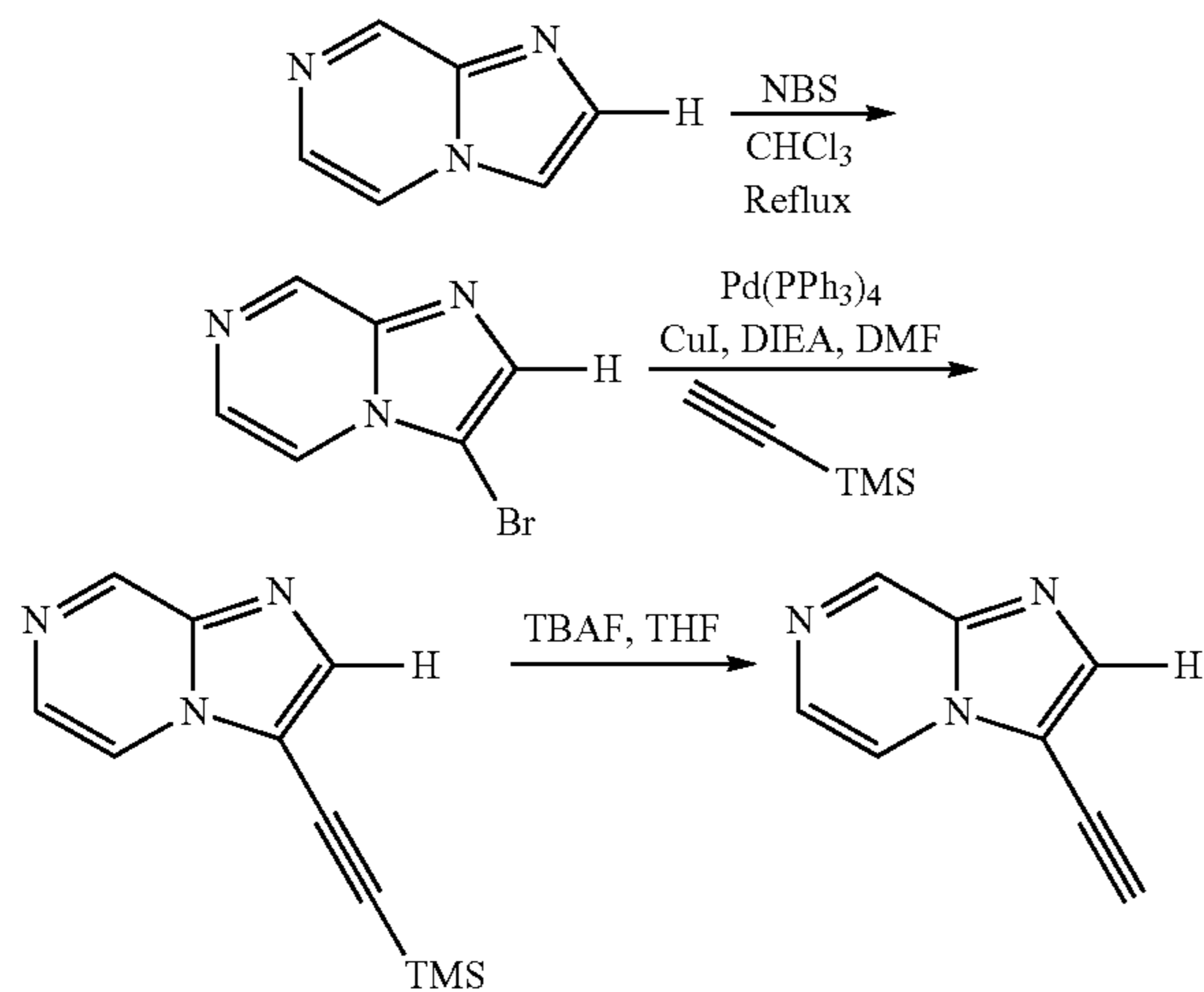
Scheme IV: Preparation of C-8 Substituted 3-Ethynylimidazo[1,2-a]pyrazines
