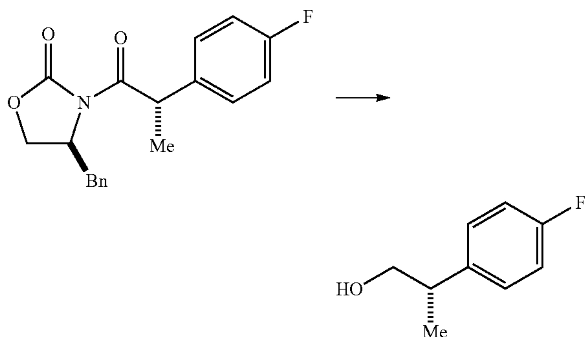
(S)-2-(4-Fluorophenyl)propan-1-ol
