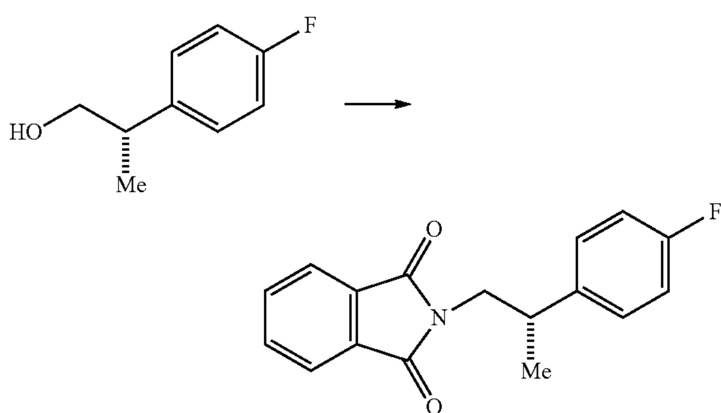
(S)-2-(2-(4-Fluorophenyl)propyl)isoindoline-1,3-dione
