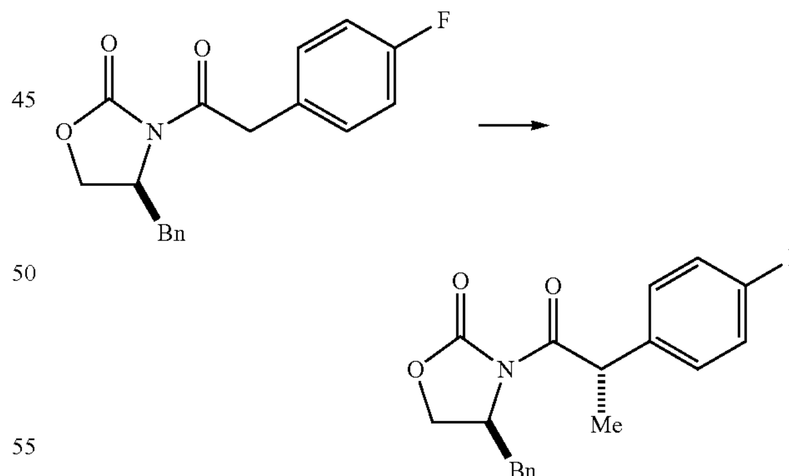
(S)-4-Benzyl-3-((S)-2-(4-fluorophenyl)propanoyl)oxazolidin-2-one
