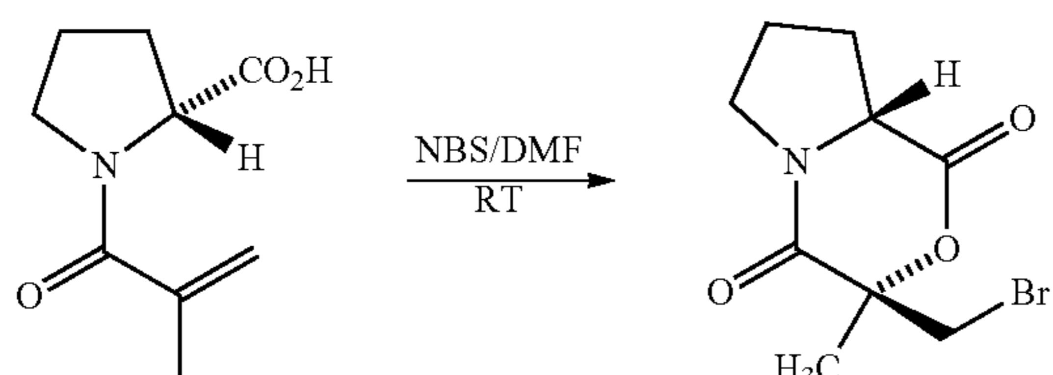
(3R,8aR)-3-Bromomethyl-3-methyl-tetrahydro-pyrrolo[2,1-c][1,4]oxazine-1,4-dione
