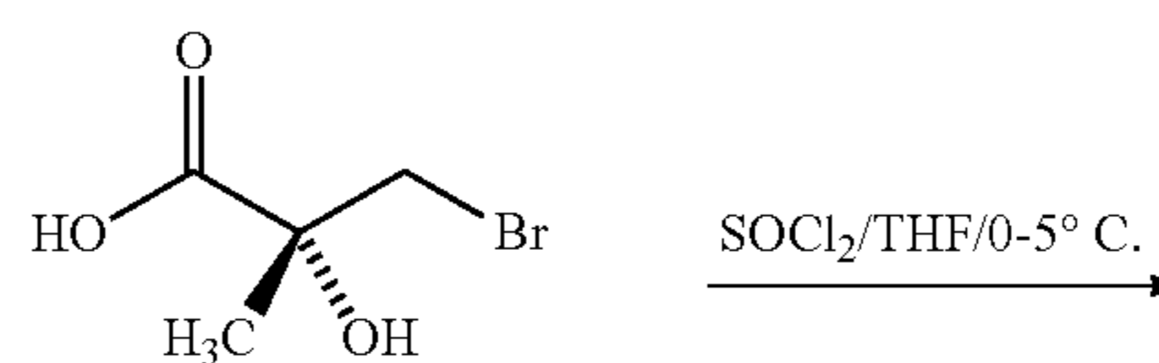
(R)-3-bromo-2-hydroxy-2-methylpropanoic acid
