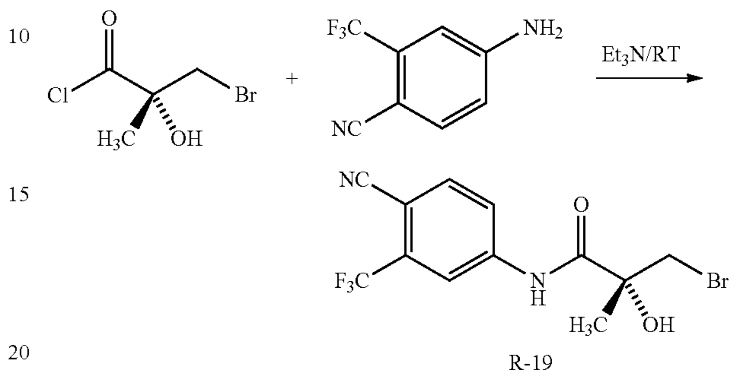
(R)-3-bromo-2-hydroxy-2-methylpropanoic acid
