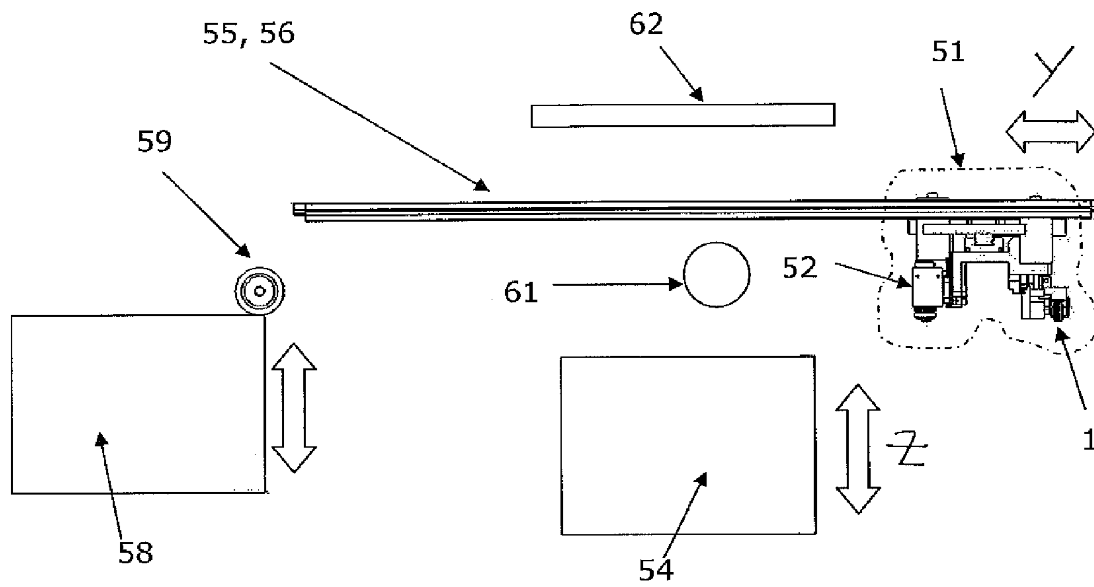
Figure 7: Basic Machine Layout: Front Elevation
