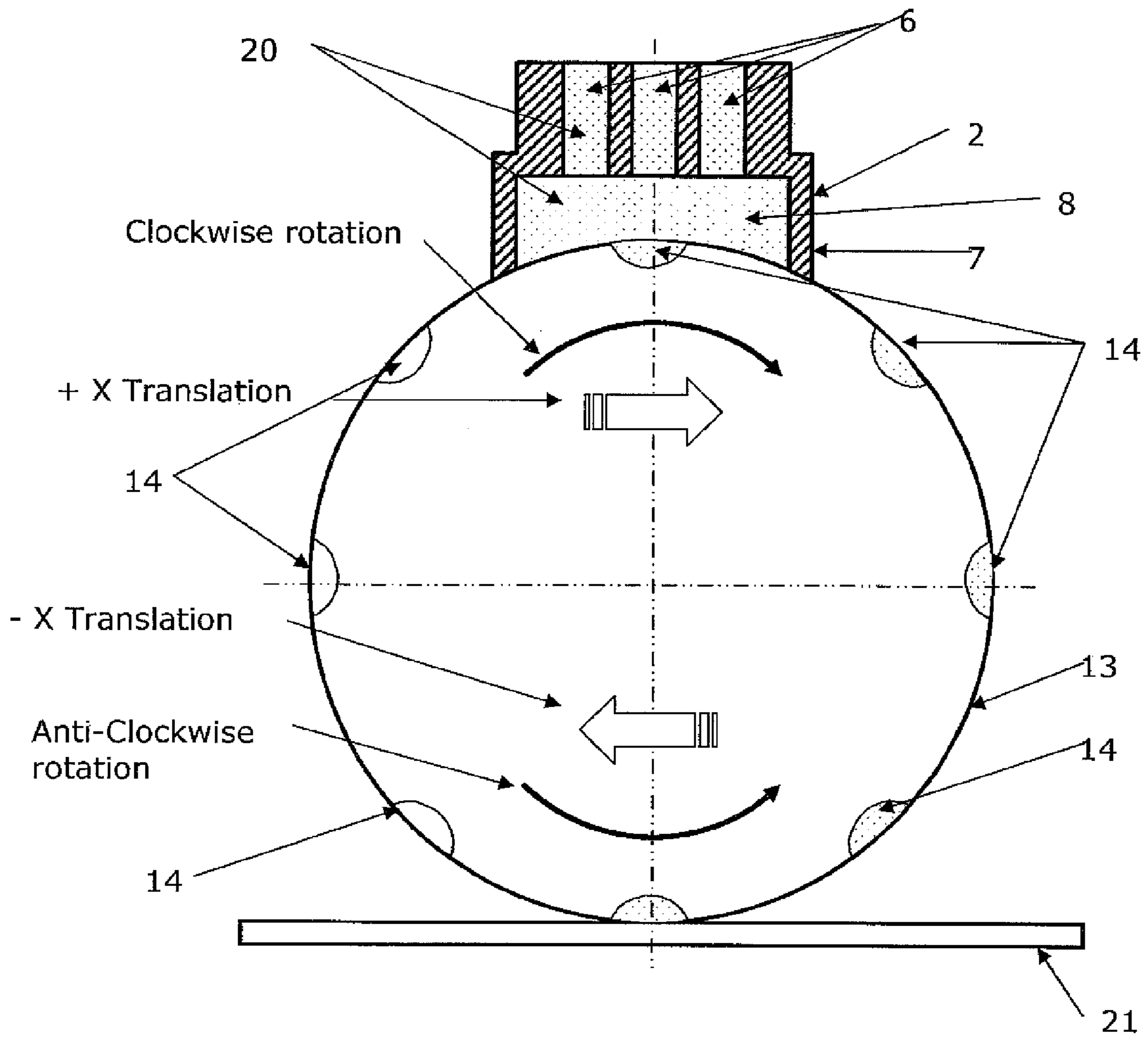
Figure 5: Priming of the adhesive wheel
