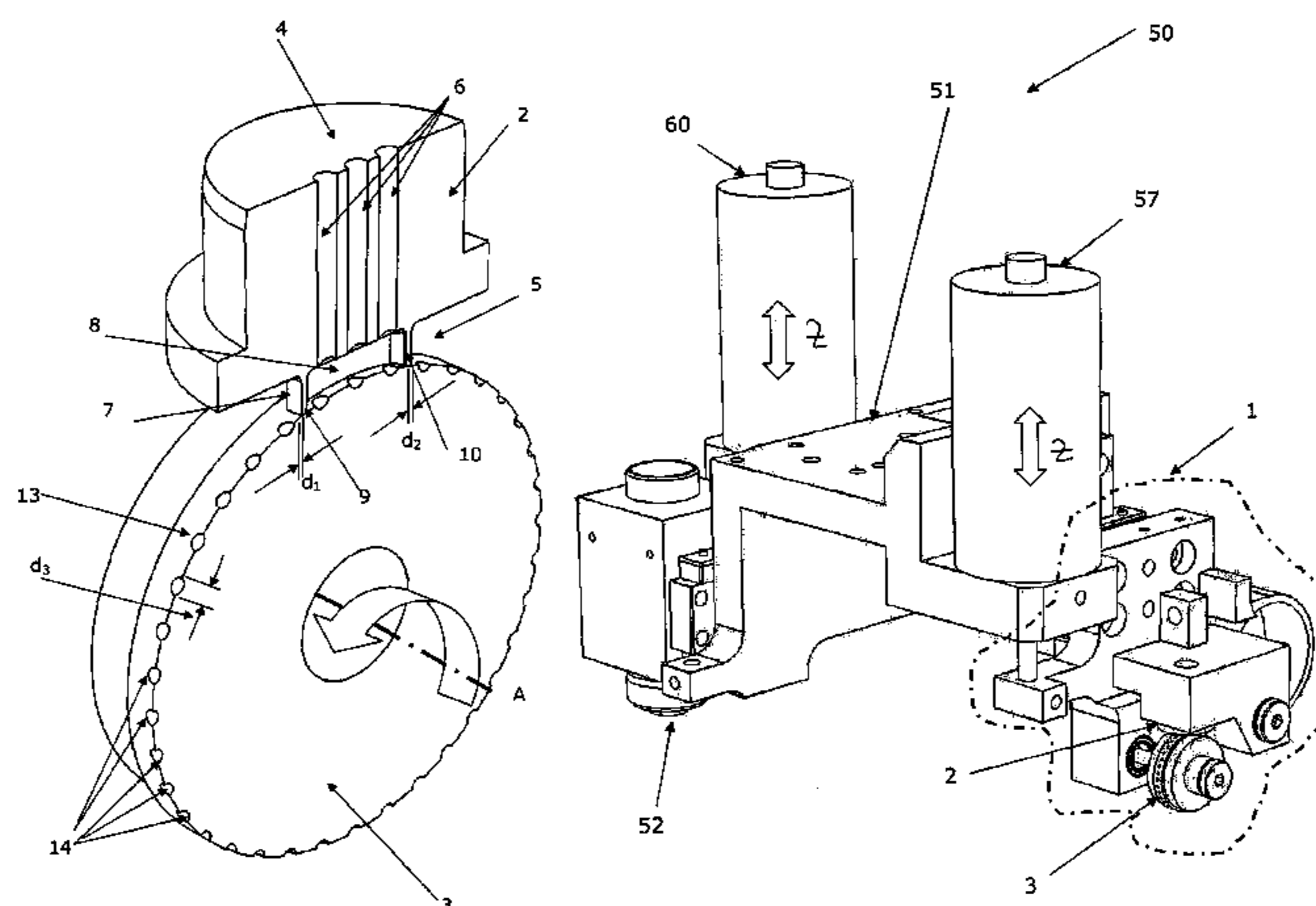
Isometric View of Multifunction Head
