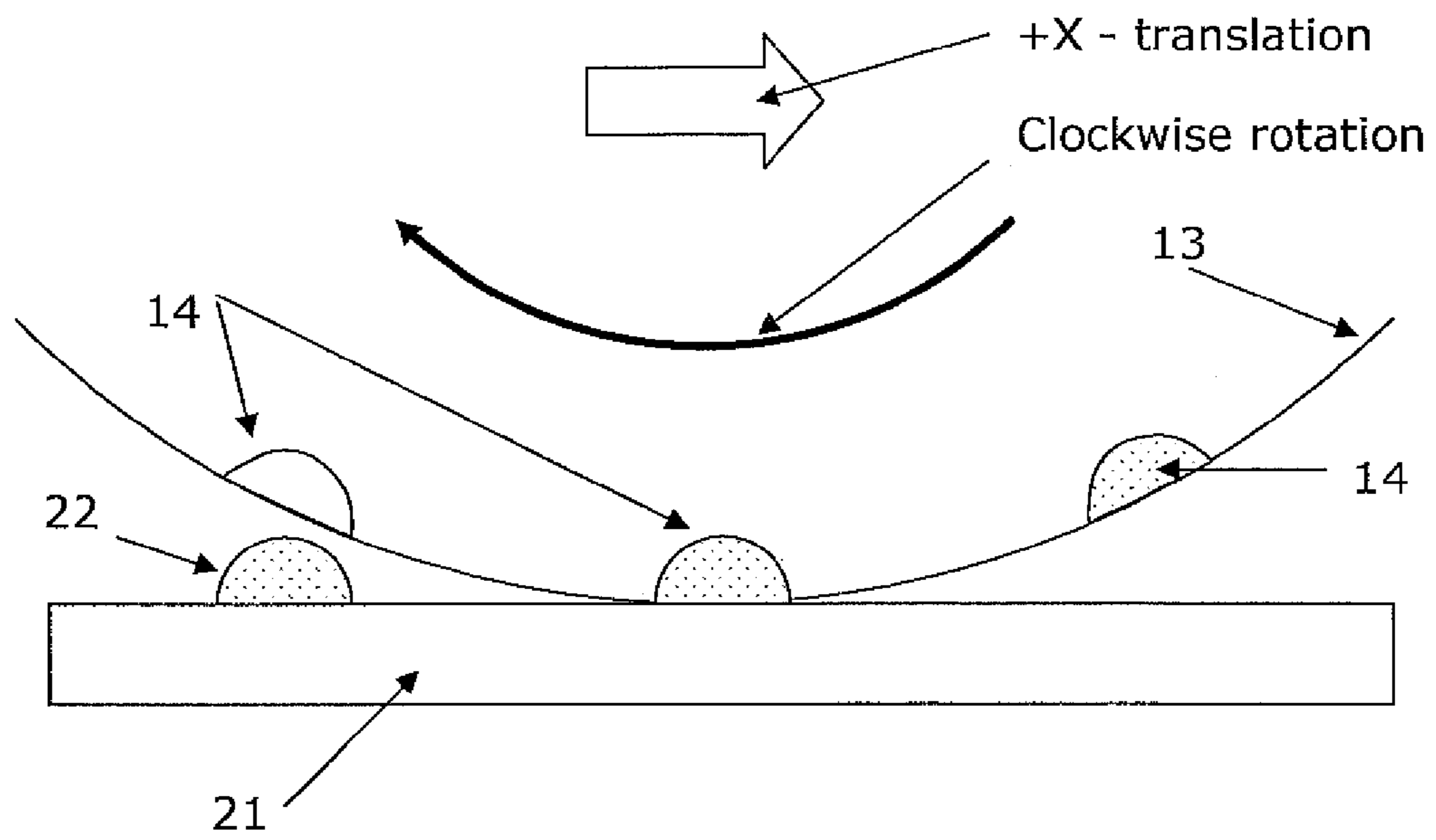
Figure 4: Schematic detailing the capillary action deposition method.
