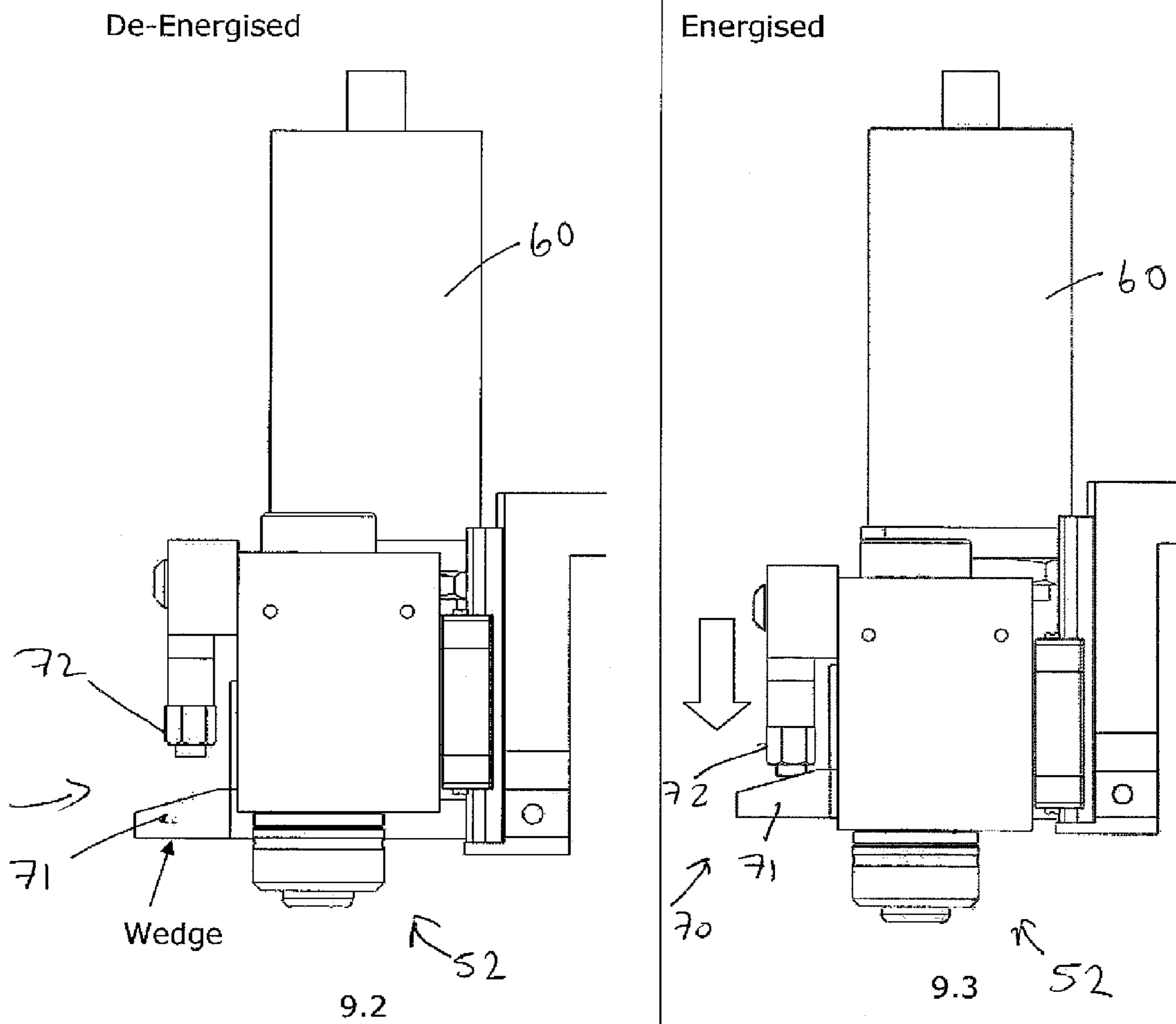
Figures 9.2 and 9.3: Grabber and wedge in a De-energised and Energised state
