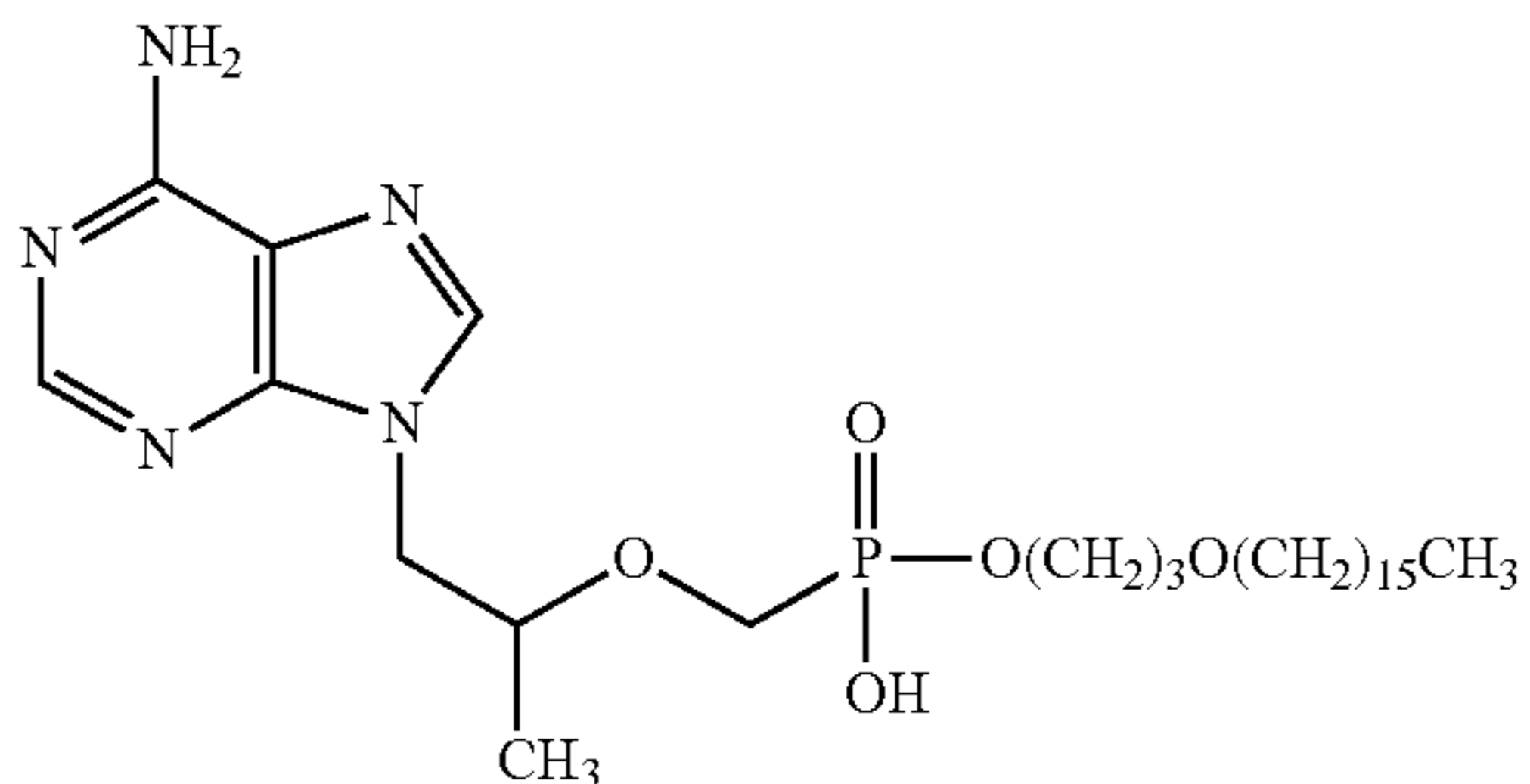
Compound 1
