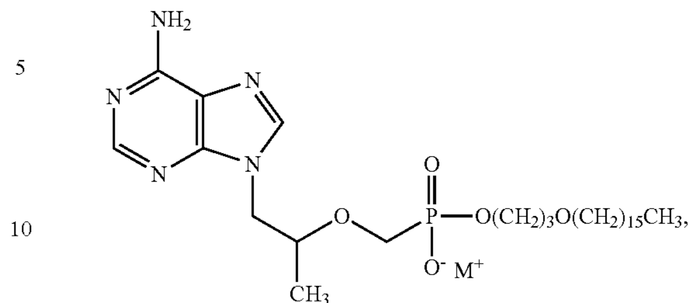
Formula I
