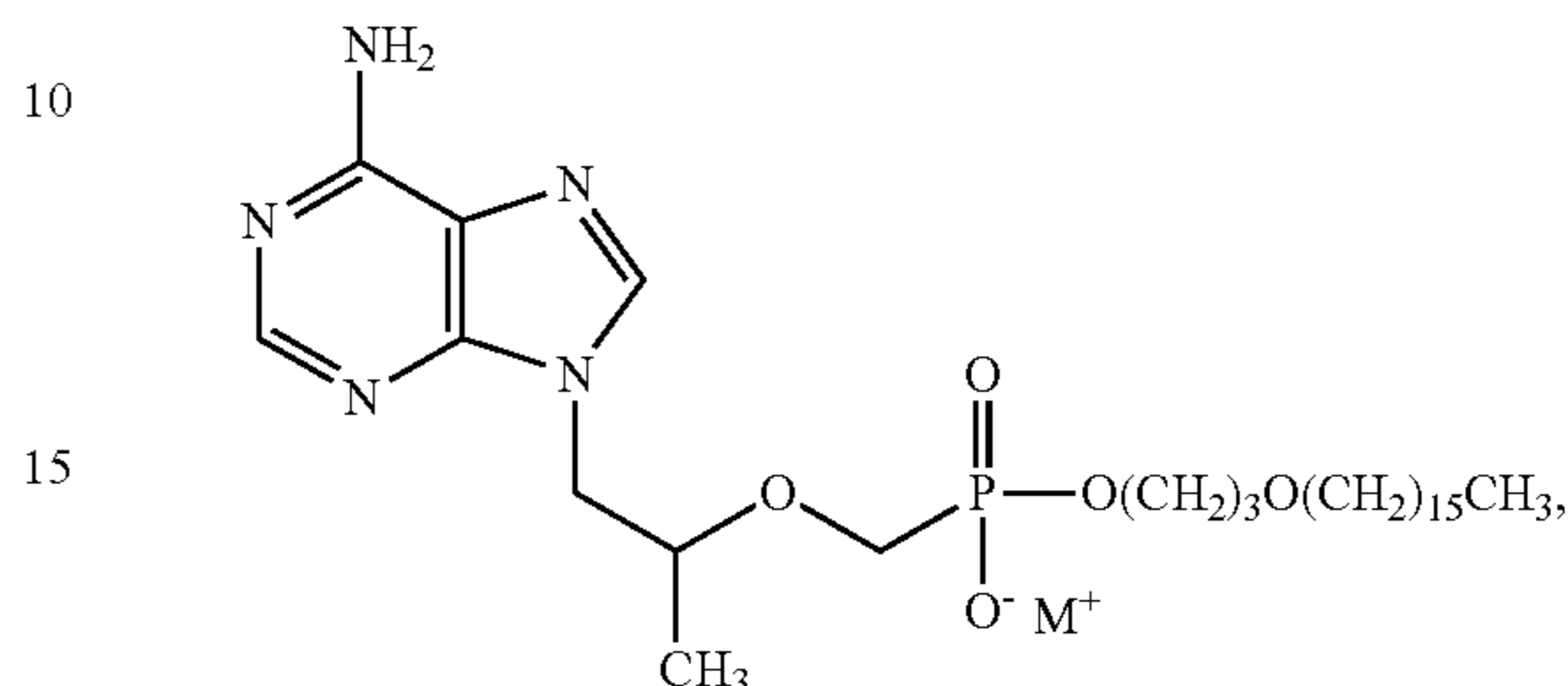
Formula I
