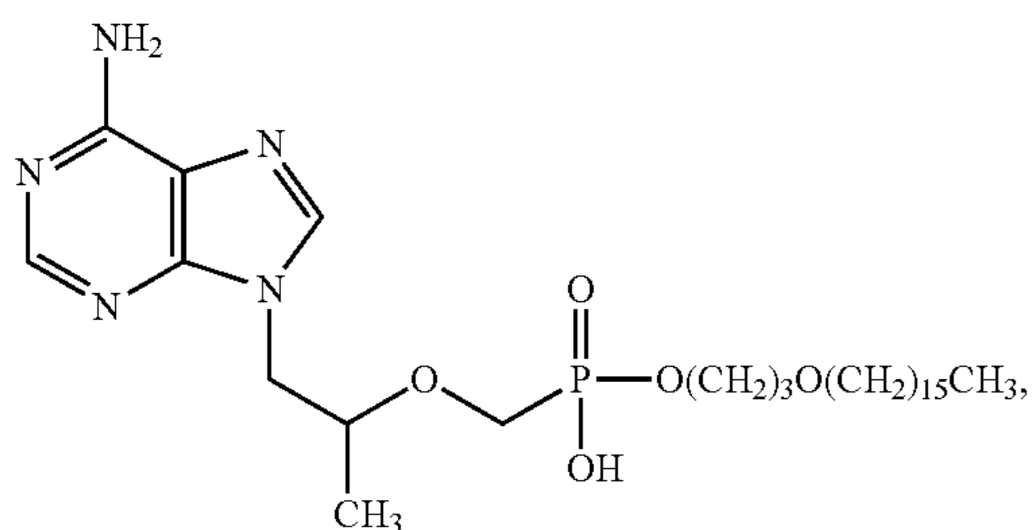
Compound I
