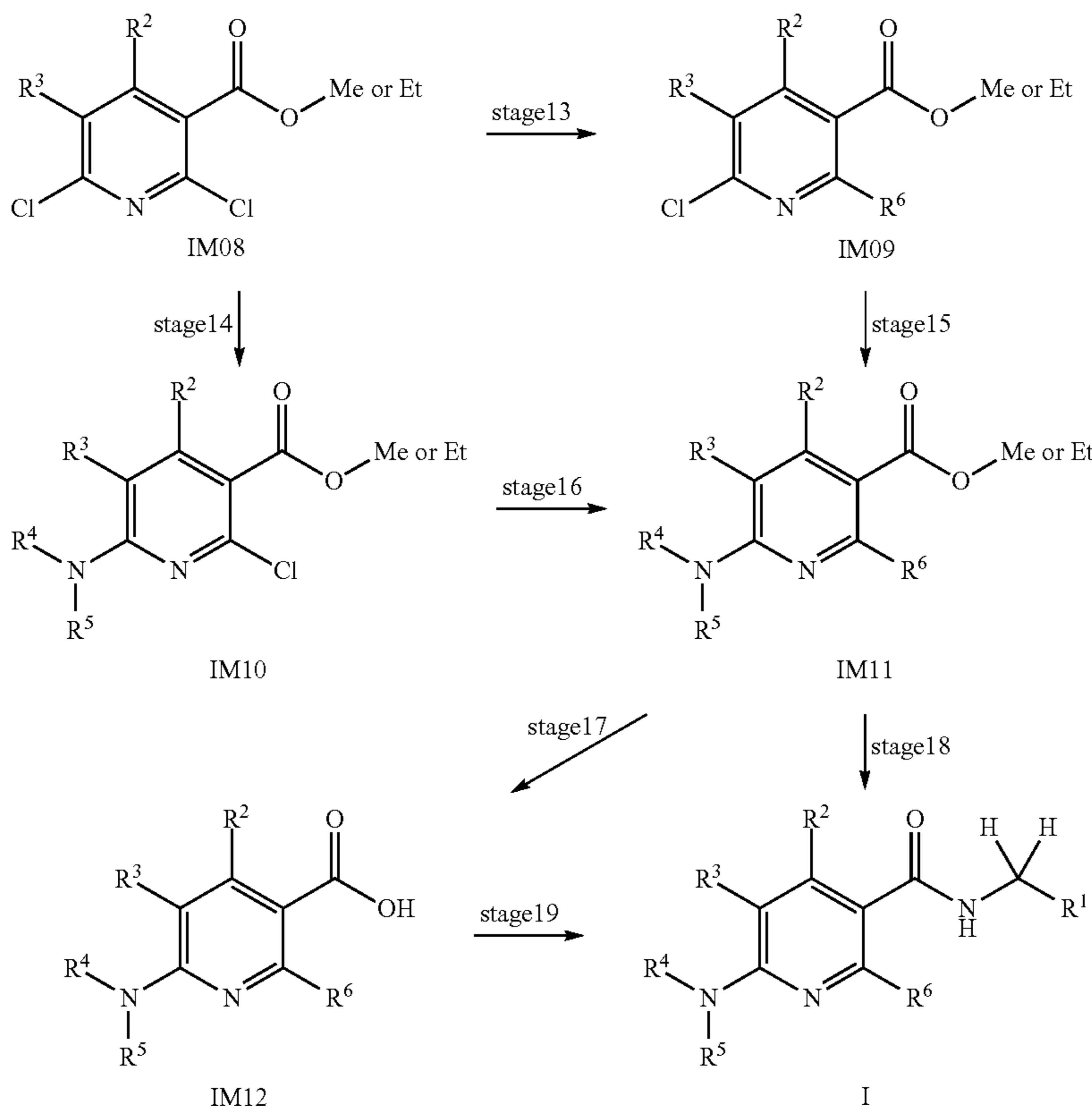
General reaction scheme III:
