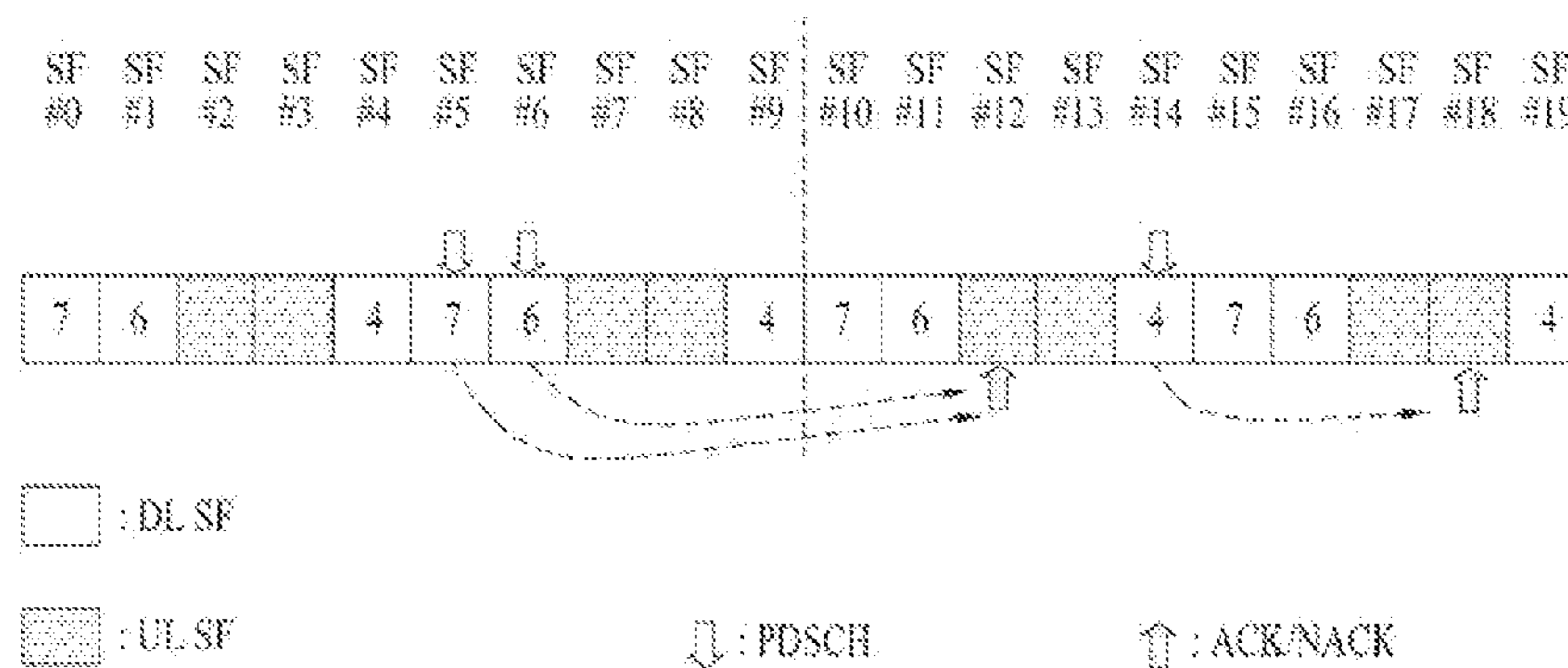
PDSCH-ACK/NACK timing (UL-DL configuration #1)
