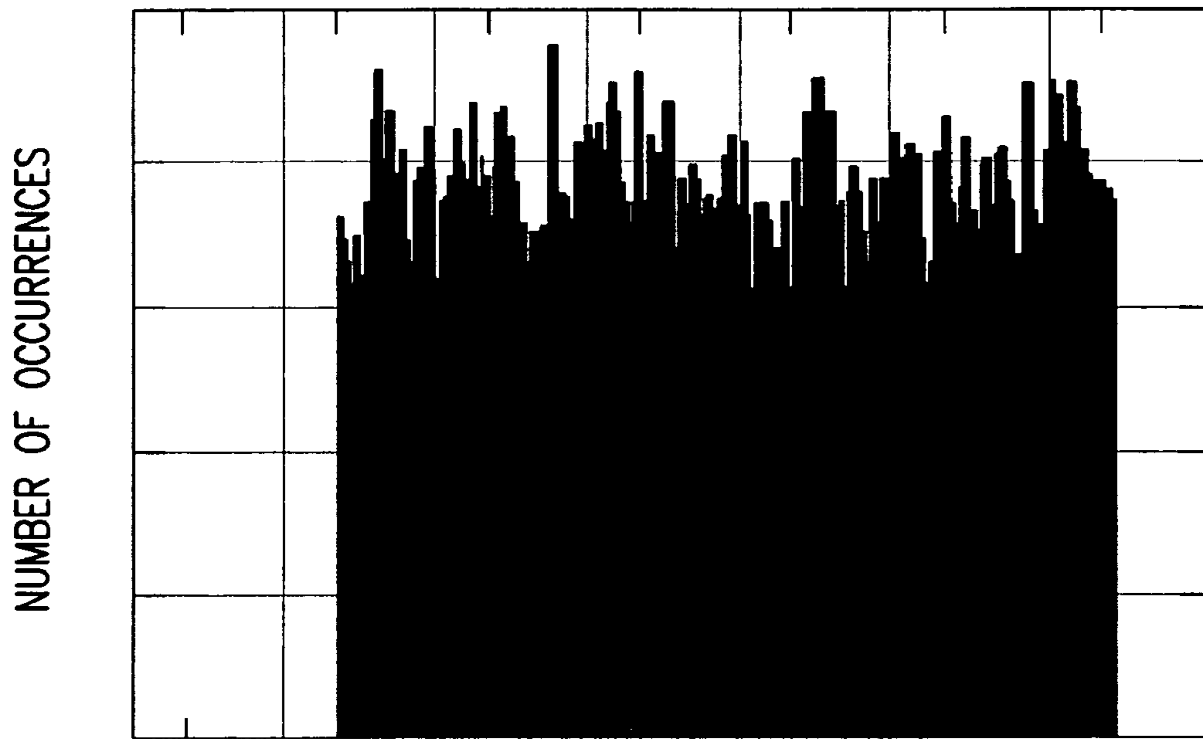
MODEL JPEG
