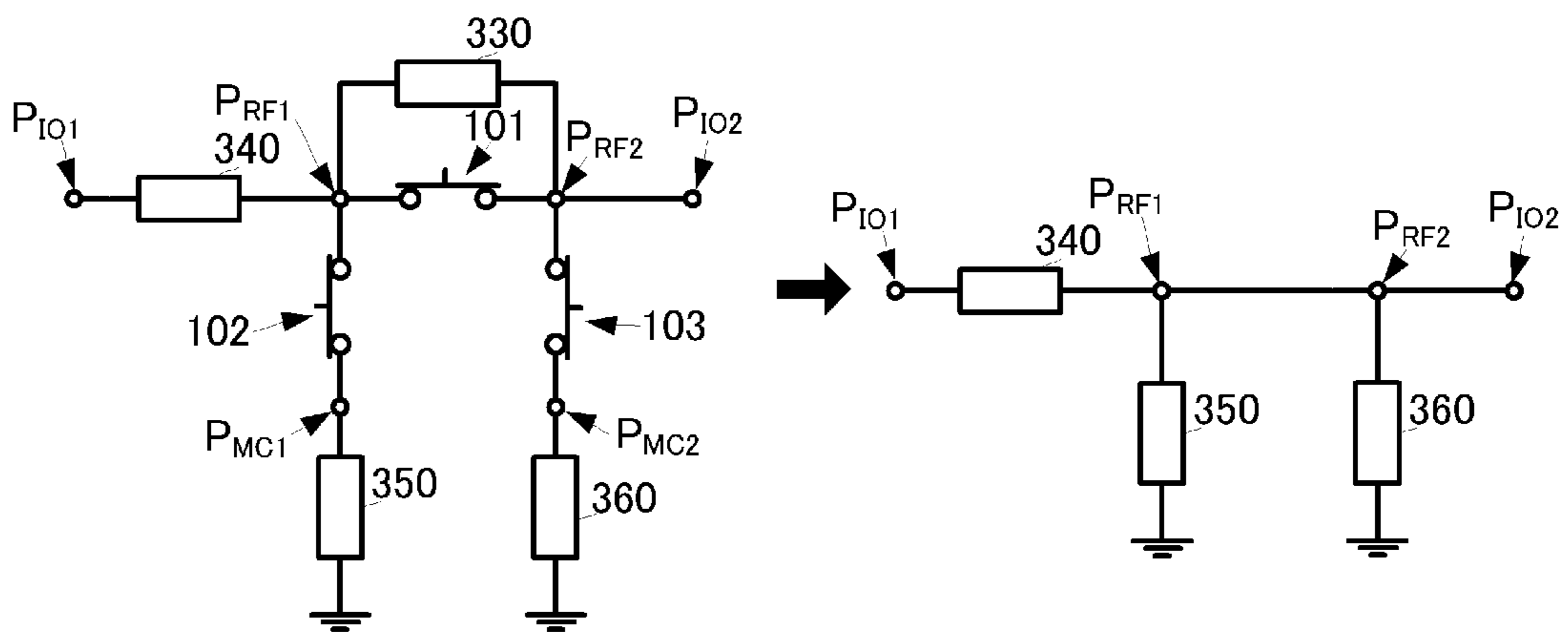
FIG. 5C 101:ON,102:ON,103:ON
