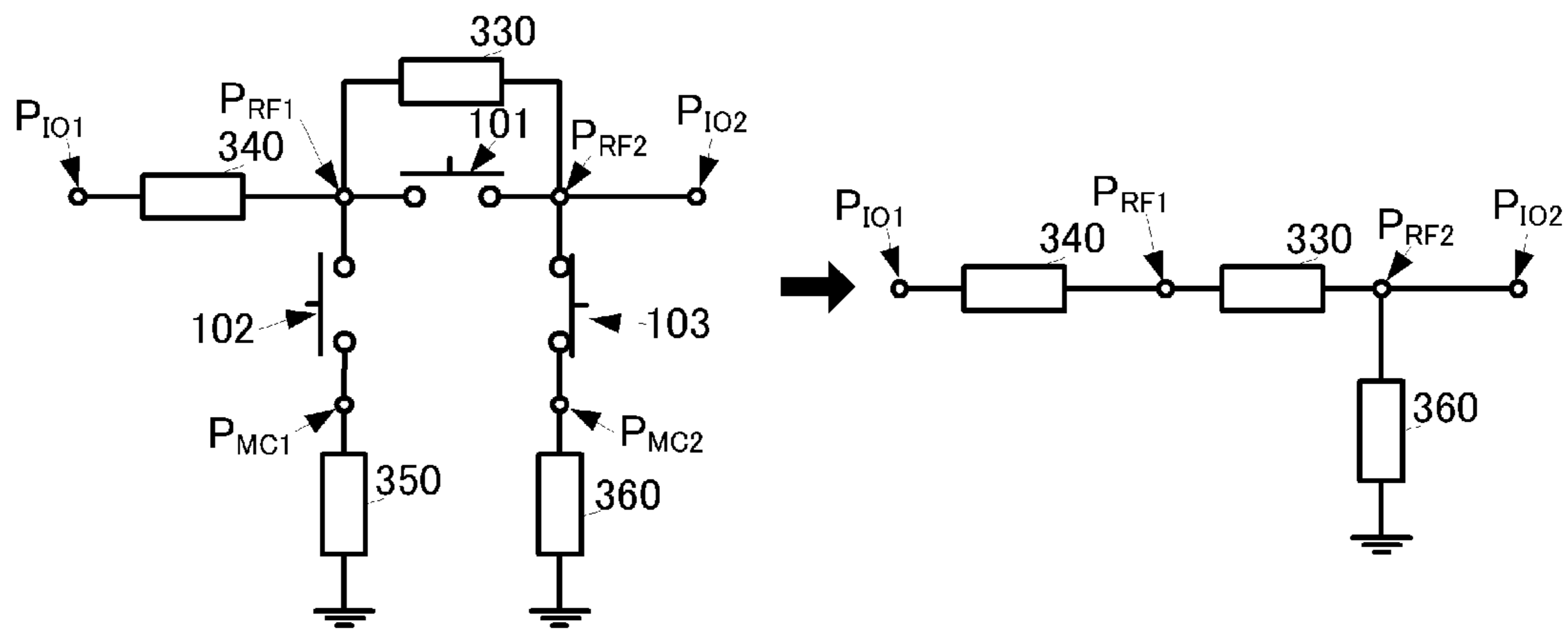
FIG. 7H 101:OFF,102:OFF,103:ON
