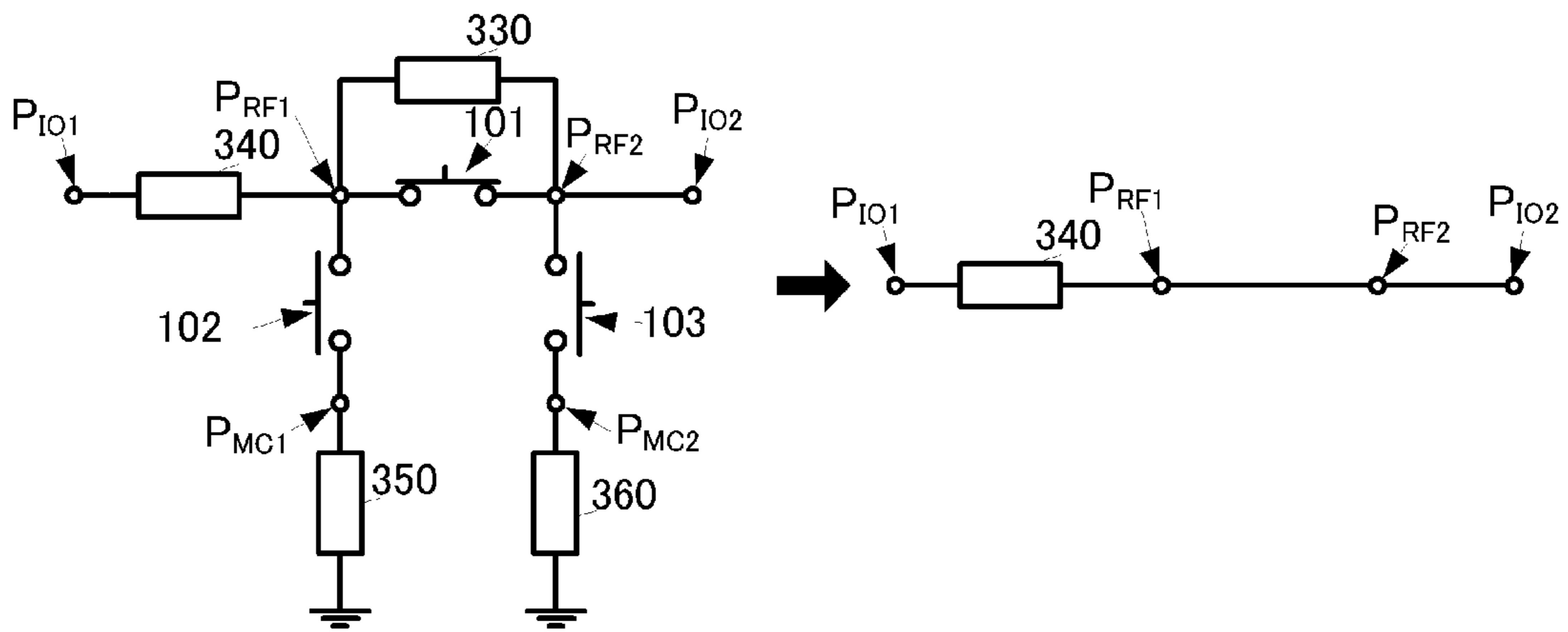
FIG. 5A 101:ON,102:OFF,103:OFF
