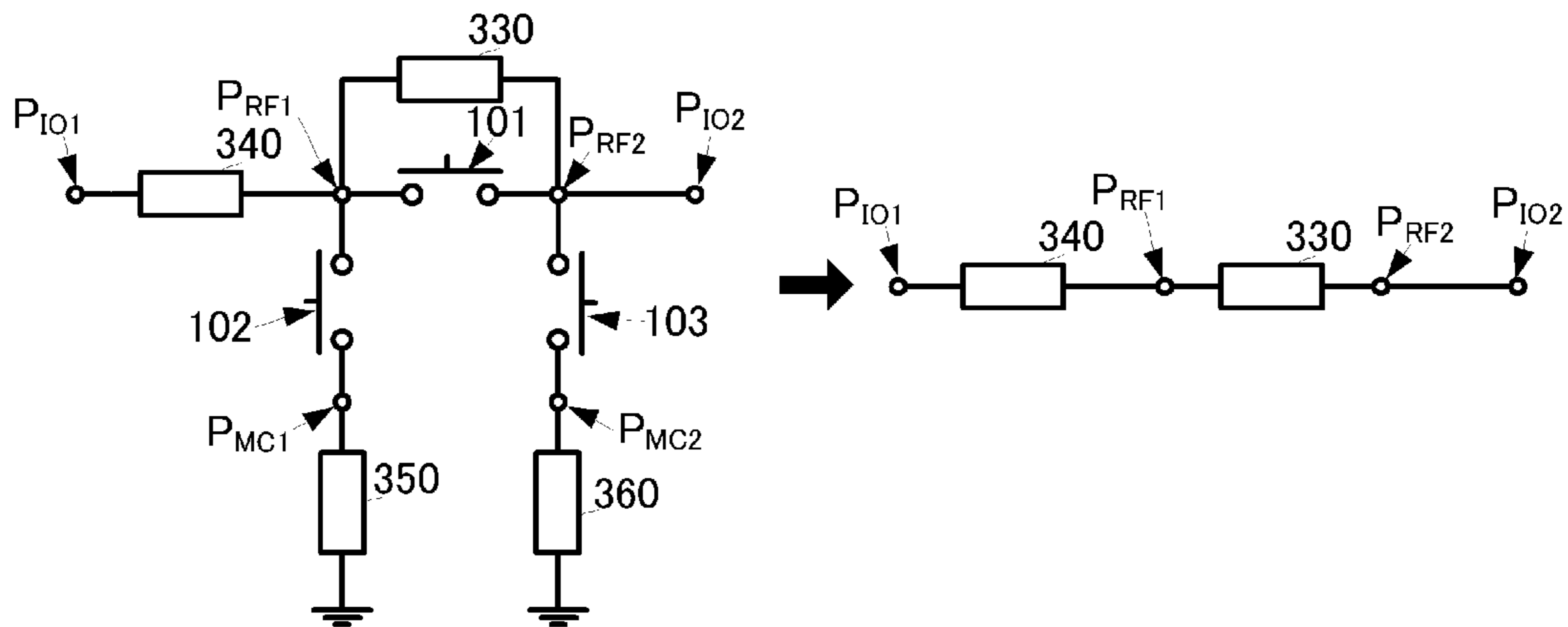
FIG. 6E 101:OFF,102:OFF,103:OFF
