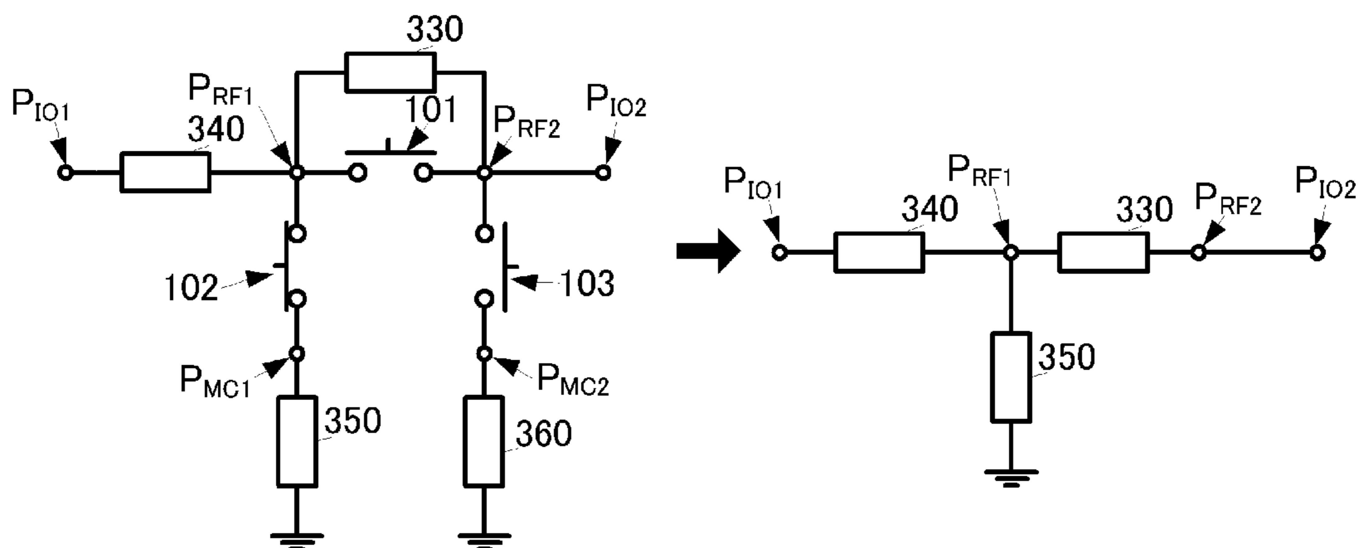
FIG. 6F 101:OFF,102:ON,103:OFF
