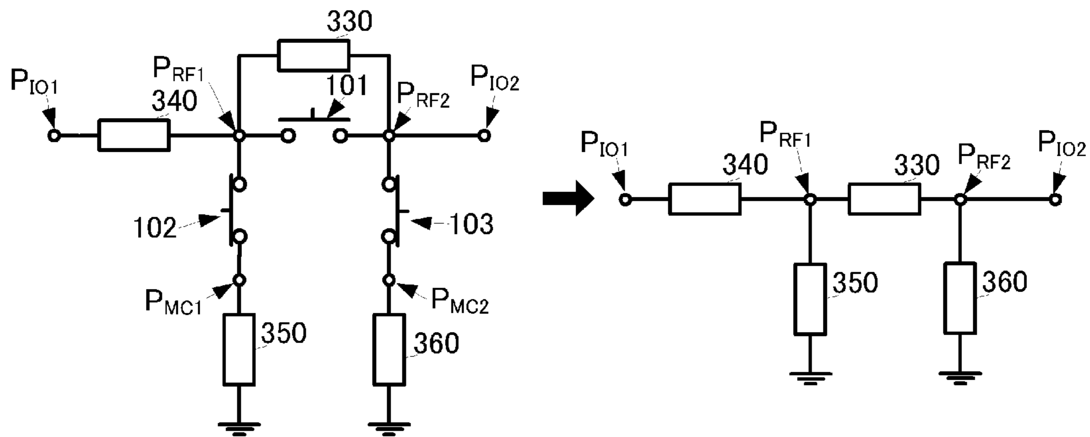
FIG. 7G 101:OFF,102:ON,103:ON
