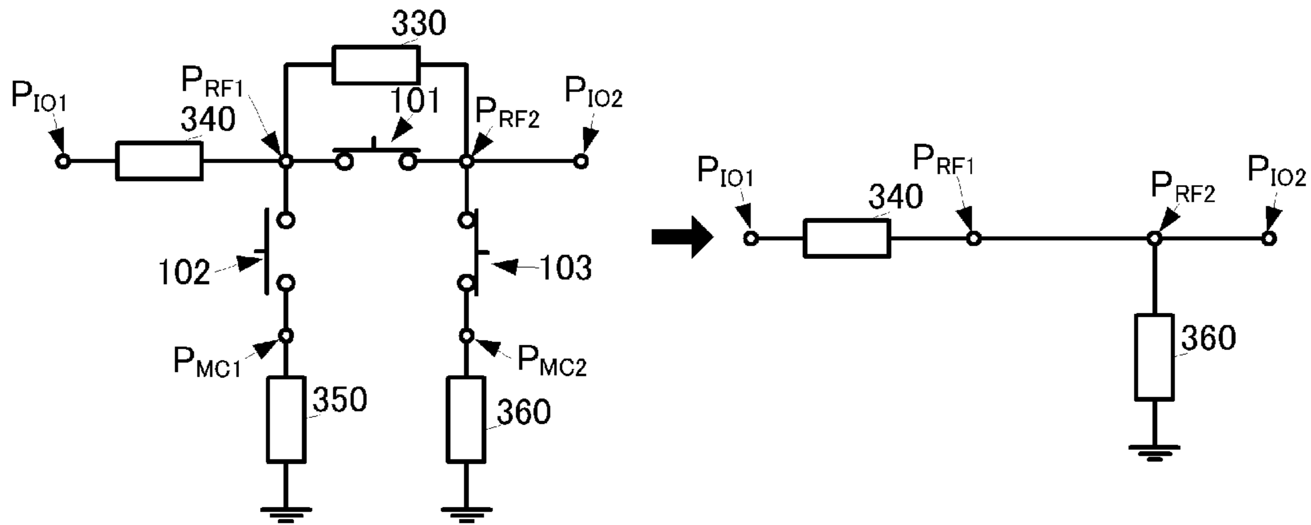
FIG. 6D 101:ON,102:OFF,103:ON
