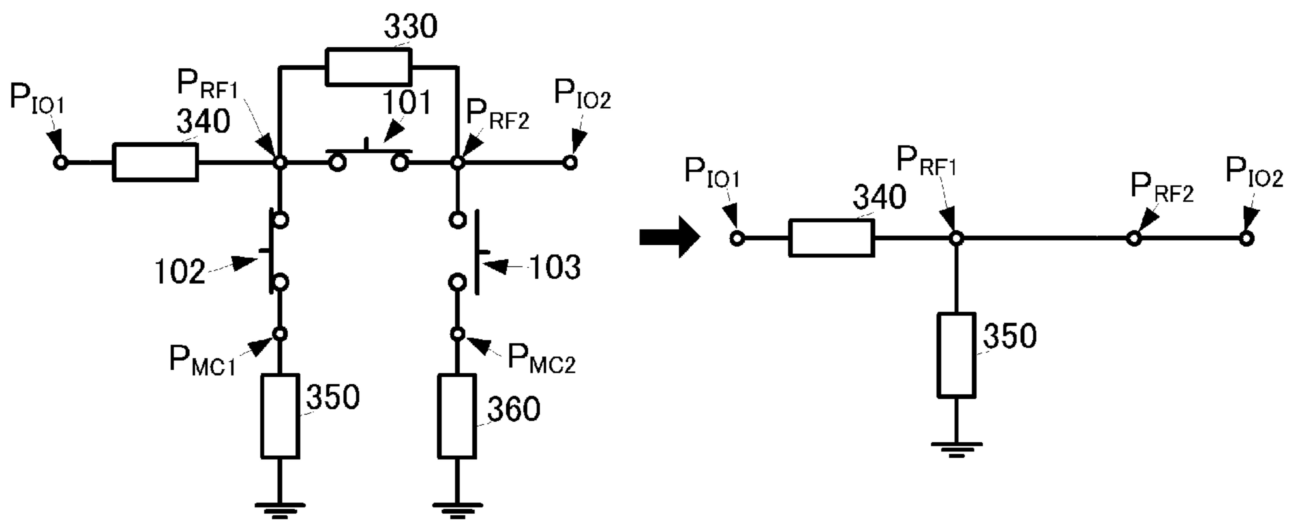
FIG. 5B 101:ON,102:ON,103:OFF
