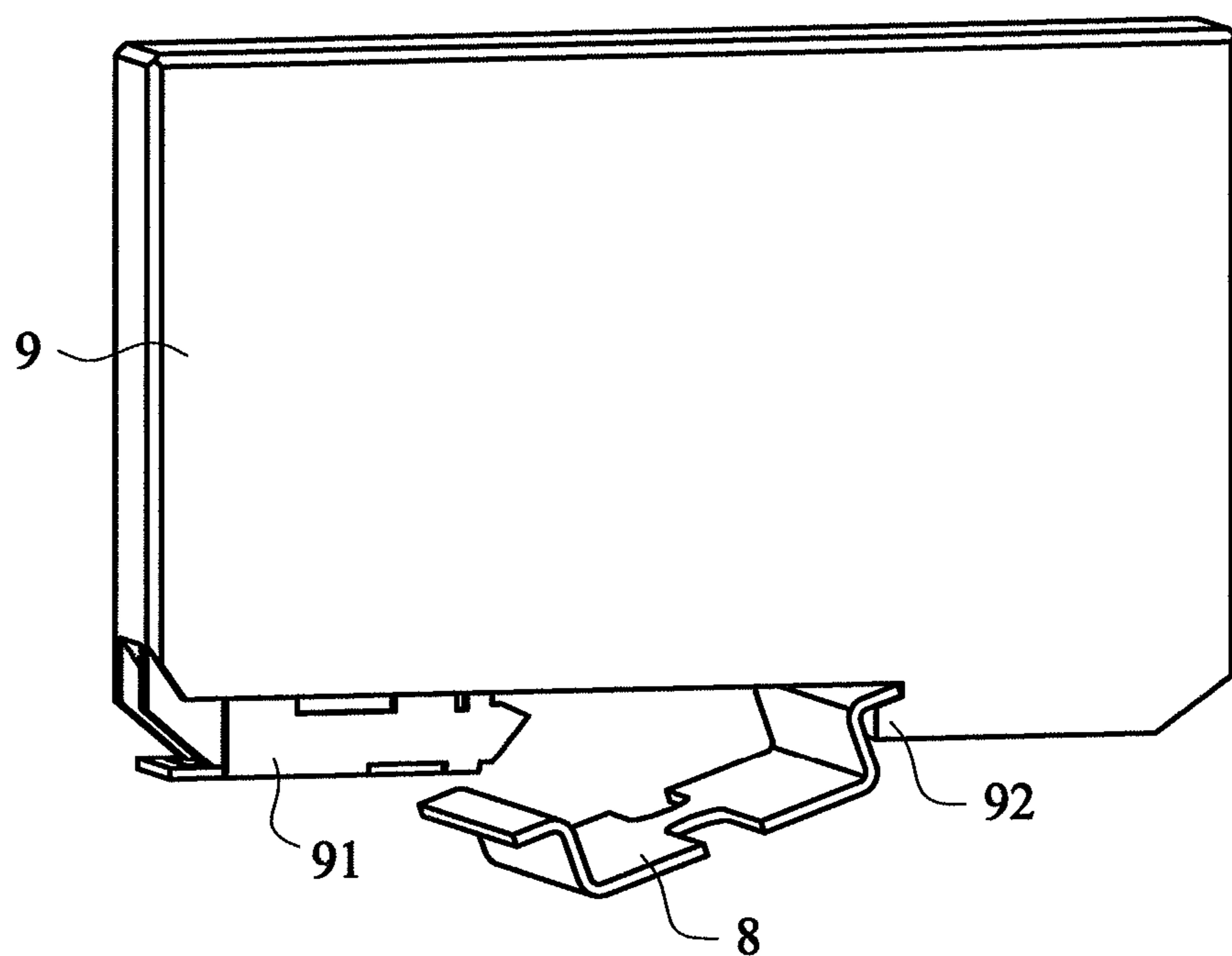
FIG. 3 (Prior Art)
