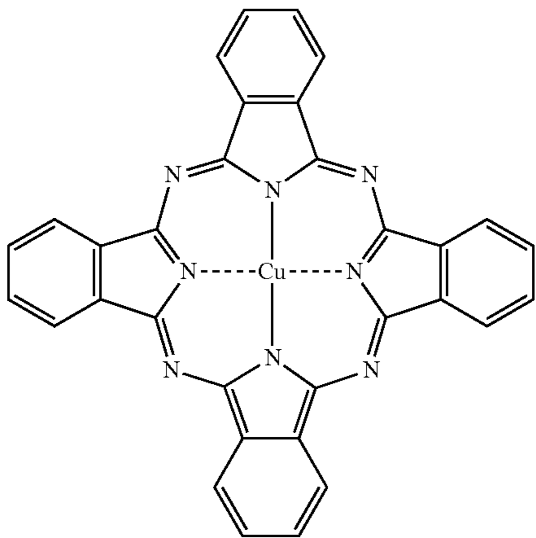
CuPc
