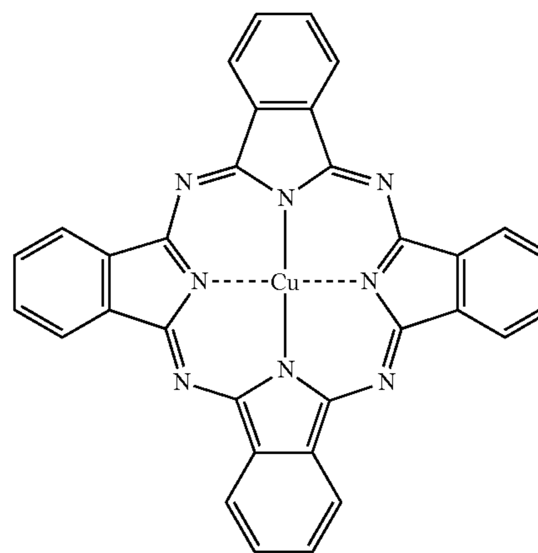
CuPc
