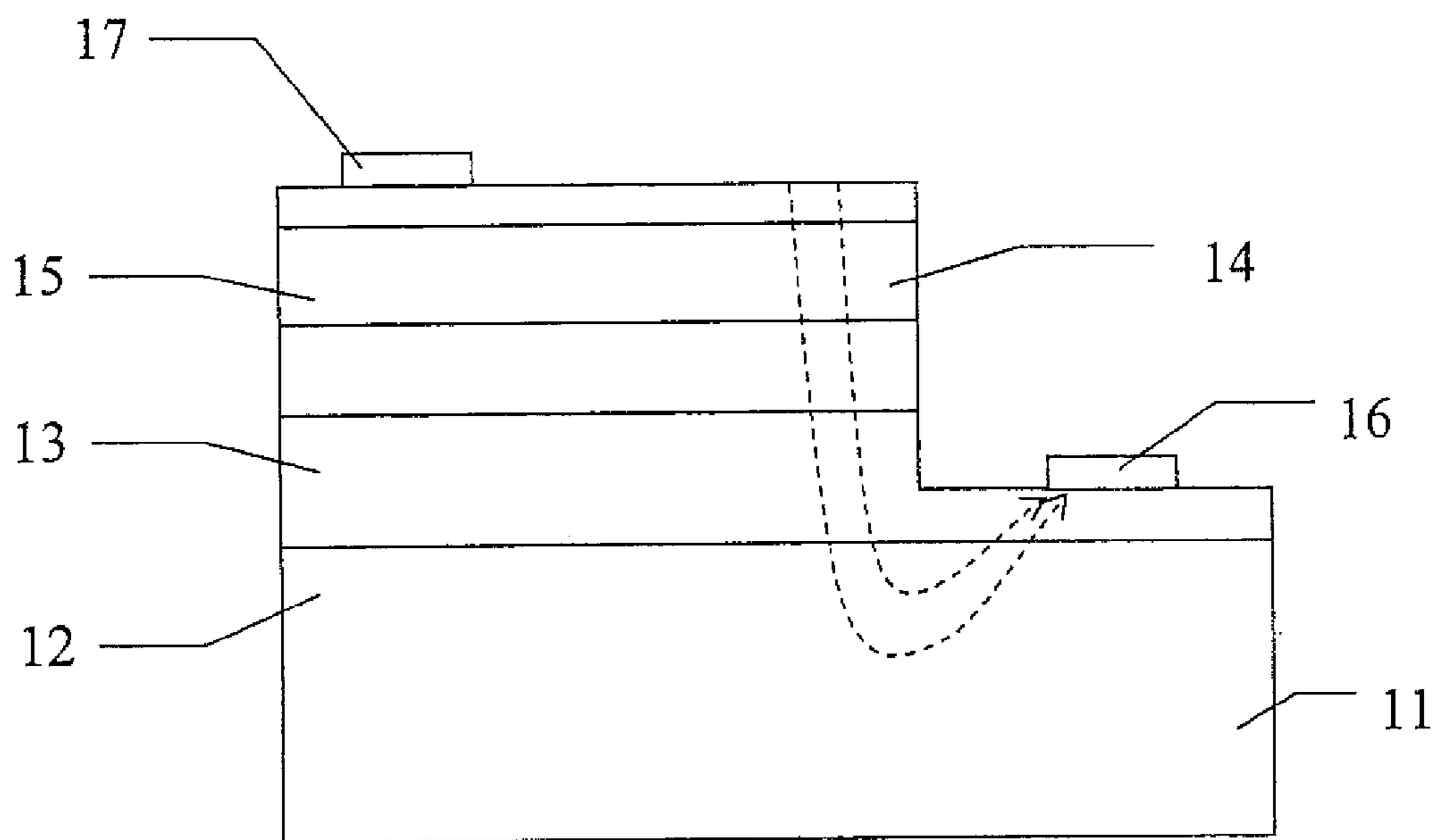
FIG. 1B (Conventional LED)
