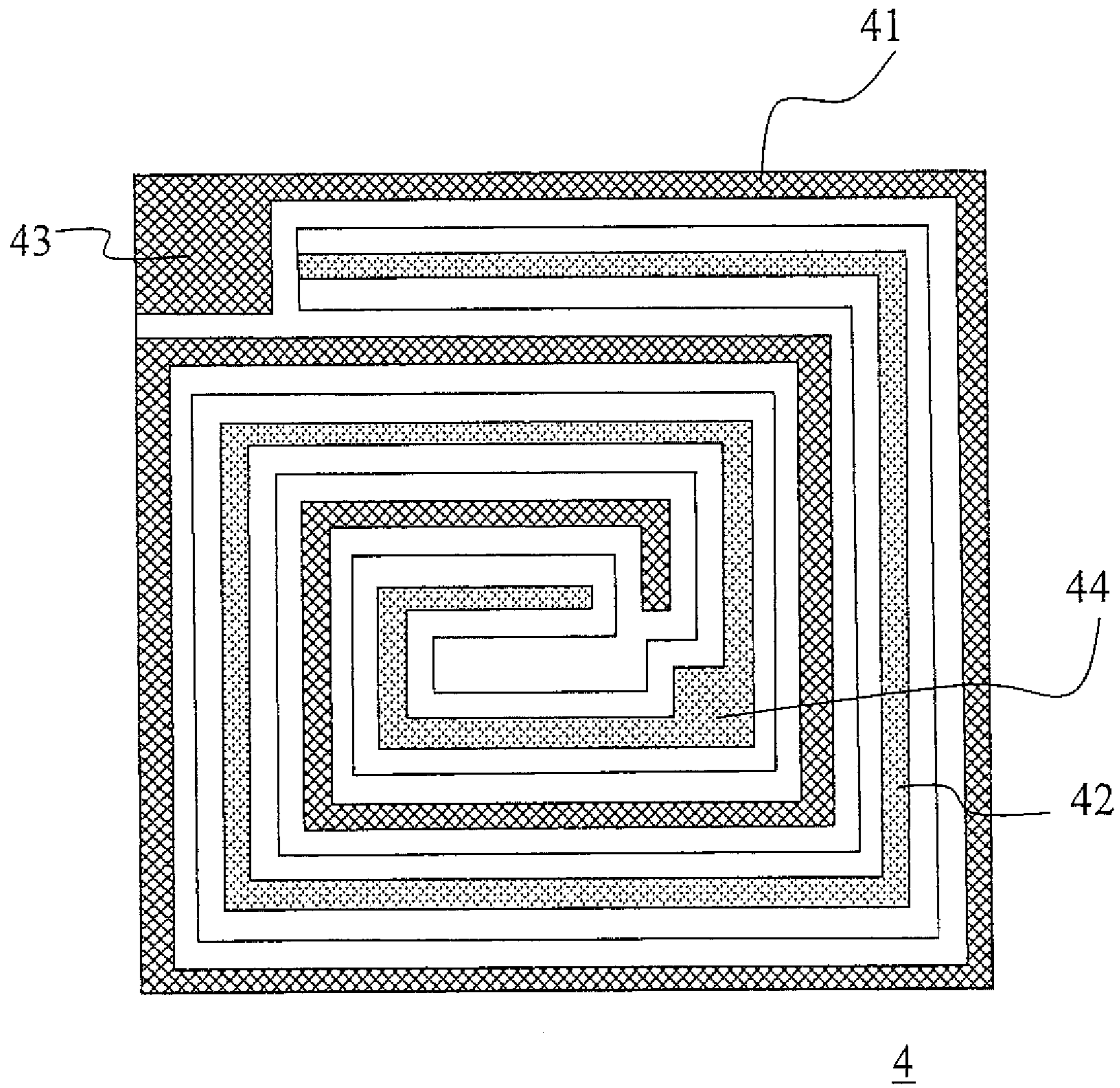
FIG.4 (Conventional LED)
