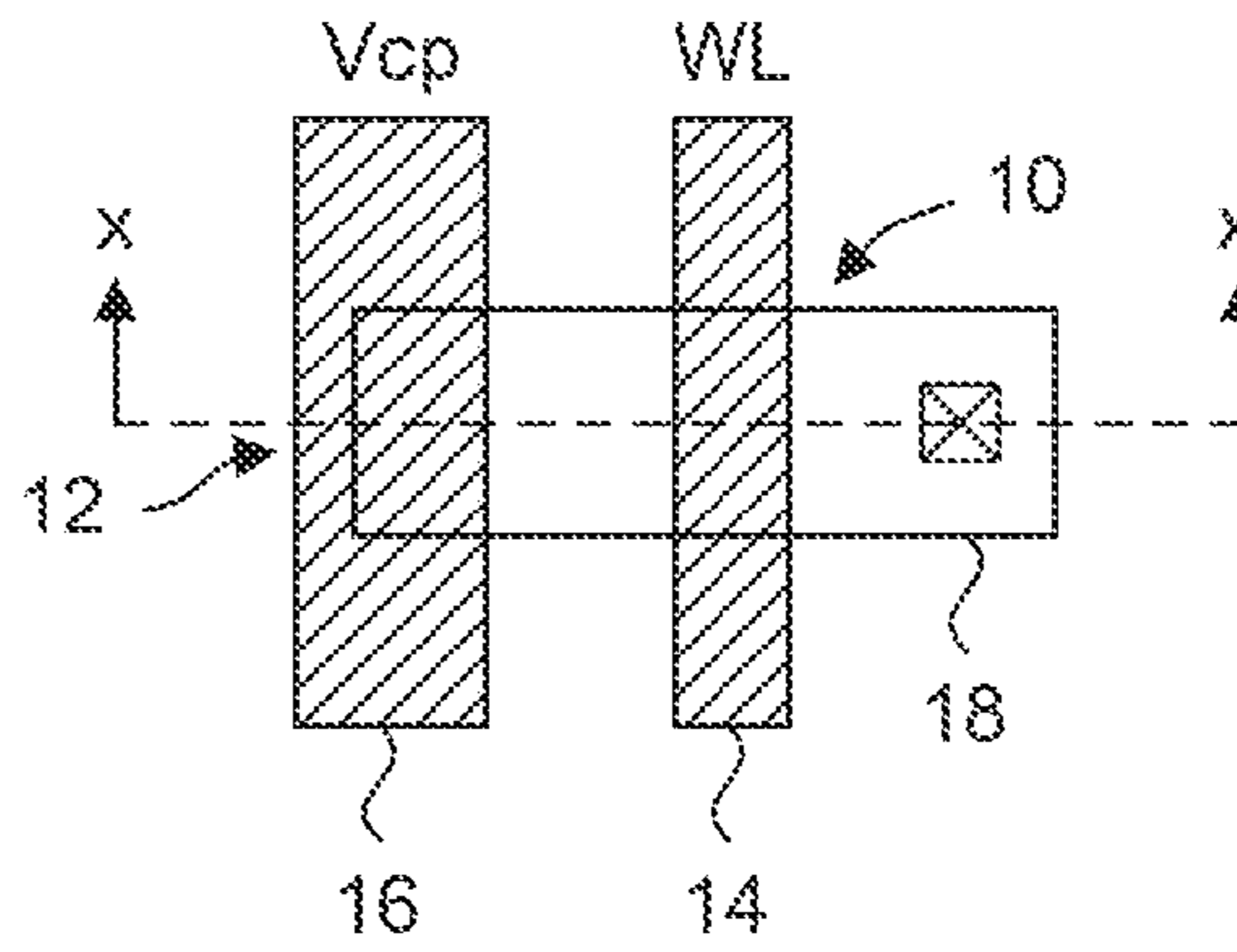
FIG. 2 (Prior Art)
