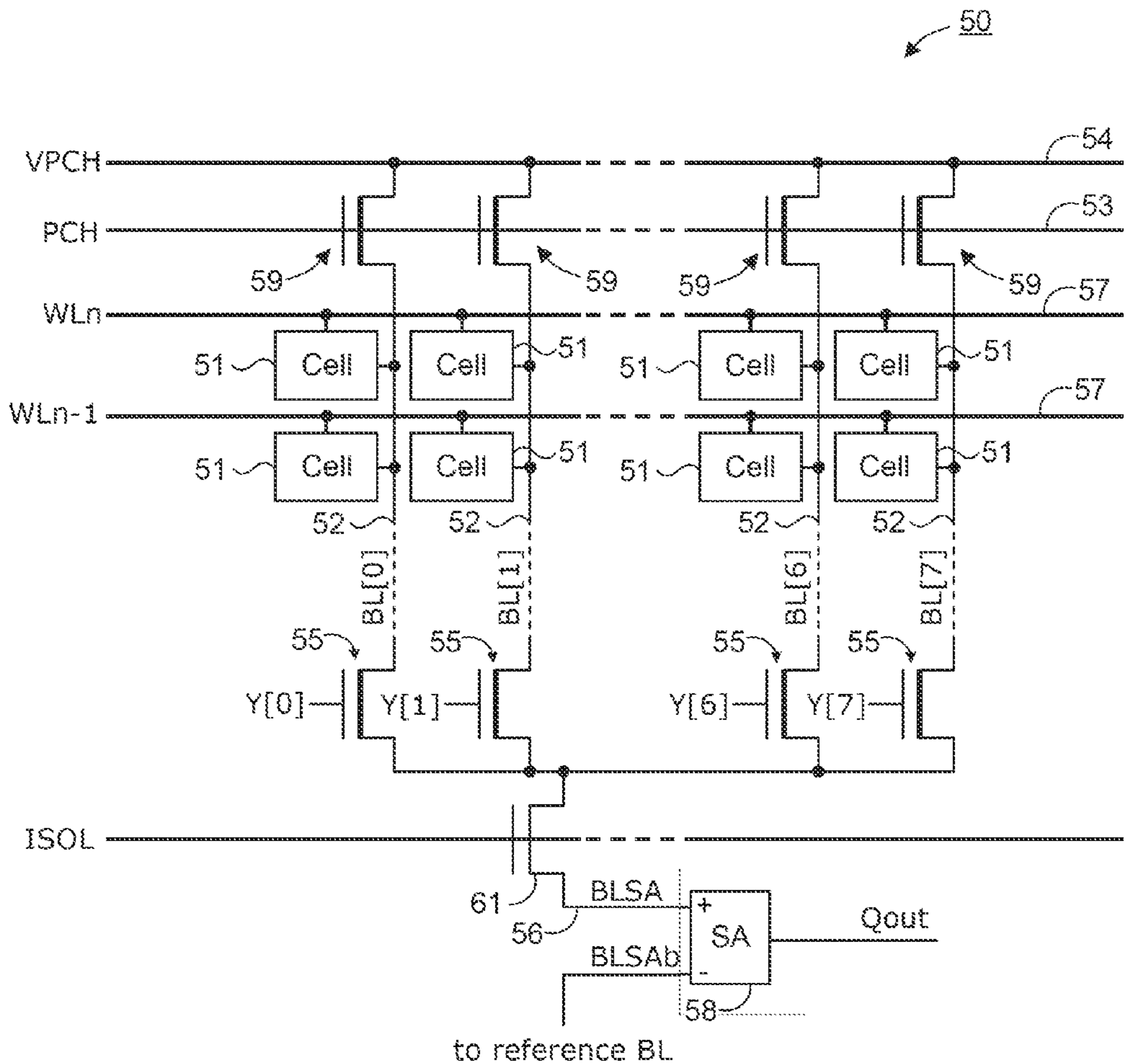
FIG. 5 (Prior Art)
