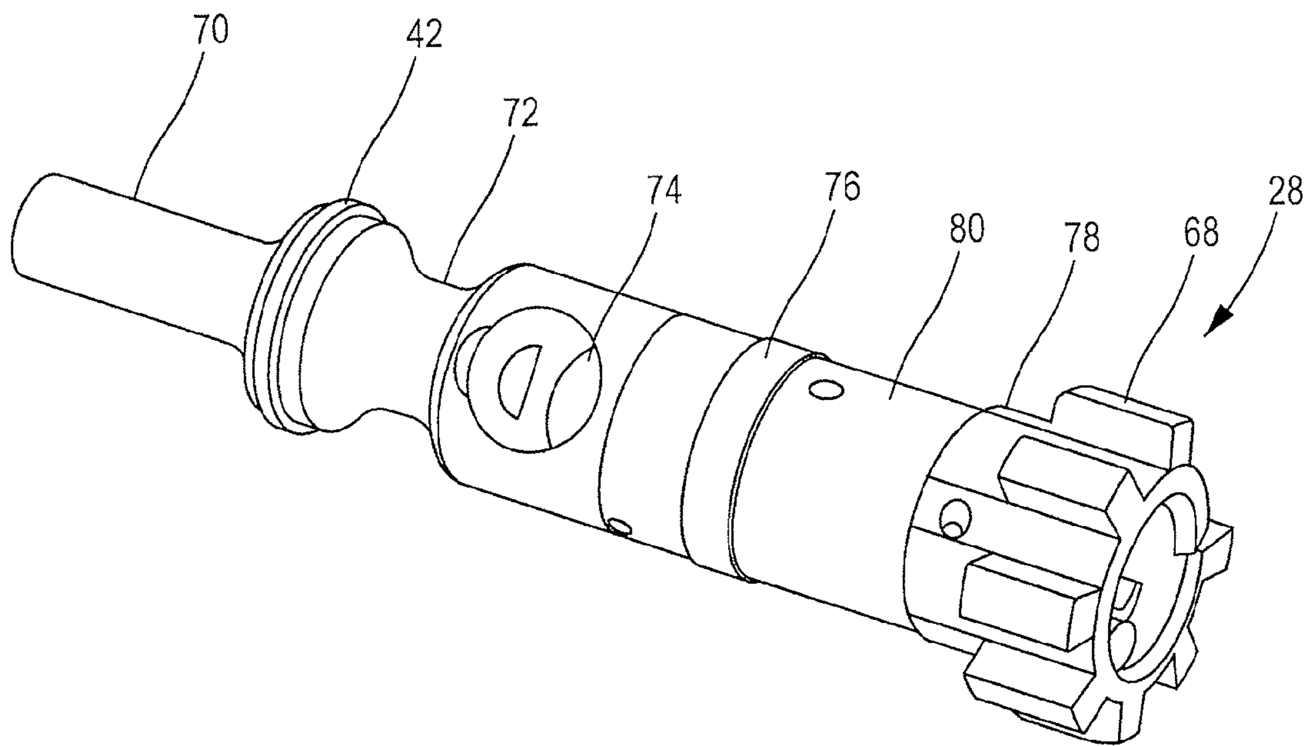
Fig.16 PRIOR ART
