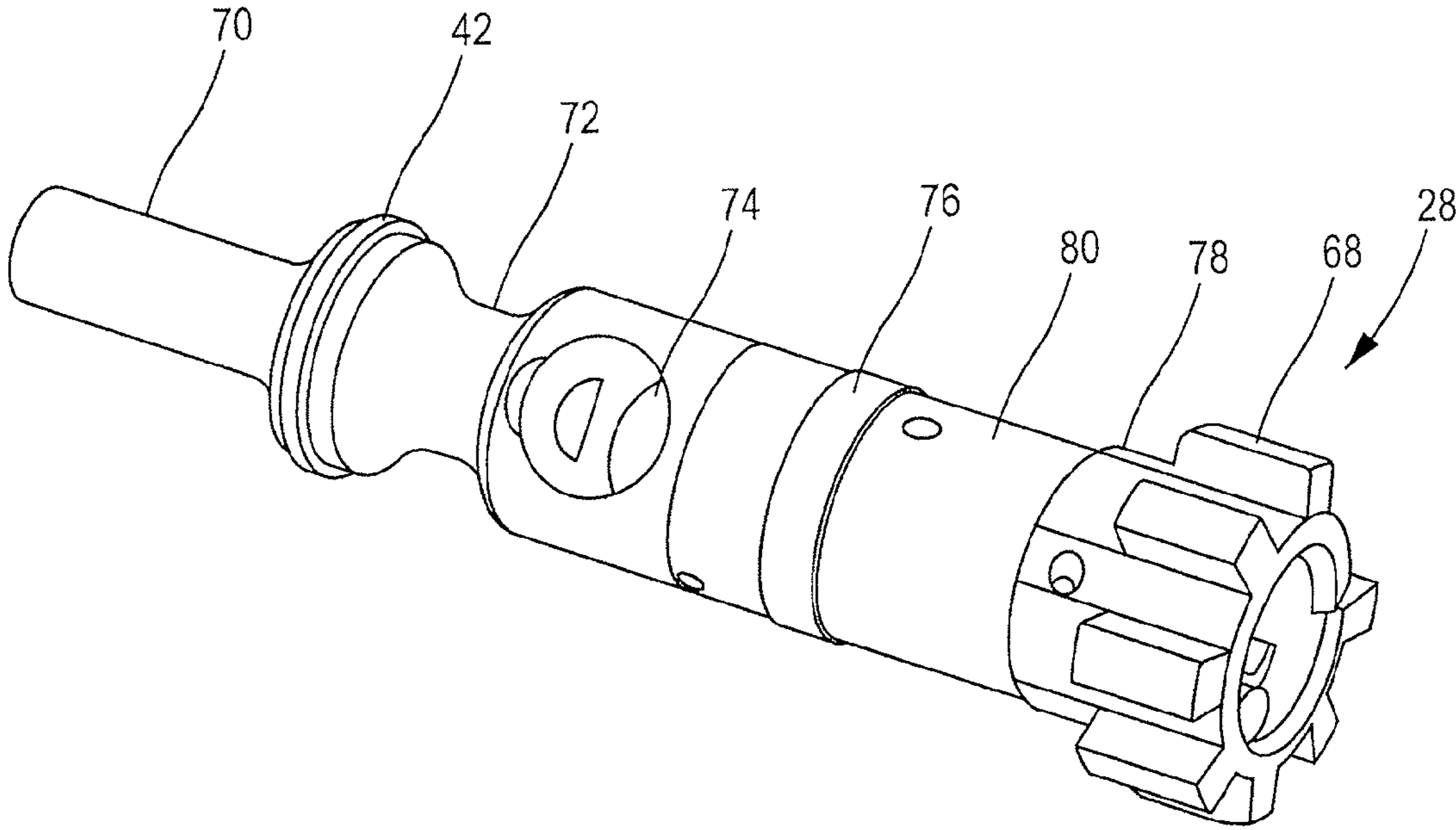
Fig.16 PRIOR ART
