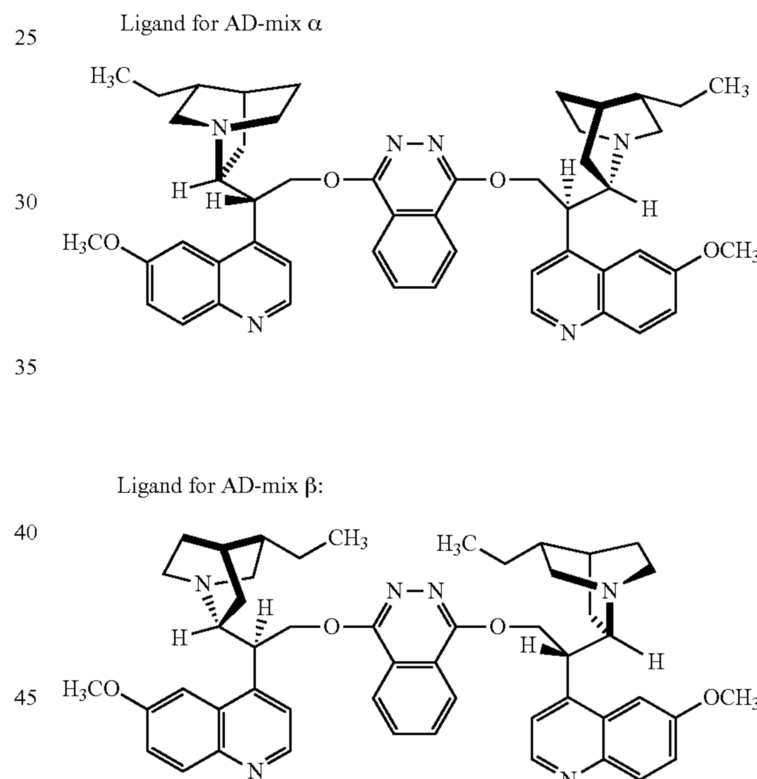
Scheme 5
