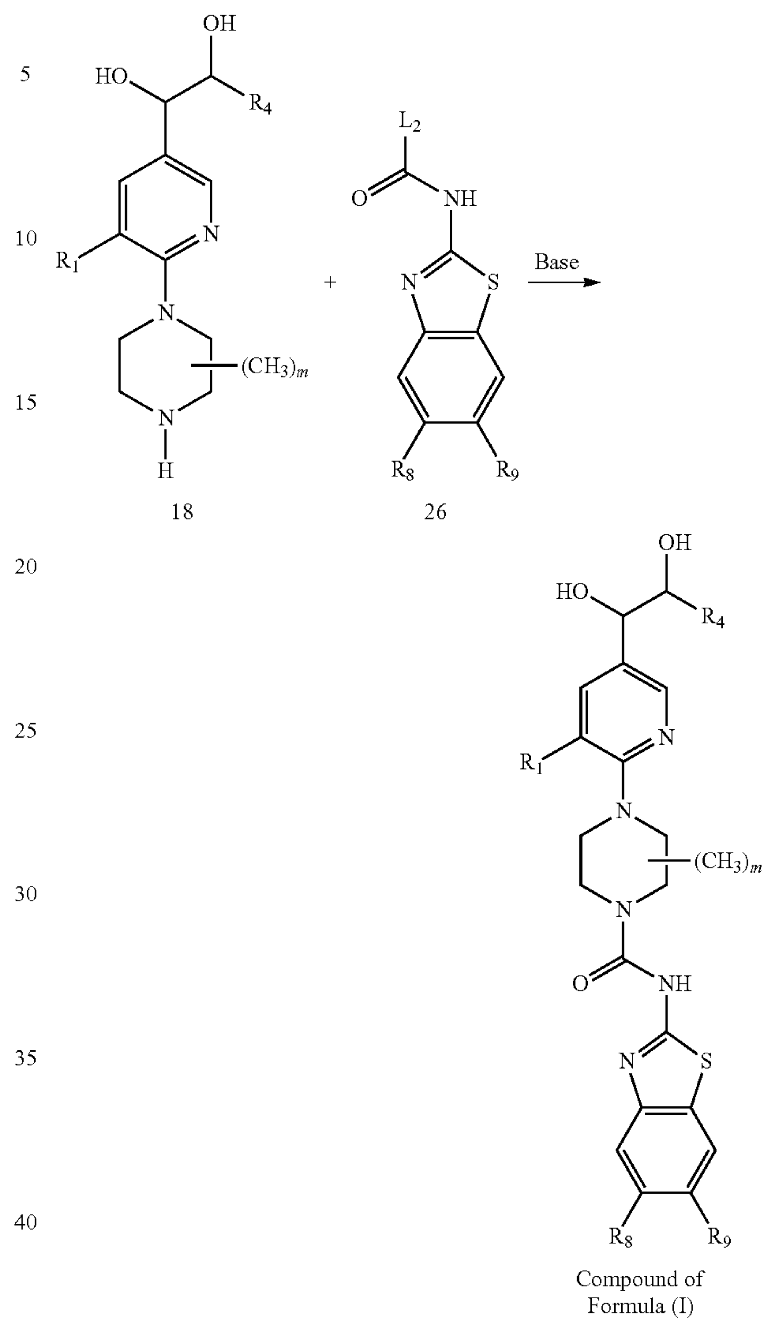
Scheme 16
