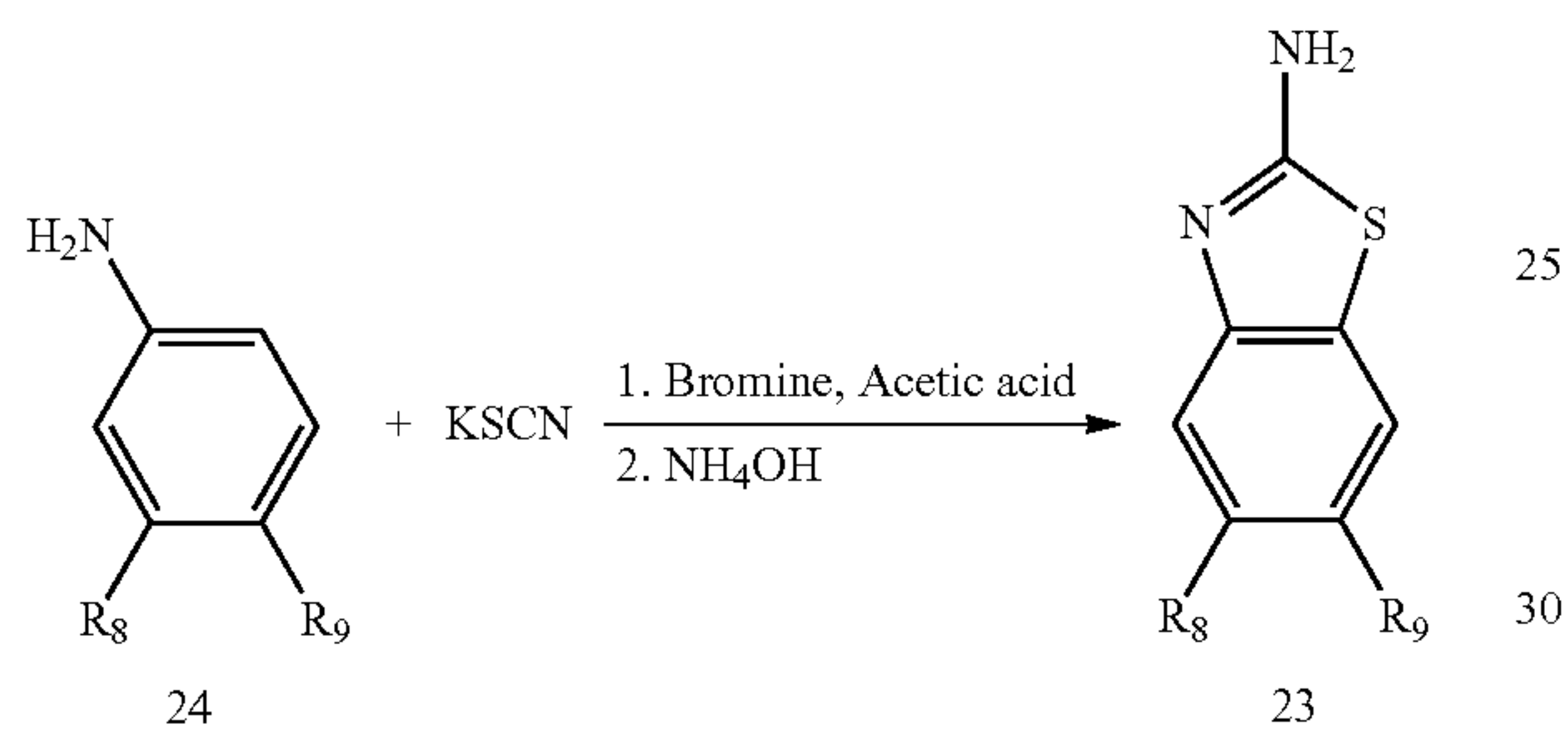
Scheme 14
