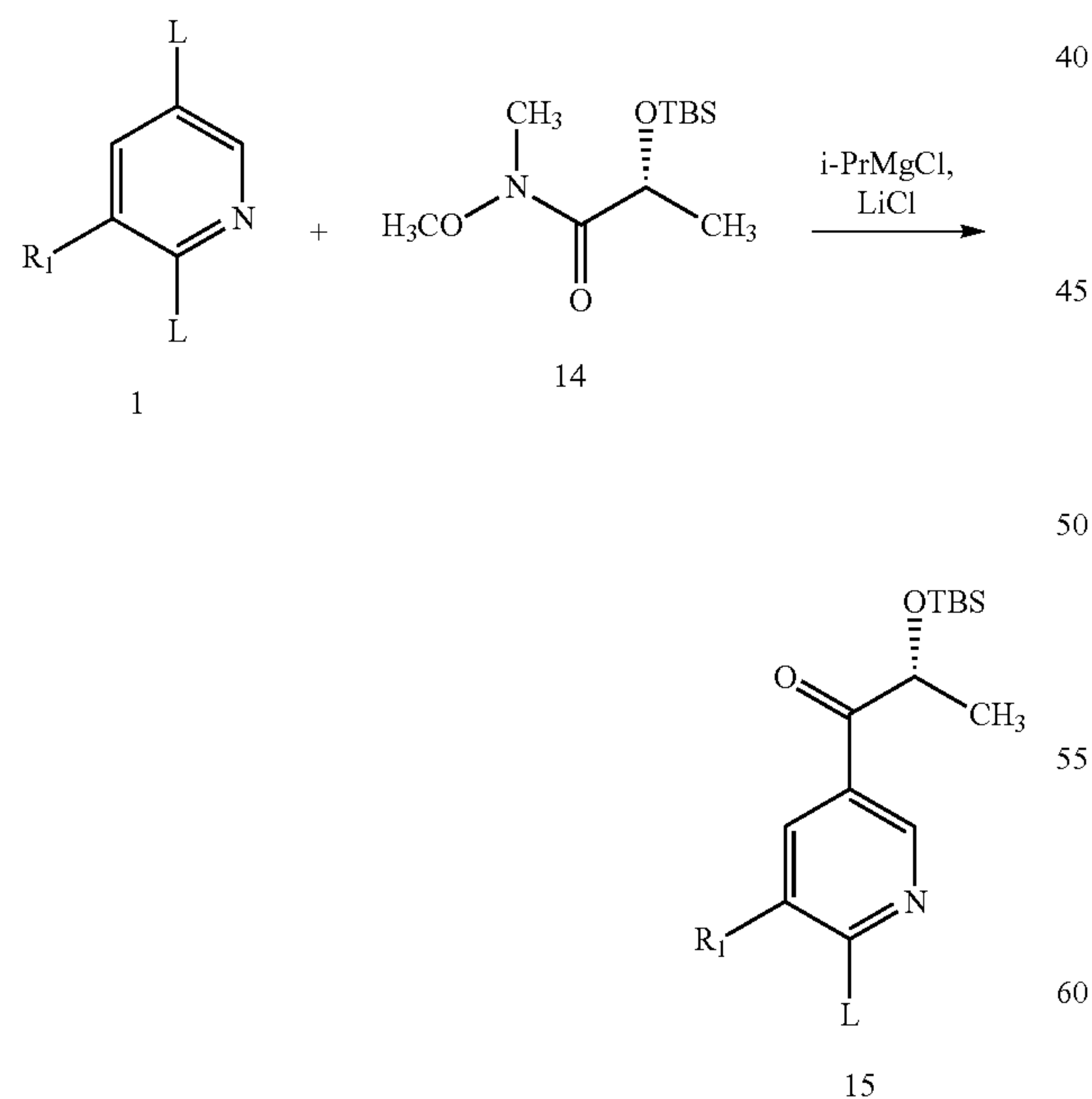
Scheme 7
