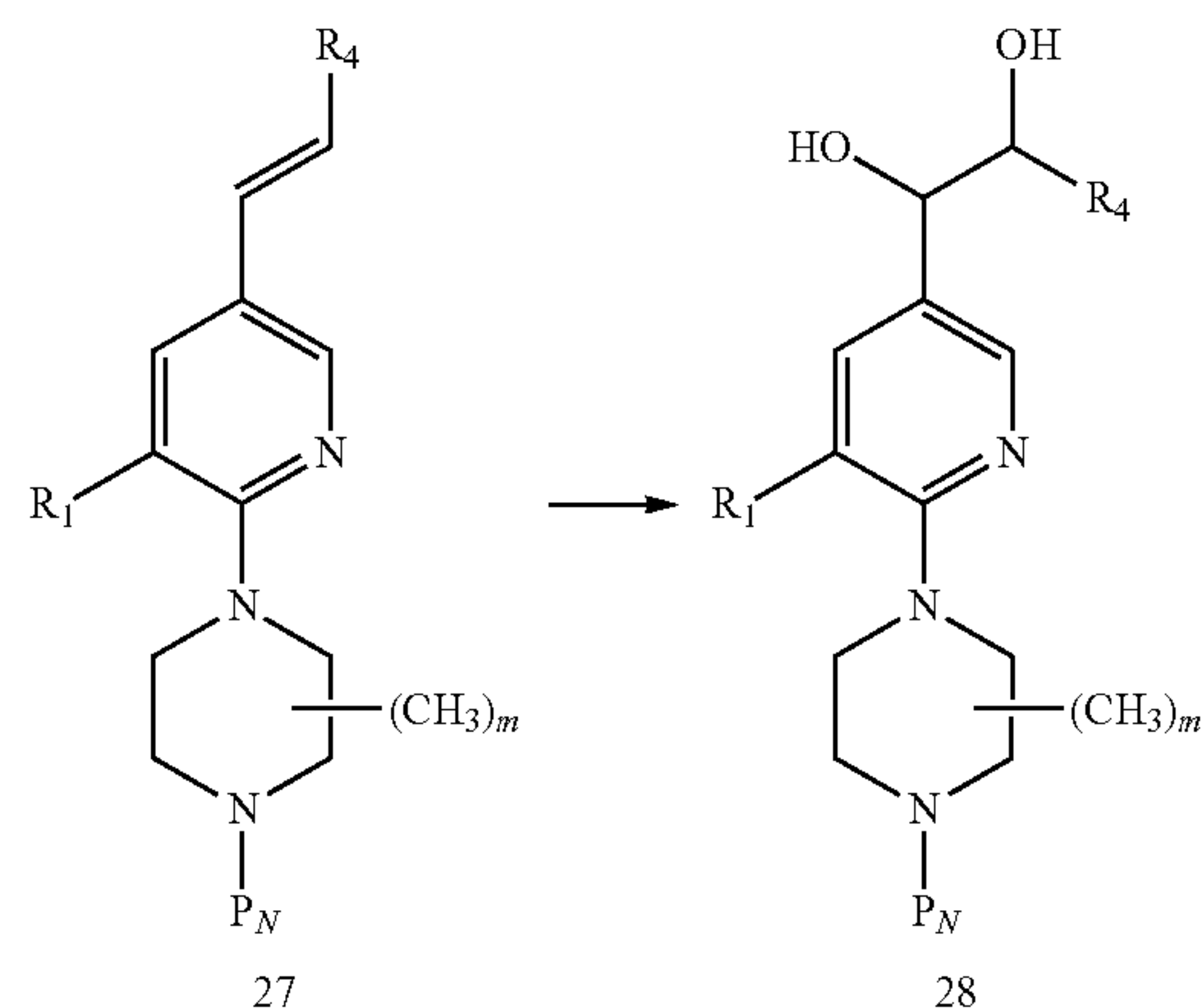
Scheme 19
