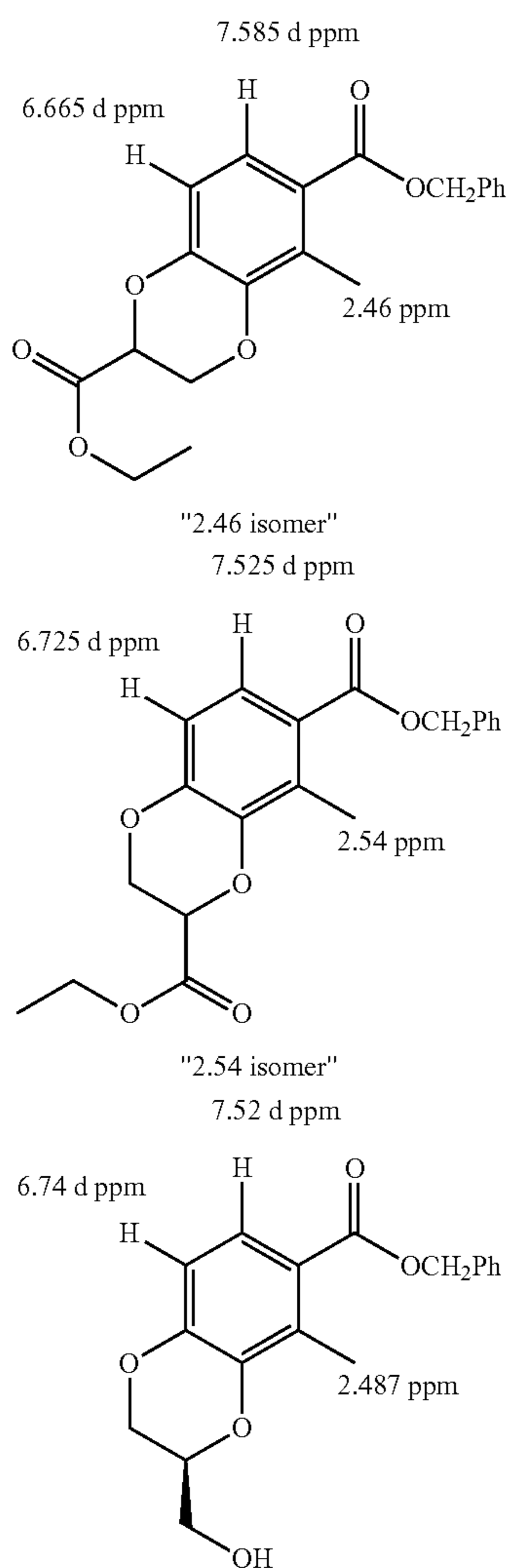
X-ray crystal structure of RG-119097 (naphthyl, ethylamide derivative) proves benzodioxan regioisomer
