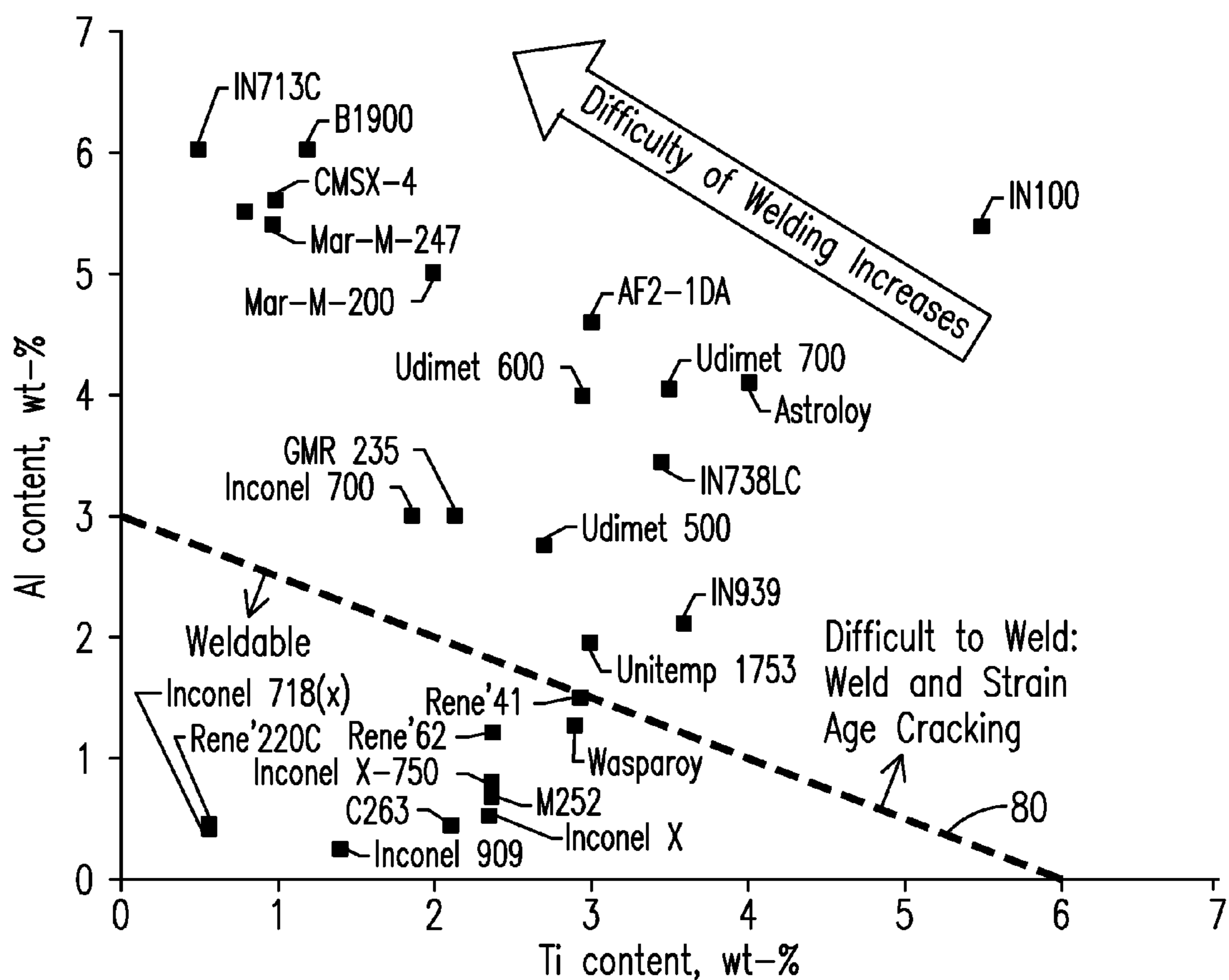
FIG. 6 PRIOR ART
