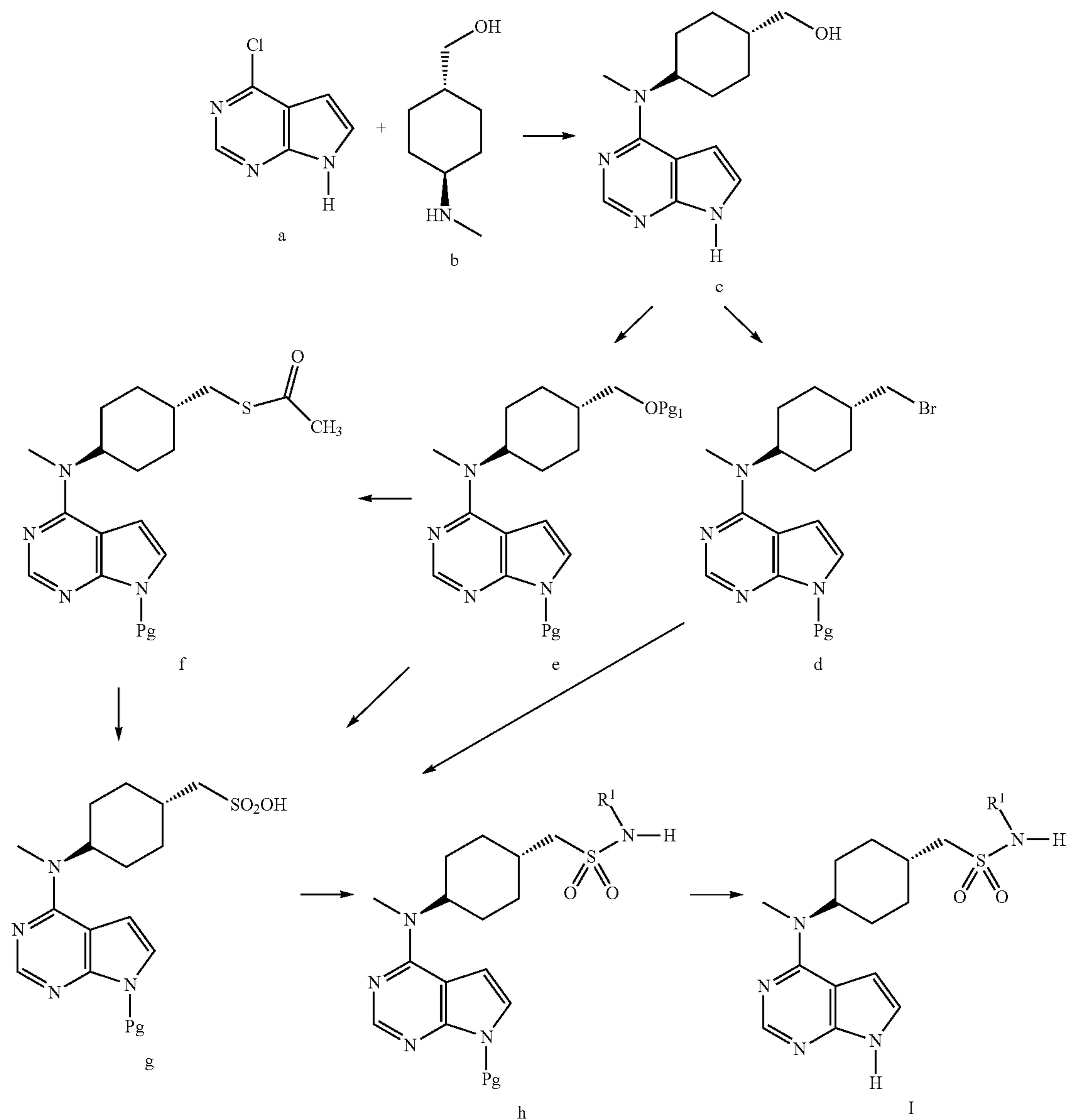
Scheme I
