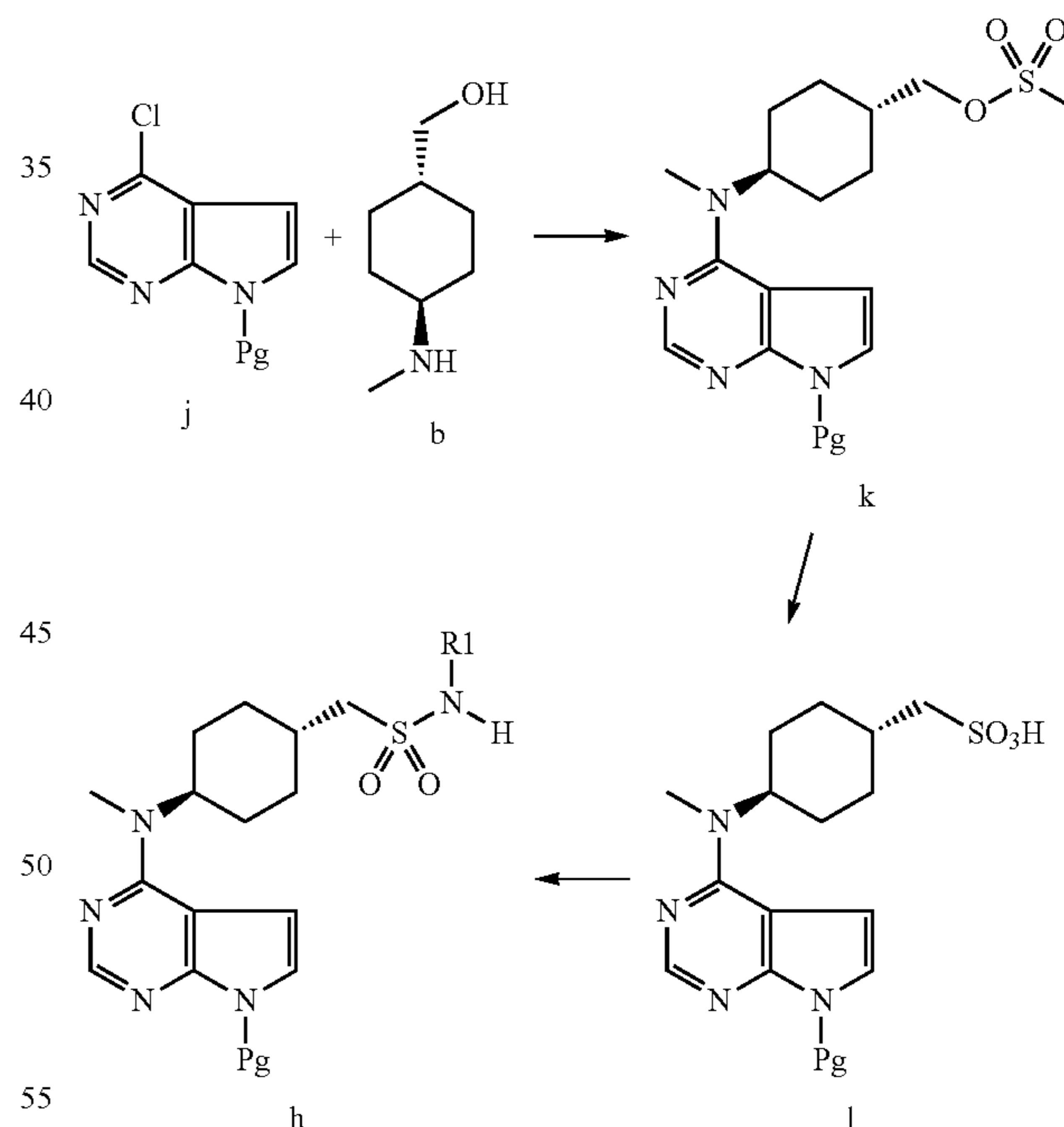
Scheme II
