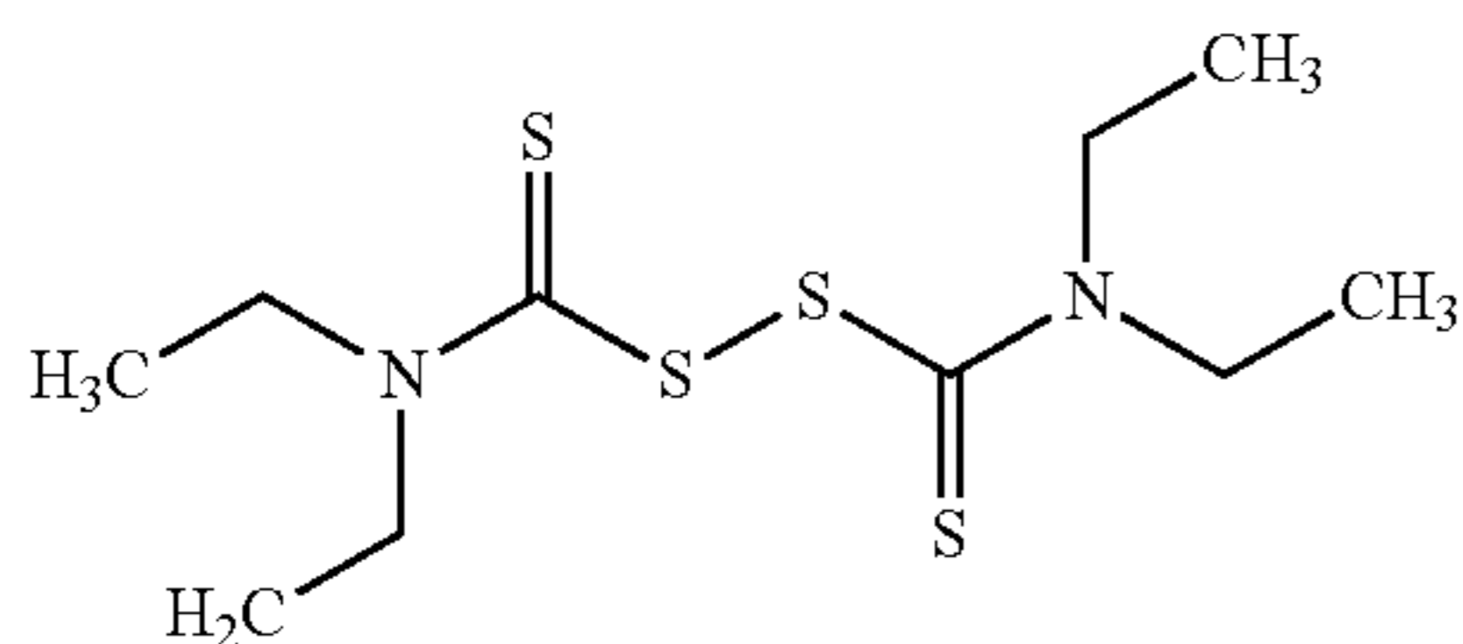
1,1',1'',1'''-[disulfanediy]bis(carbonothioylnitriloyl) tetraethane
