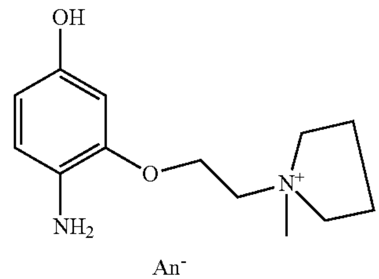
1-[2-(2-amino-5-hydroxyphenoxy)ethyl]-1-methylpyrrolidinium, An -
