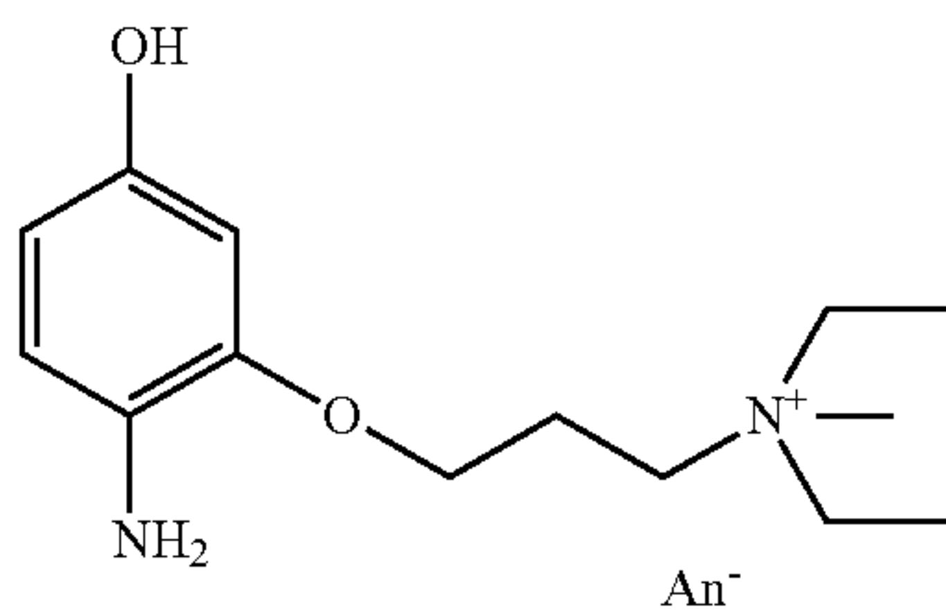
1-[3-(2-amino-5-hydroxyphenoxy)propyl]-1-methylpyrrolidinium, An -
