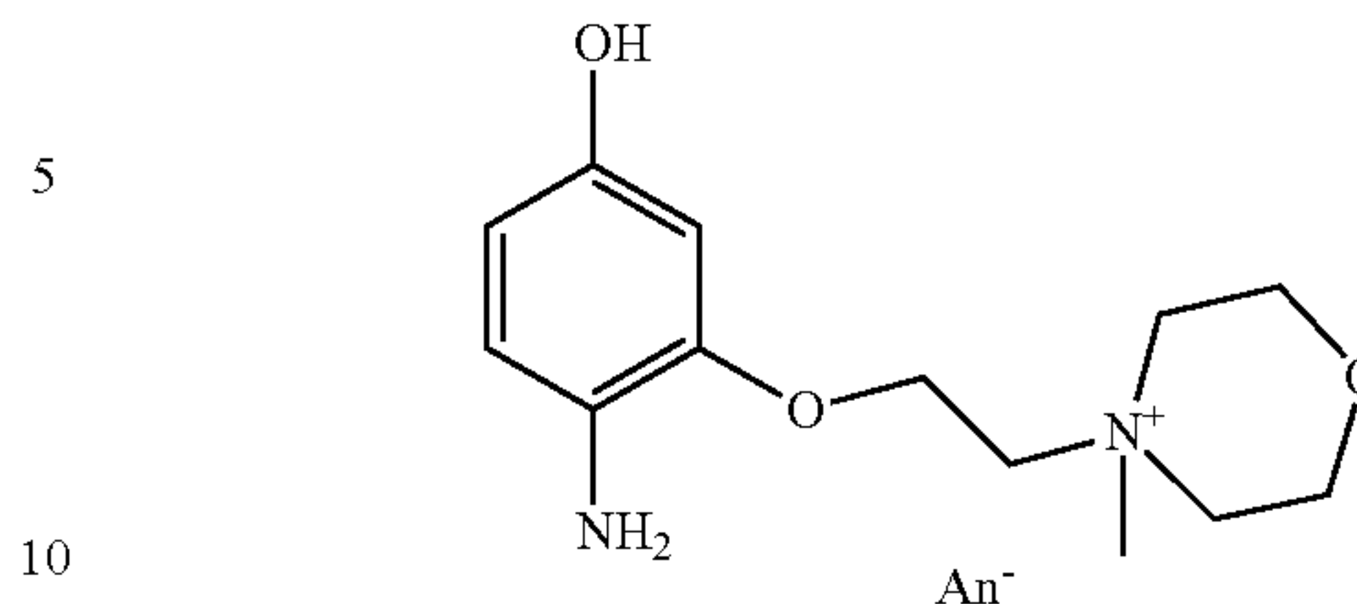
4-[2-(2-amino-5-hydroxyphenoxy)ethyl]-4-methylmorpholin-4-ium, An -
