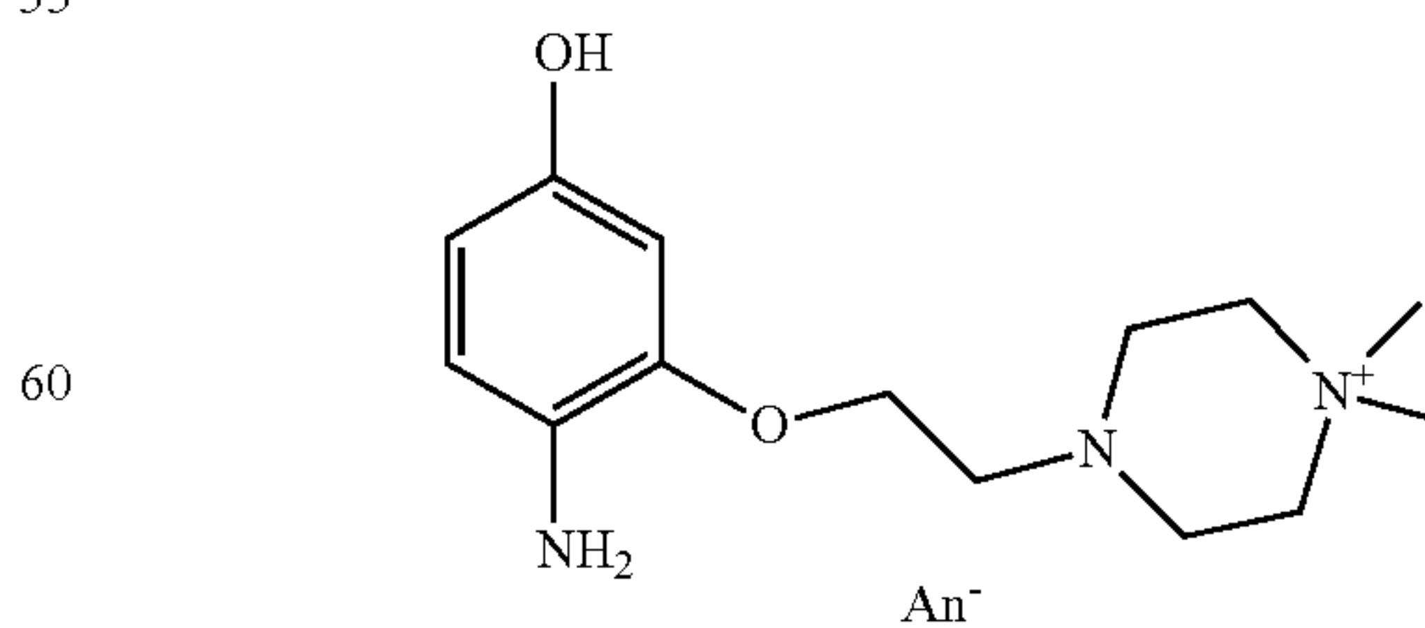
4-[2-(2-amino-5-hydroxyphenoxy)ethyl]-1,1-dimethylpiperazin-1-ium, An -
