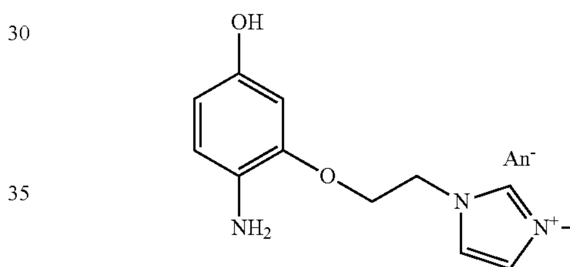
1-[2-(2-amino-5-hydroxyphenoxy)ethyl]-3-methyl-1H-imidazol-3-ium, An -
