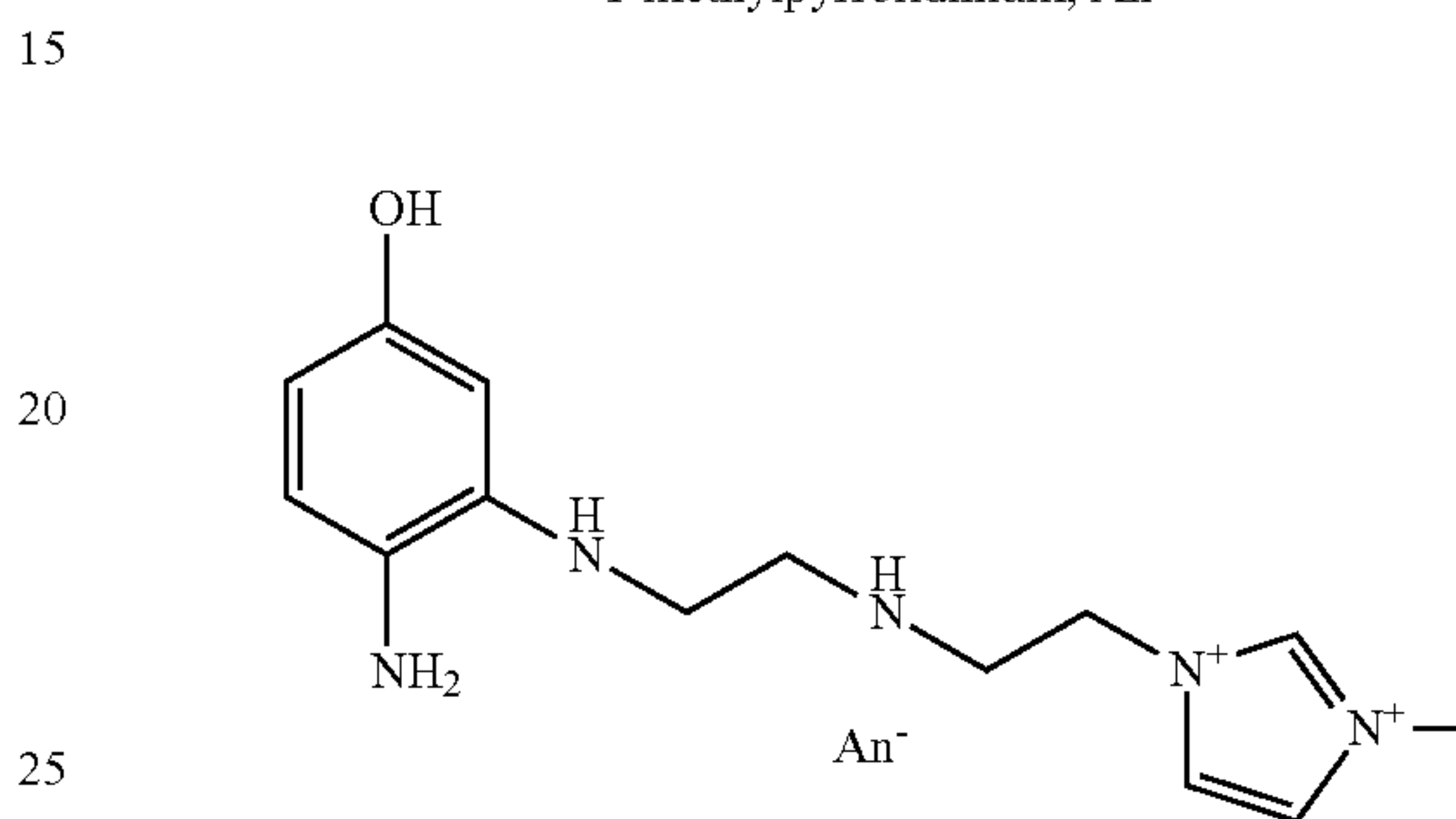
1-[2-({2-[(2-amino-5-hydroxyphenyl)amino]ethyl}amino)ethyl]-1-methylpyrrolidinium, An -
