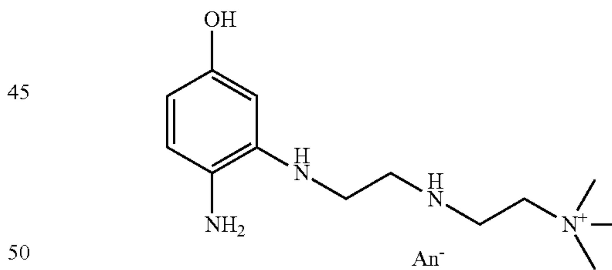
2-({2-[(2-amino-5-hydroxyphenyl)amino]ethyl}amino)-N,N,N-trimethylethanaminium, An -
