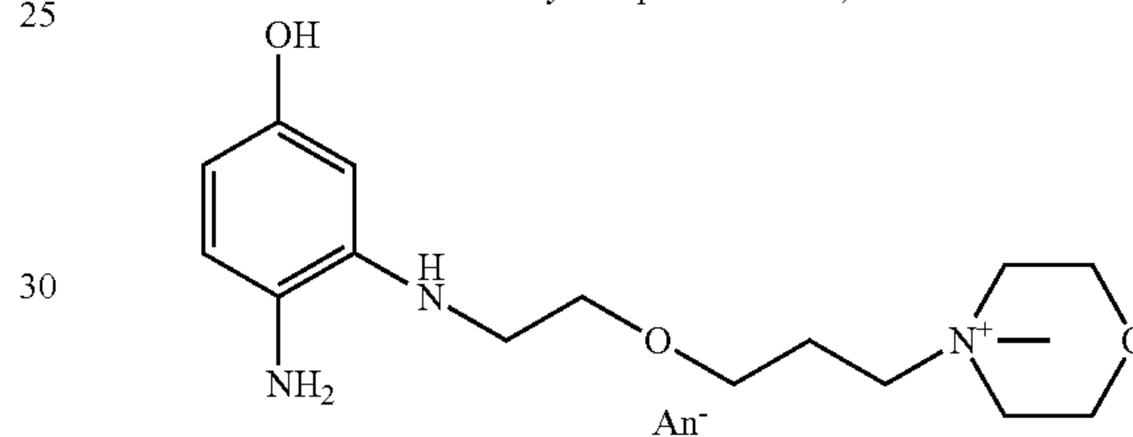
4-(2{2-[(2-amino-5-hydroxyphenyl)amino]ethoxy}ethyl)-4-methylmorpholin-4-ium, An -
