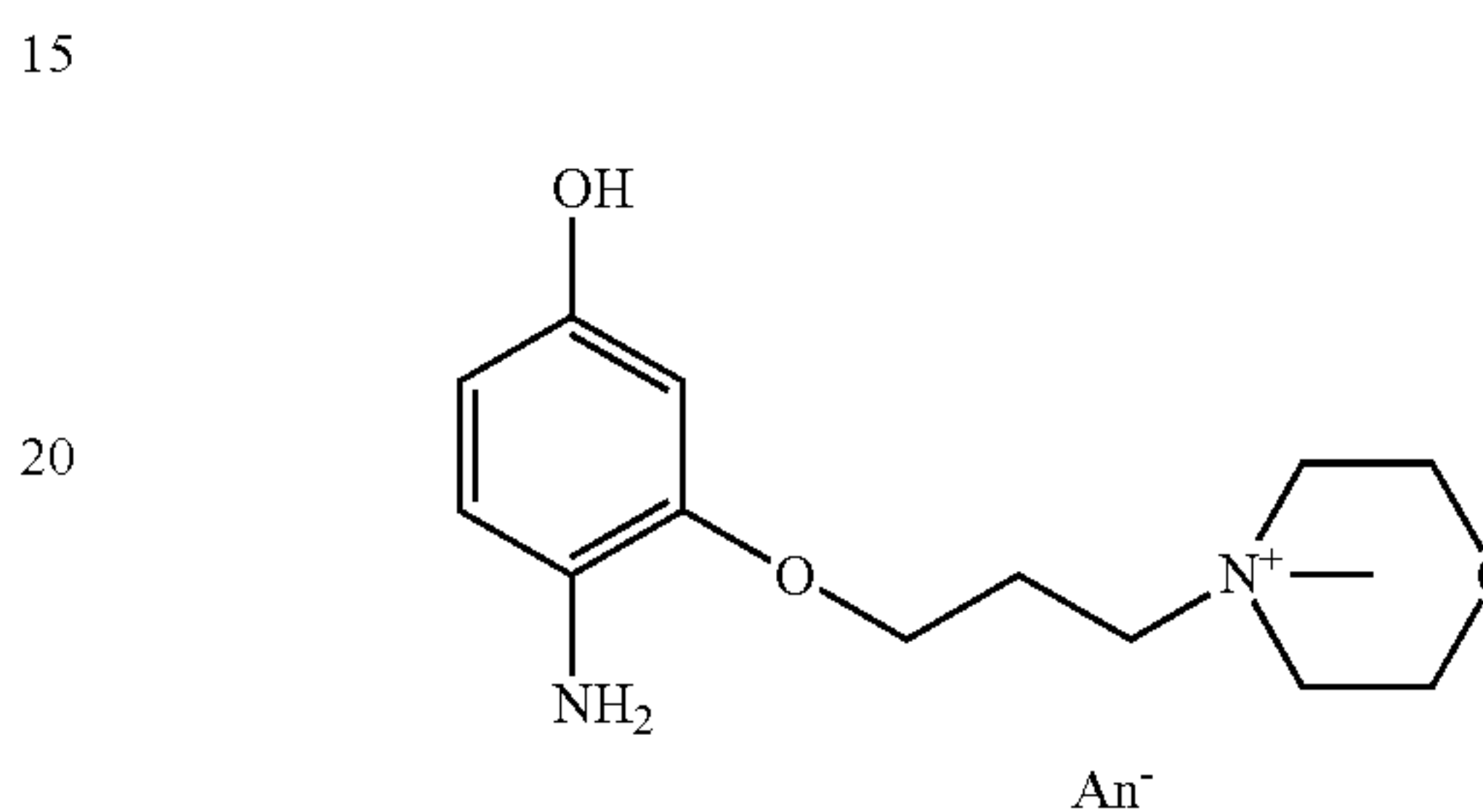
4-[3-(2-amino-5-hydroxyphenoxy)propyl]-4-methylmorpholin-4-ium, An -
