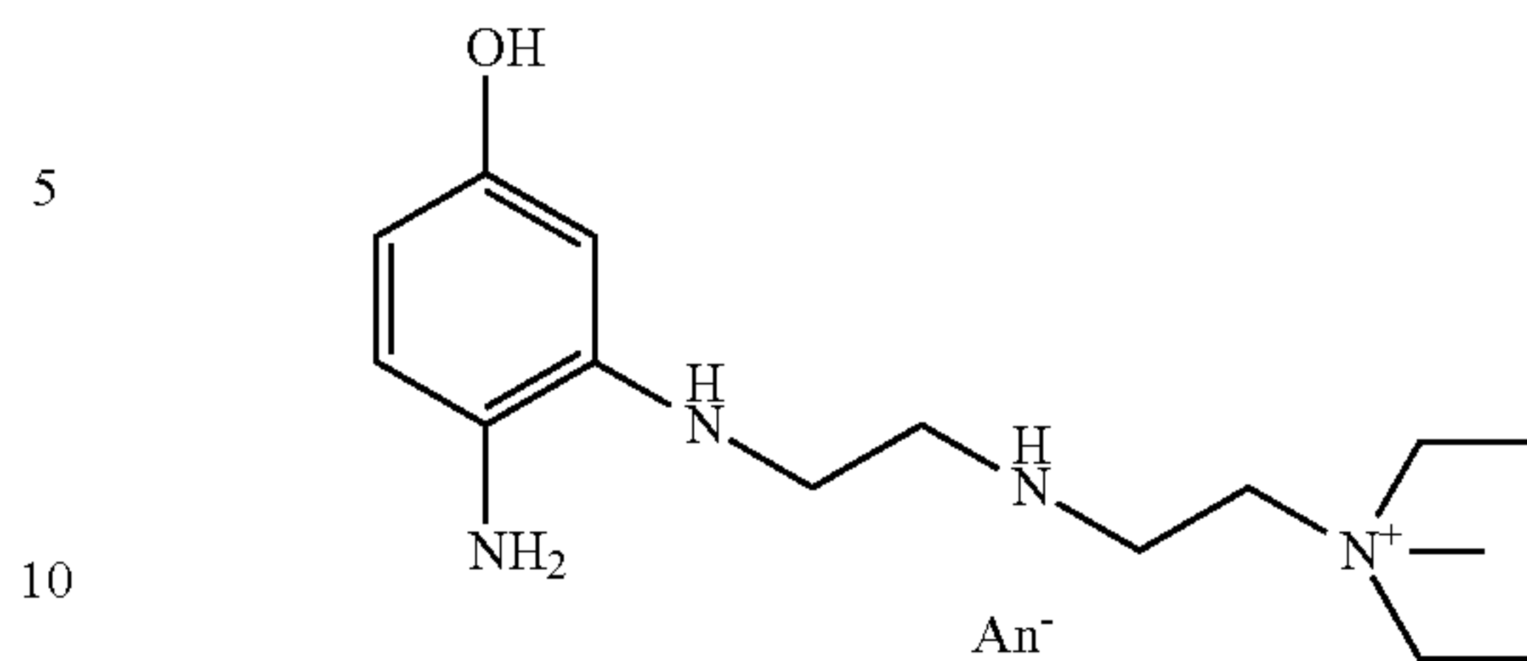
1-[2-({2-[(2-amino-5-hydroxyphenyl)amino]ethyl}amino)ethyl]-1-methylpyrrolidinium, An -
