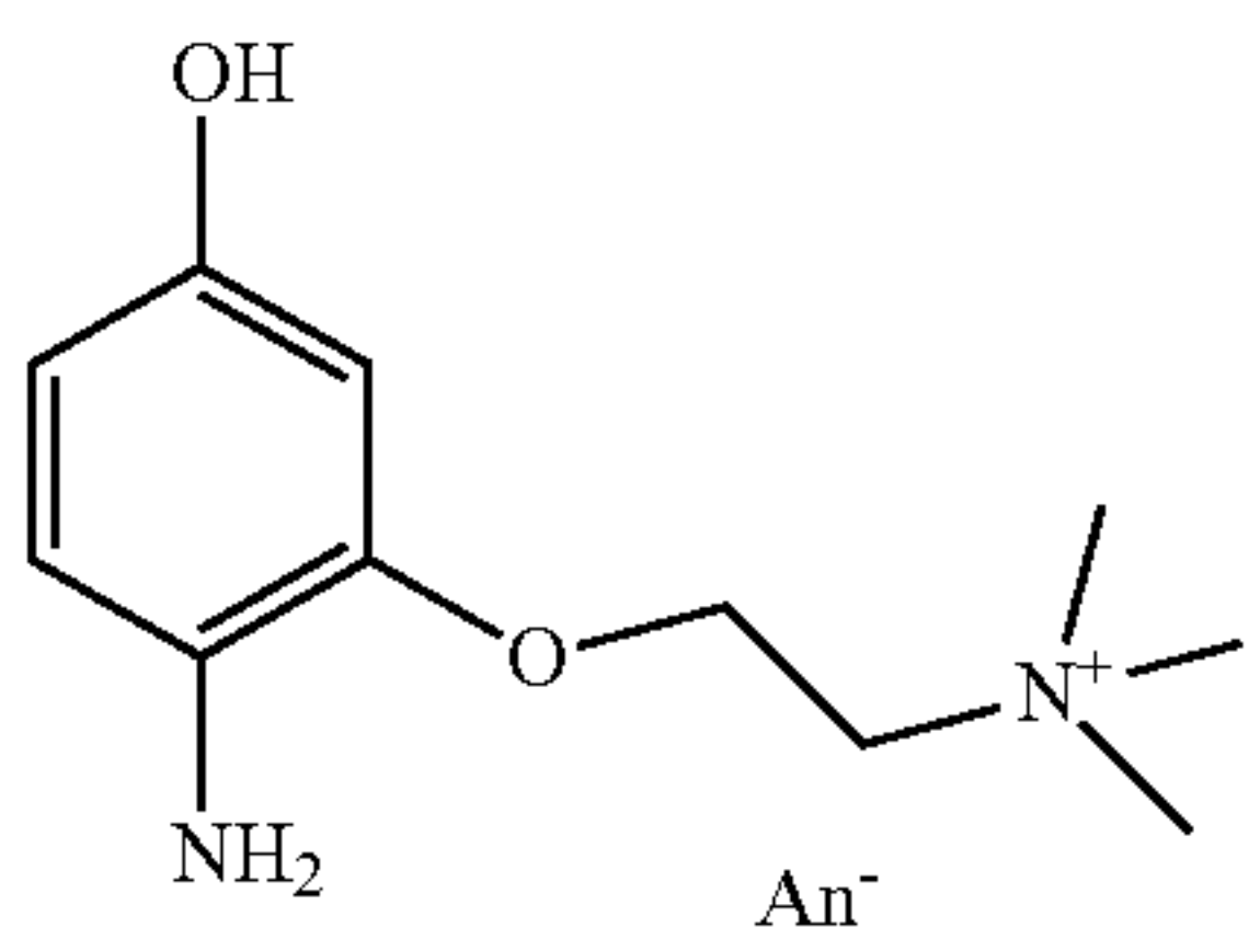
2-(2-amino-5-hydroxyphenoxy)-N,N,N-trimethylethanaminium, An -
