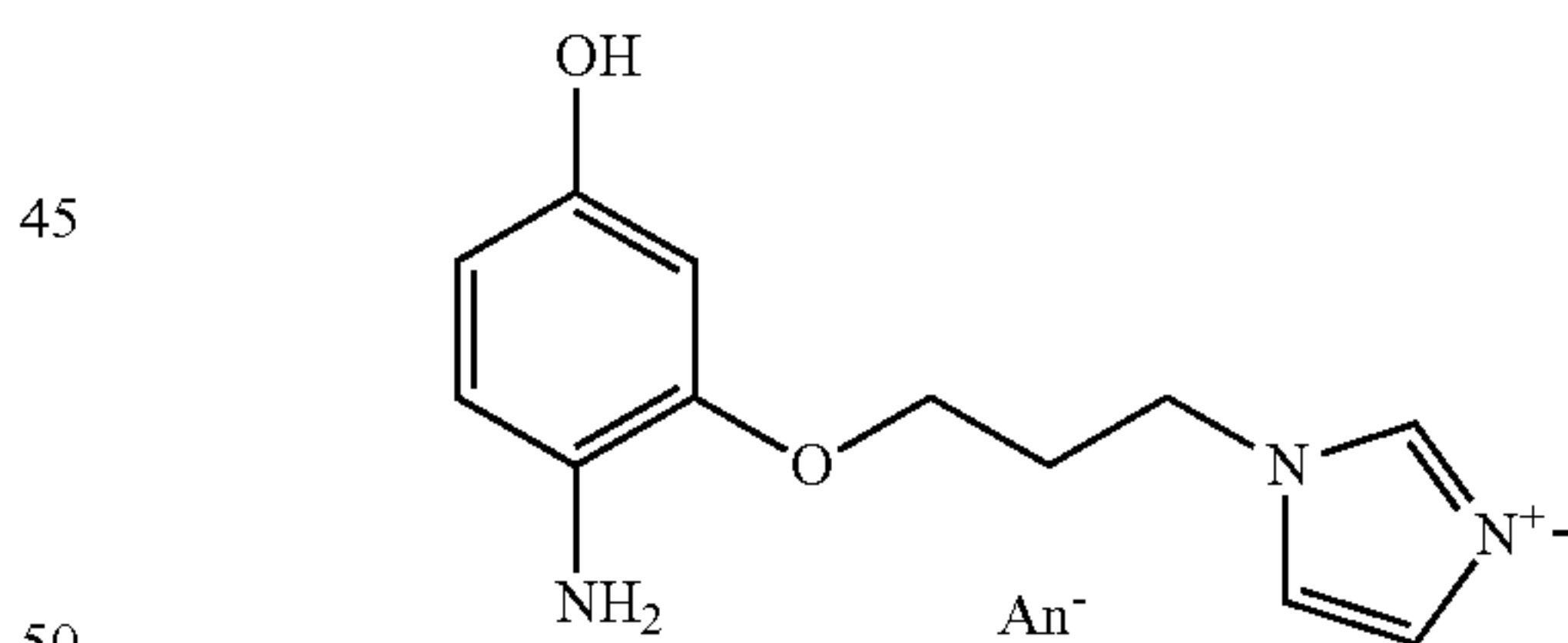
1-[3-(2-amino-5-hydroxyphenoxy)propyl]-3-methyl-1H-imidazol-3-ium, An -
