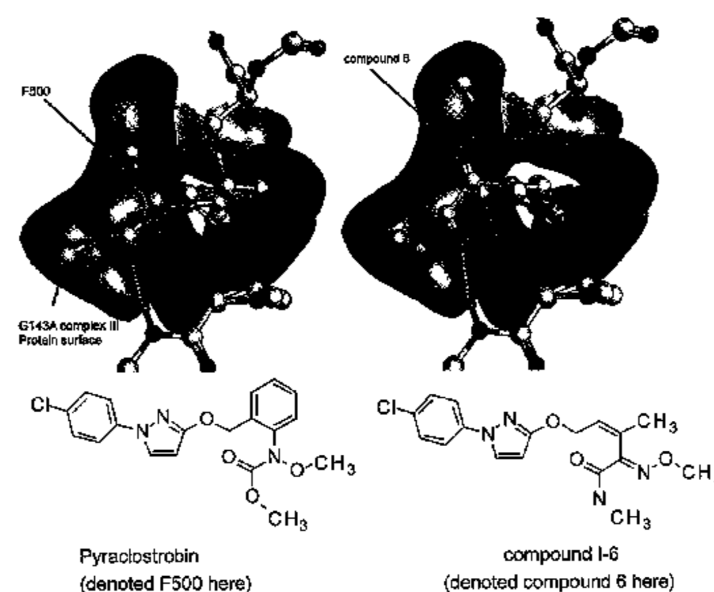
Structural Models of G143A mutant binding site
