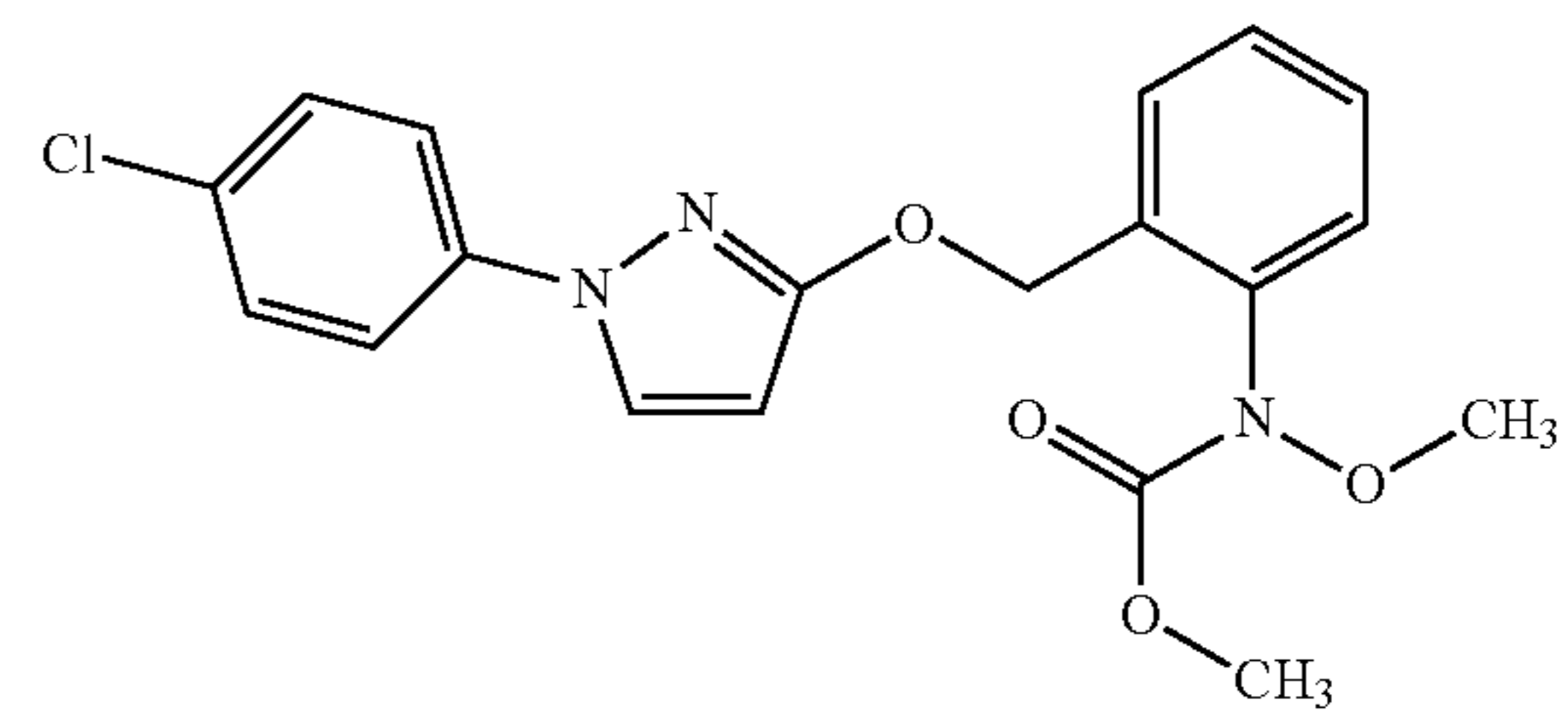
Pyraclostrobin
