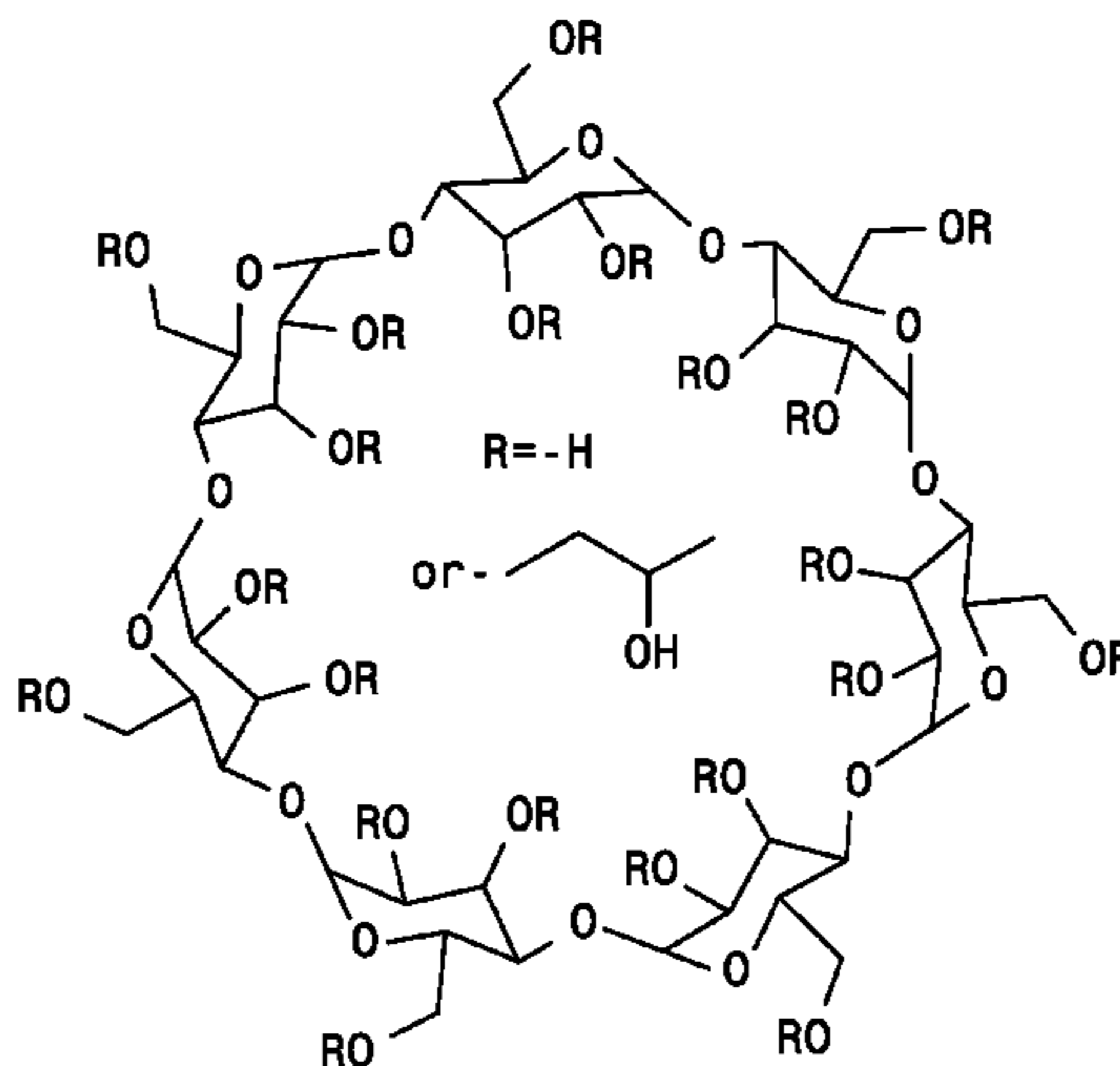
β-CYCLODEXTRIN AND ITS HYDROXYPROPYL DERIVATIVE
