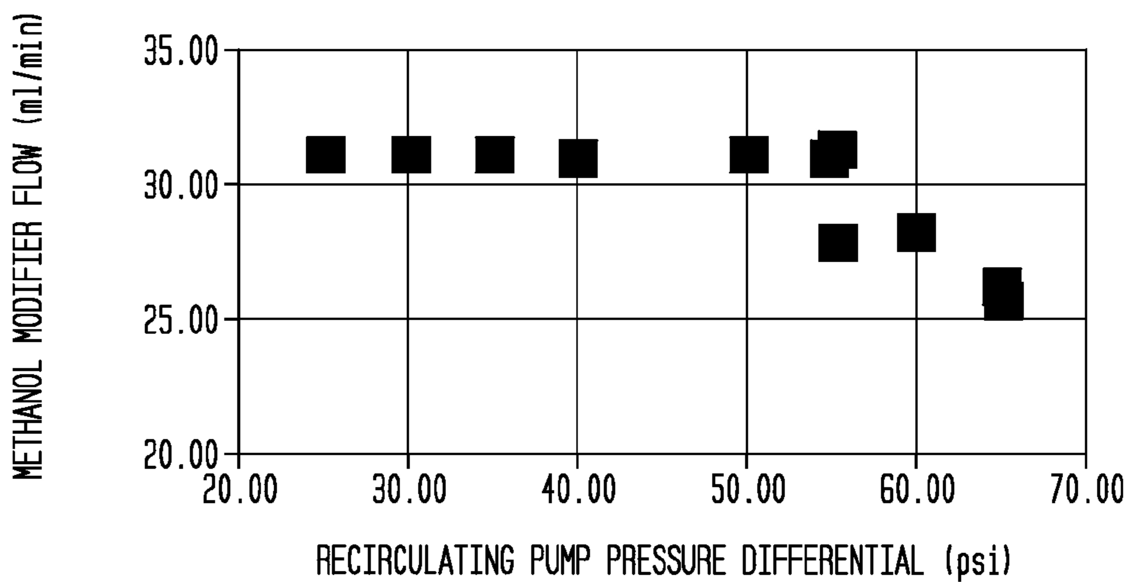
FIG. 6 METHANOL FEED AS A FUNCTION OF DELTA P (CIRCULATION RATE); HIGHLY REACTIVE PIB; NOMINAL M_n of 1000
