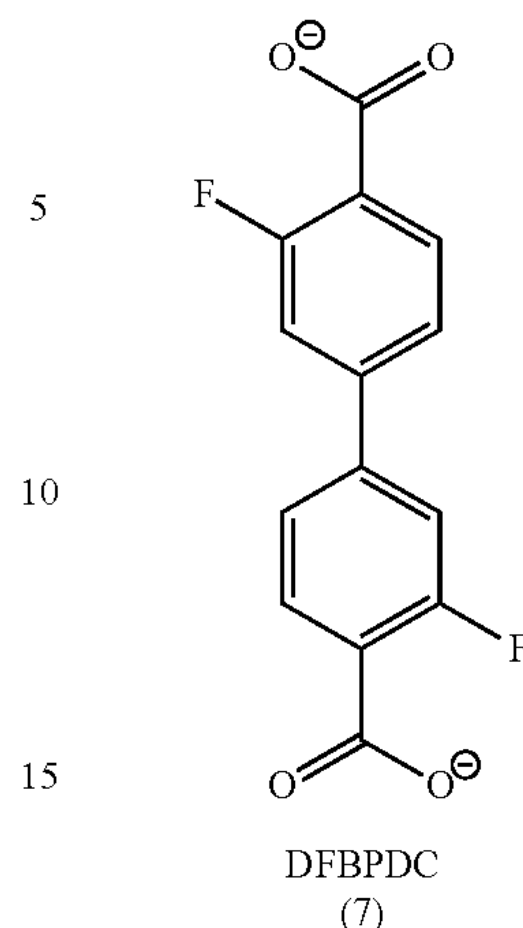
Scheme 1. Representation of the organic linkers present in compounds 1-7.
