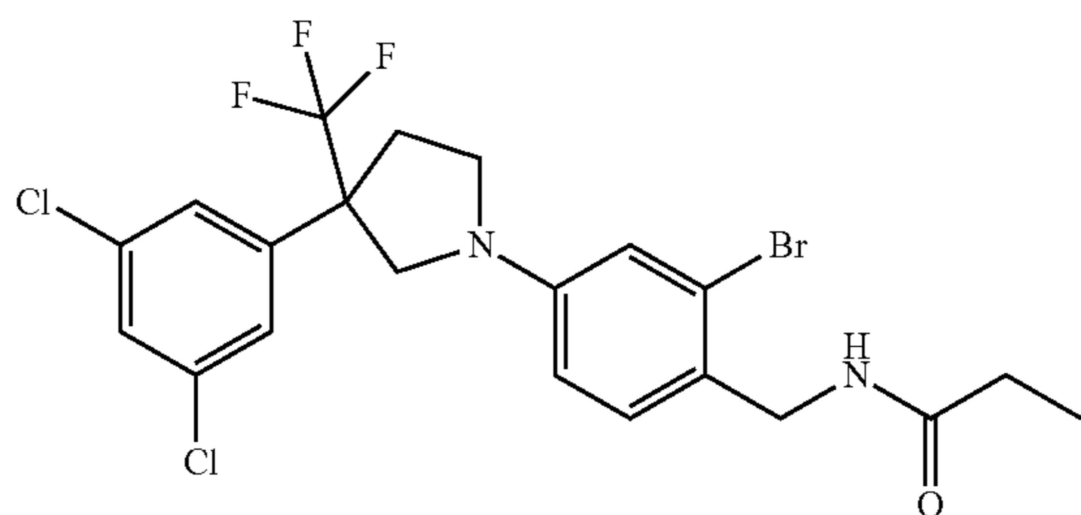
Compound No. 3-5 according to WO2008/12871
