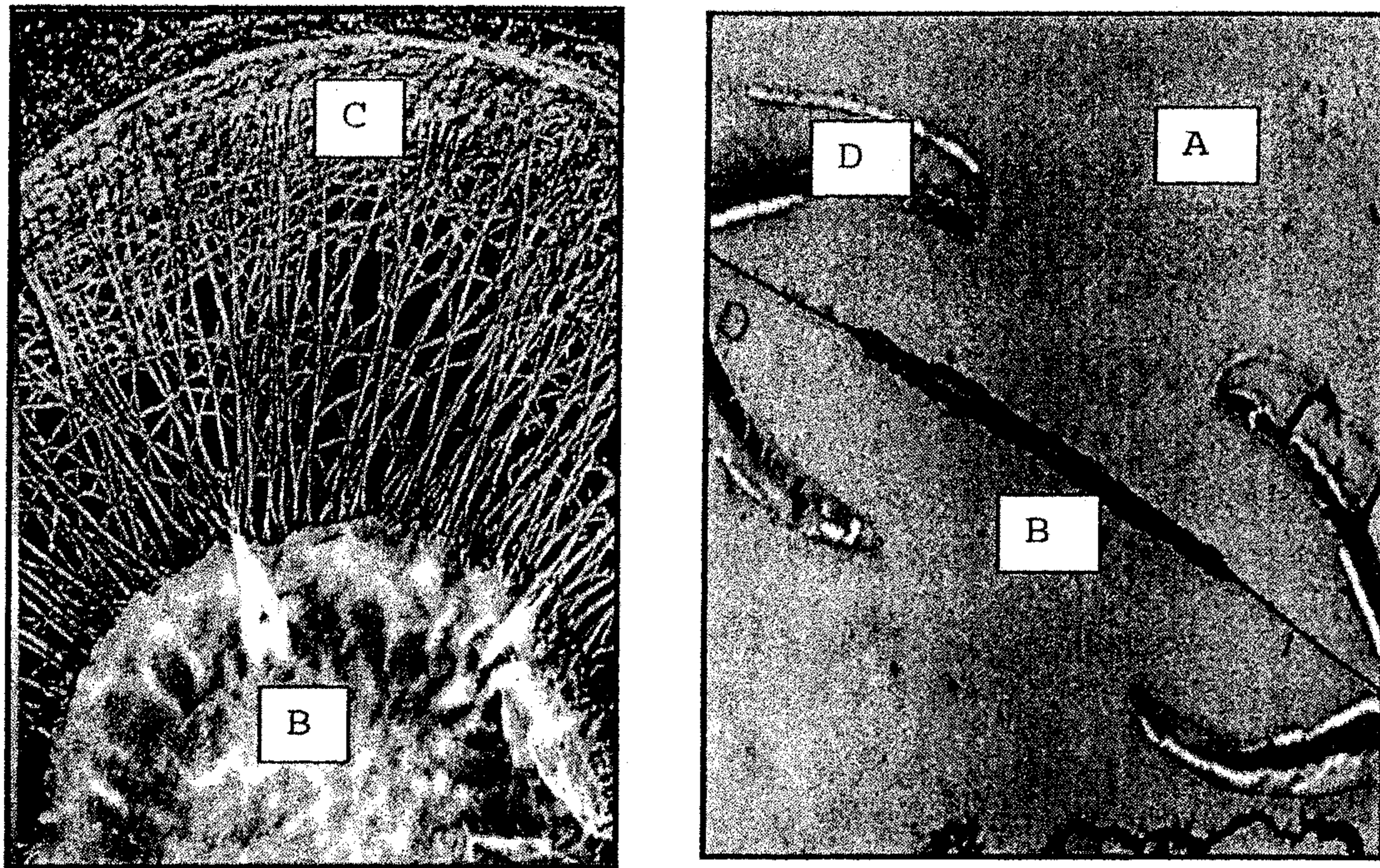
Bordered Pit
