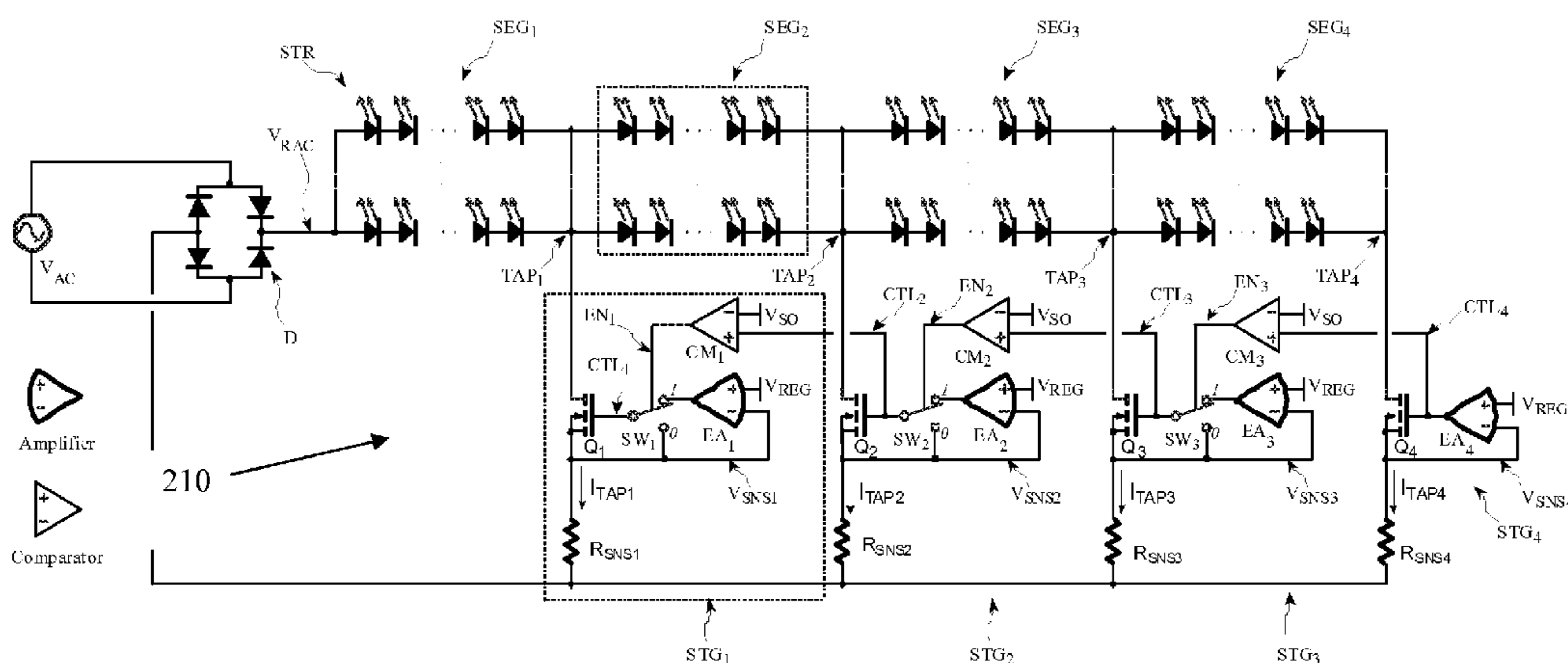
Self-Commutating Circuit
