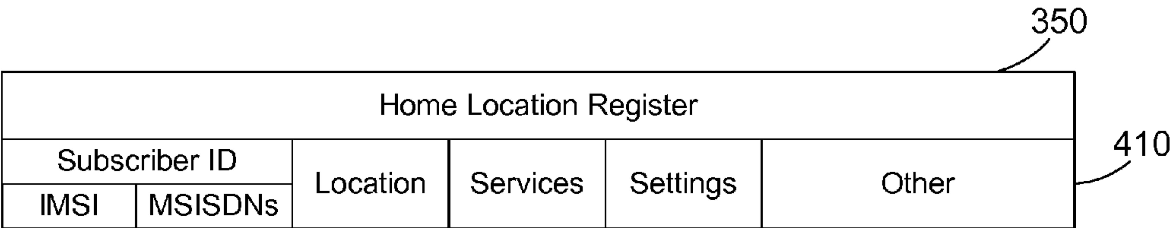
FIG. 3 Prior Art
