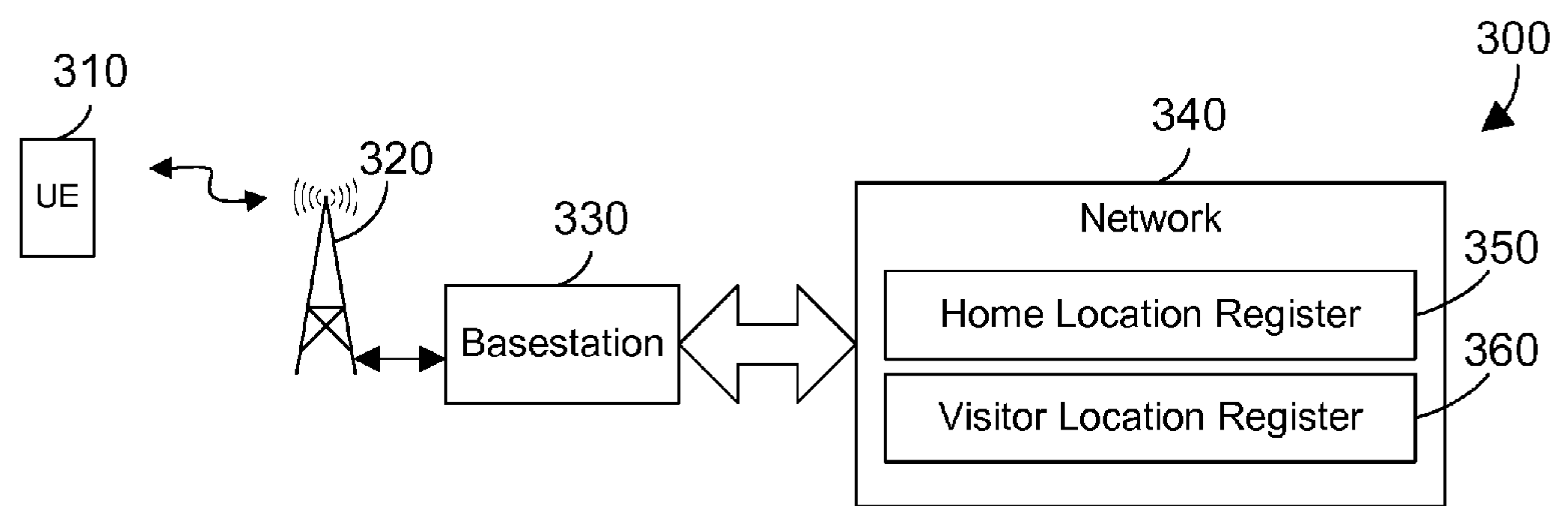
FIG. 3 Prior Art
