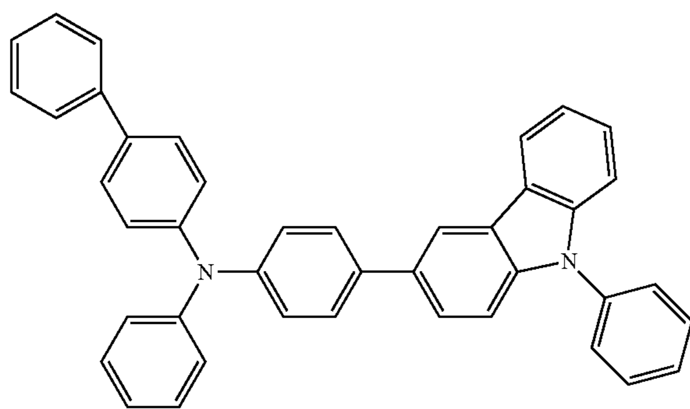
PCBA1BP
