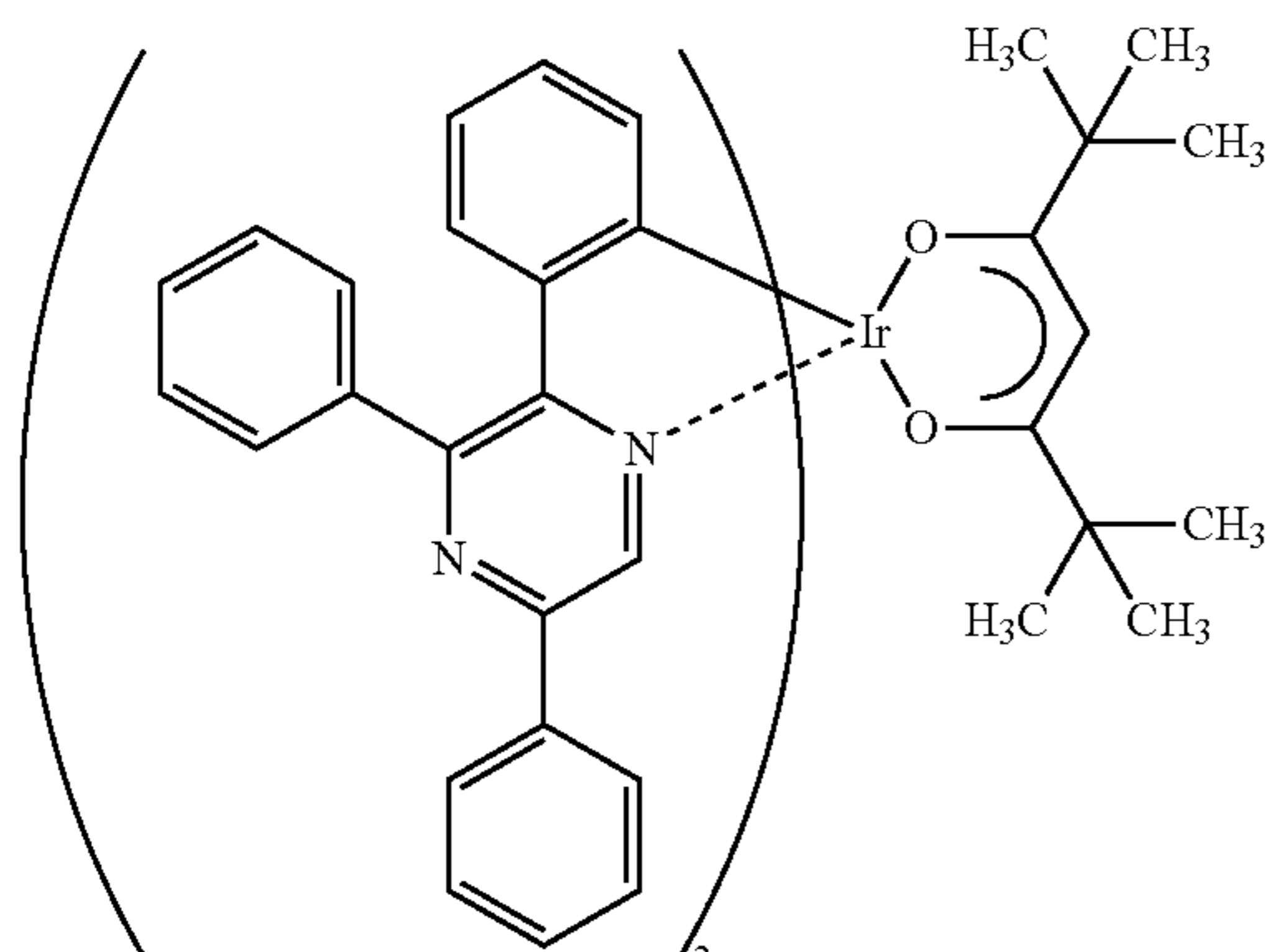
Ir(tppr) 2 (dpm)
