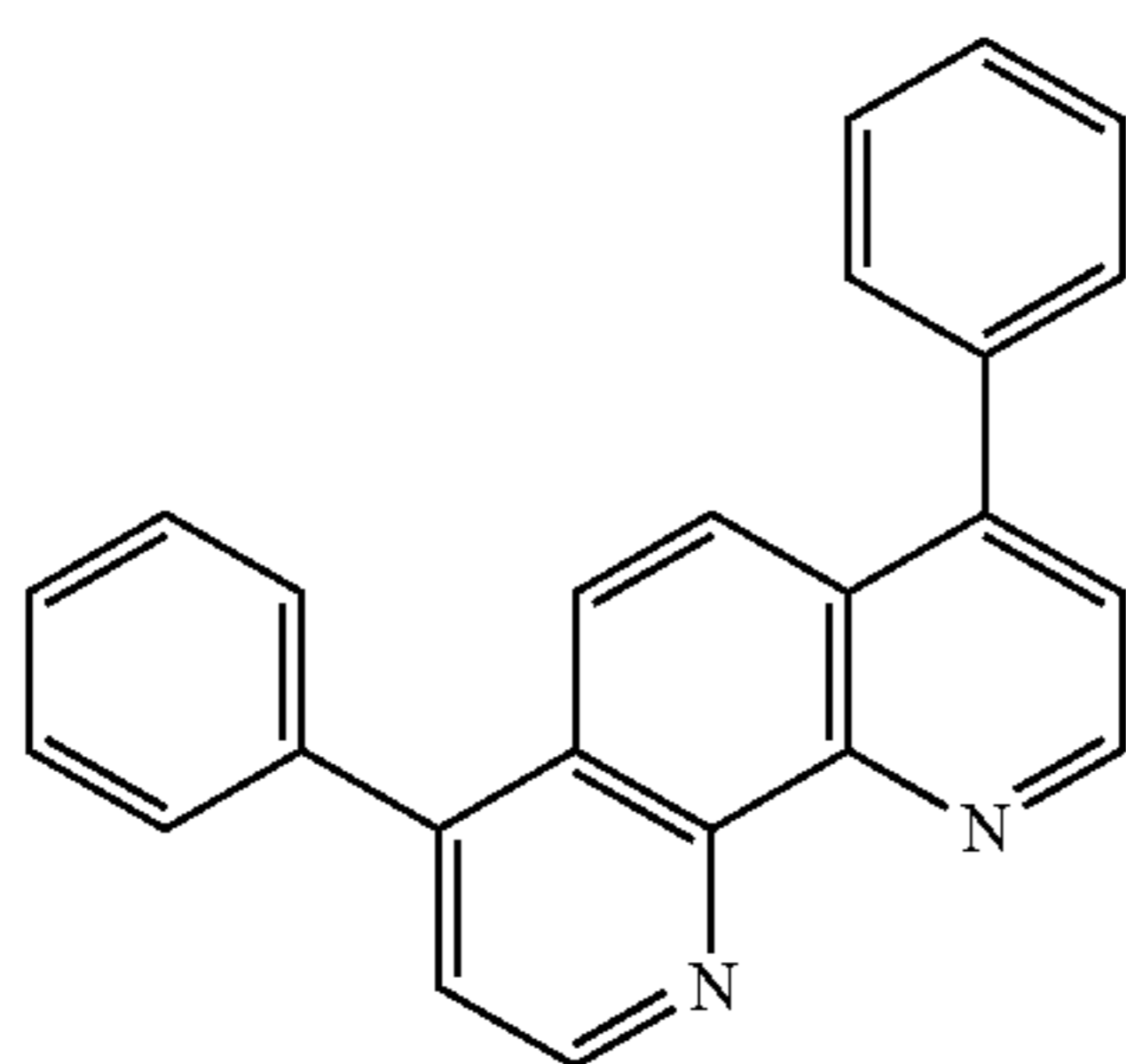
BPhen
