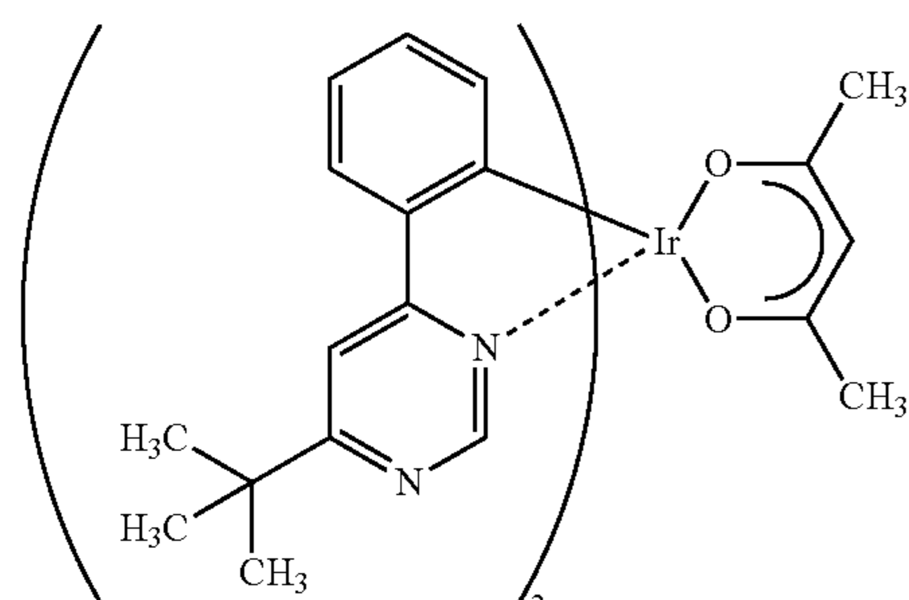
Ir(tBuppm) 2 (acac)
